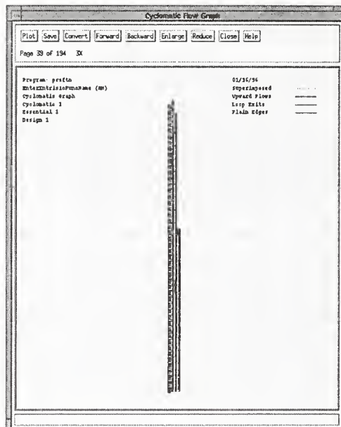
Figure 3-1. Control flow graph with complexity 1.
