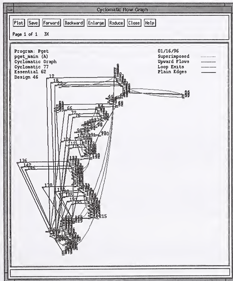
Figure 4-9. Module with complexity 77.
