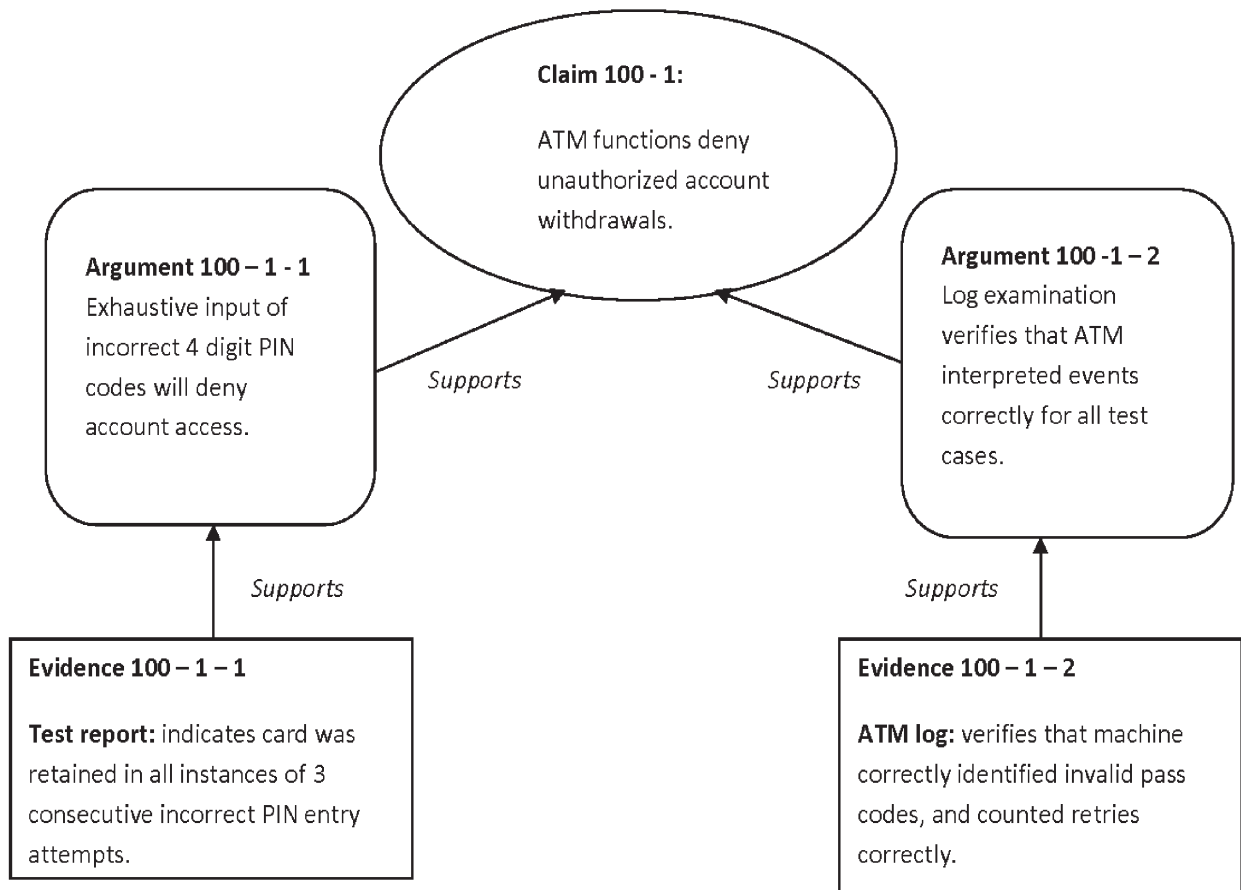
Fig. 2. Assurance Case Model for ATM.
