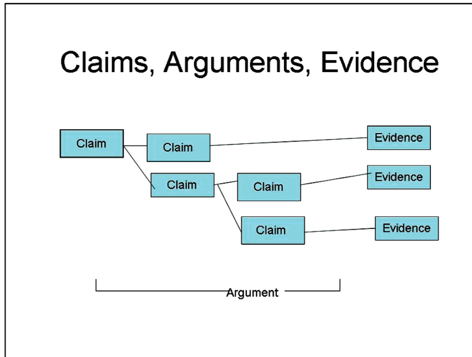
Fig. 1. Representation of a Structured Assurance Case Model.
