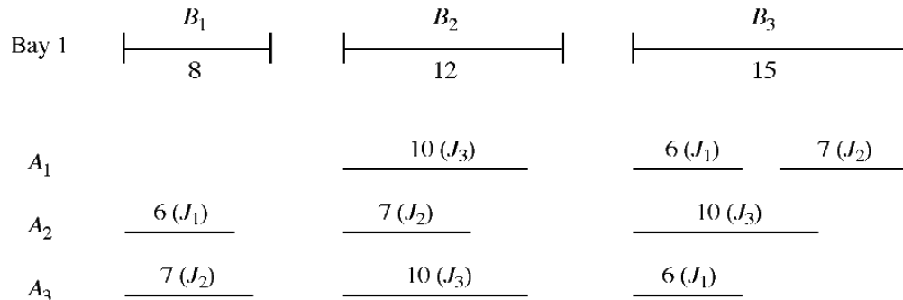
Fig. 1. Assignments A_1 , A_2 , A_3 .
