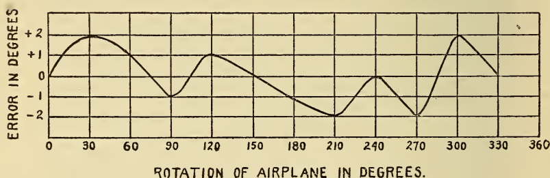
FIGURE 9.—Calibration graph for errors introduced by airplane structure.
