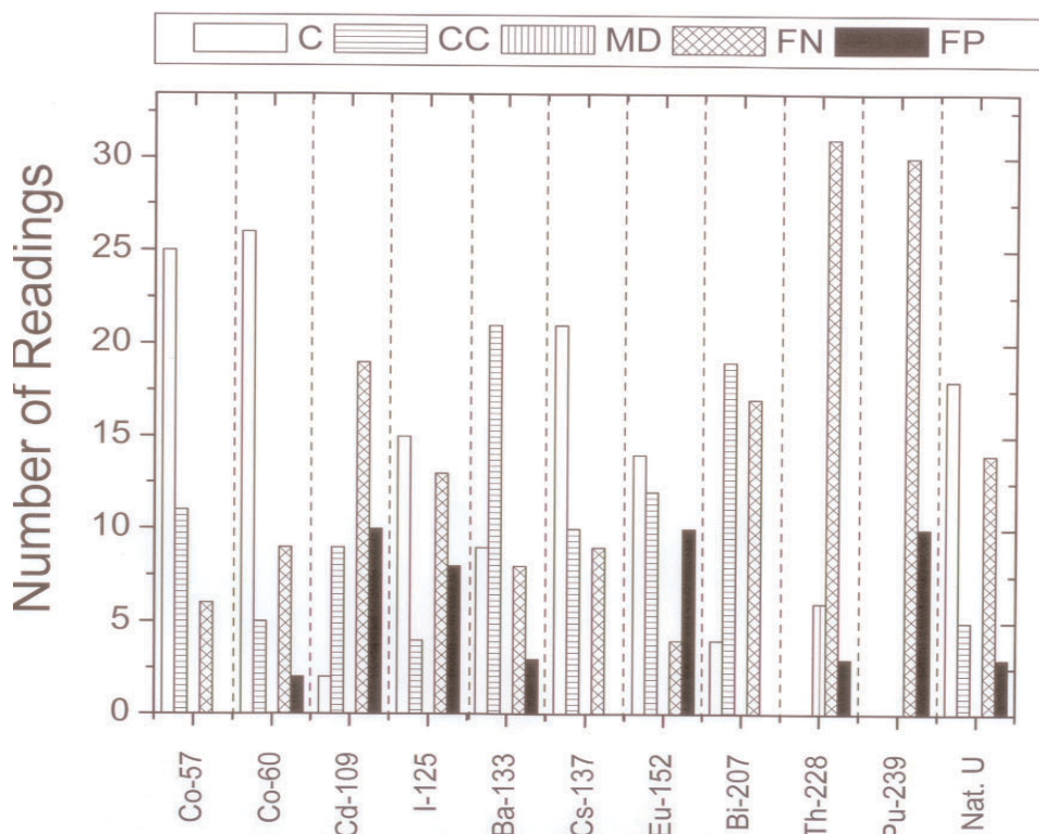
Fig. 2. Combined number of readings from all four detectors for each category, defined as correct, conditional-ly correct, minor daughter, false negative and false positive, for all radioactive sources measured.
