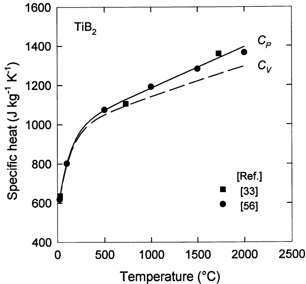
Fig. 15. Specific heat C_p of \text{TiB}_2 as a function of temperature. The solid curve is the fit of Eq. (14). The dashed curve is C_v calculated from Eq. (15).
