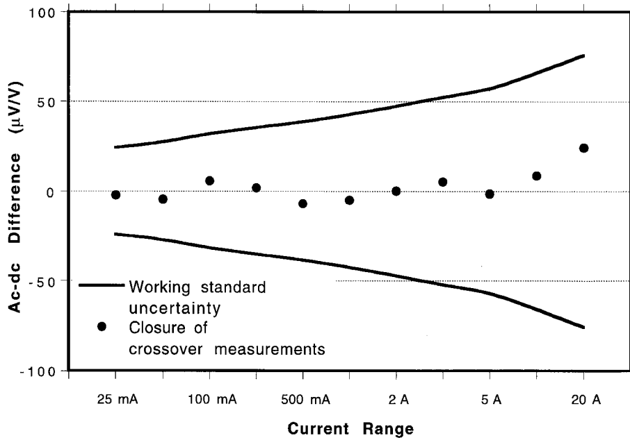
Fig. 6. Expanded uncertainties (in \mu\text{V}/\text{V} ) for the reference standards plotted with the closure between the buildup paths.
