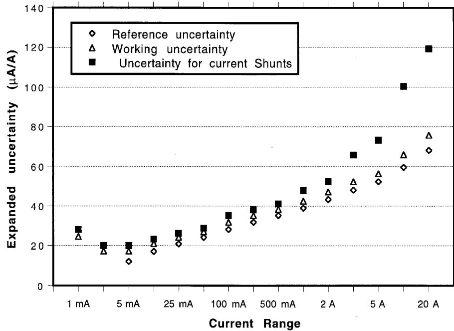
Fig. 5. Final, expanded uncertainties (in \mu\text{A}/\text{A} ) for thermal current converters at 100 kHz, calculated with a coverage factor of k = 2 , plotted together.
