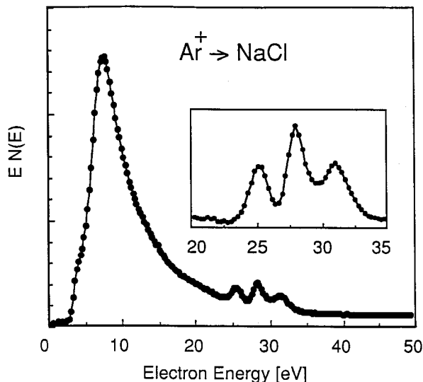
Fig. 1. Energy distributions of electrons emitted from a stoichiometric NaCl (100) single crystal surface bombarded with 3 keV Ar + ions. The inset shows the three peaks (assigned to autoionizing transitions of neutral sodium) after subtraction of a smooth background; energies are referenced to the vacuum level.
