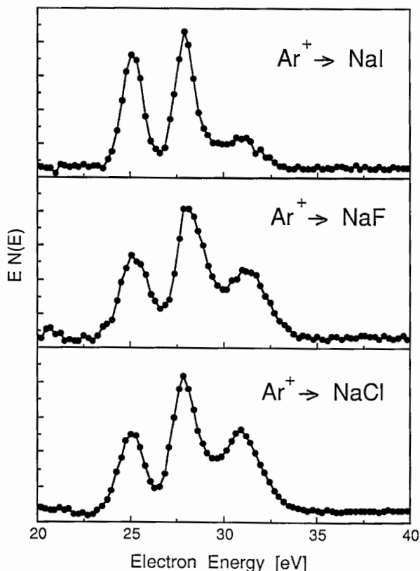
Fig. 2. Electron spectra obtained on several stoichiometric sodium halide crystal surfaces (NaCl, NaF, NaI) bombarded with 3 keV Ar + ions. The energies of each of the three sodium autoionizing transitions are the same for all of these halide surfaces. A smooth secondary electron background has been subtracted from the measured data to give the spectra shown here and in Fig. 3.
