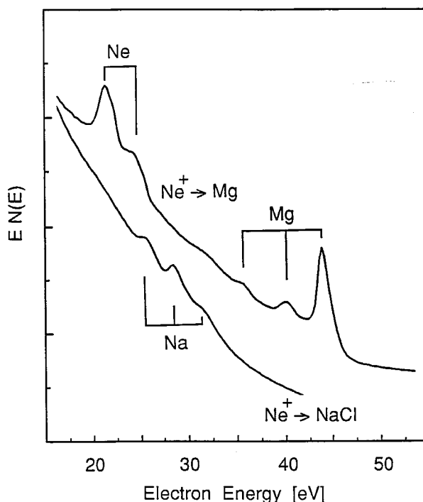
Fig. 9. \text{Ne}^+ bombardment-excited electron spectra for a stoichiometric NaCl and a clean metallic Mg surface; the incident \text{Ne}^+ projectile energy was 3 keV. The three Mg transitions have been assigned to deexcitation of \text{Mg}^{0**} and \text{Mg}^{+*} [14]. The two neon projectile excitation lines observed on Mg result from the deexcitation of neutral \text{Ne}^{0**} 2p^4 3s^2 \ ^3P (at about 20.5 eV) and ^1D (at about 23.5 eV) [40, 48] and indicate that the projectile ion is efficiently neutralized at the metal surface prior to excitation. (An additional weak feature is also observed at about 31 eV in the case of the \text{Ne}^+ bombarded Mg metal surface [40, 48, 51]. It has been assigned by Xu and Bonanno [48] to nonradiative deexcitation of a neon projectile with a triple 2p core hole ( \text{Ne}^{+,0} 2p^{-3} .) On NaCl, however, no such neutral neon transitions are observed; this result strongly suggests that the \text{Ne}^+ projectile ion is not neutralized at the ionic surface.
