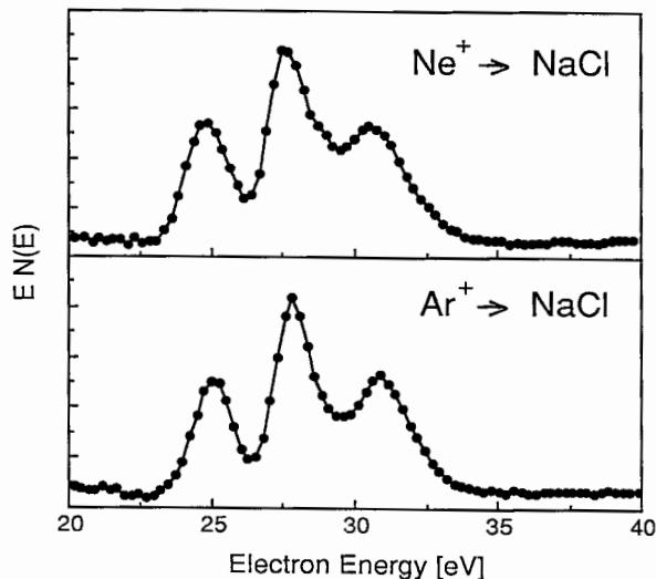
Fig. 3. Electron spectra obtained on stoichiometric crystal surfaces of NaCl bombarded with either 3 keV Ar + or Ne + ions. The set of three sodium transitions is virtually the same for both bombarding ions.
