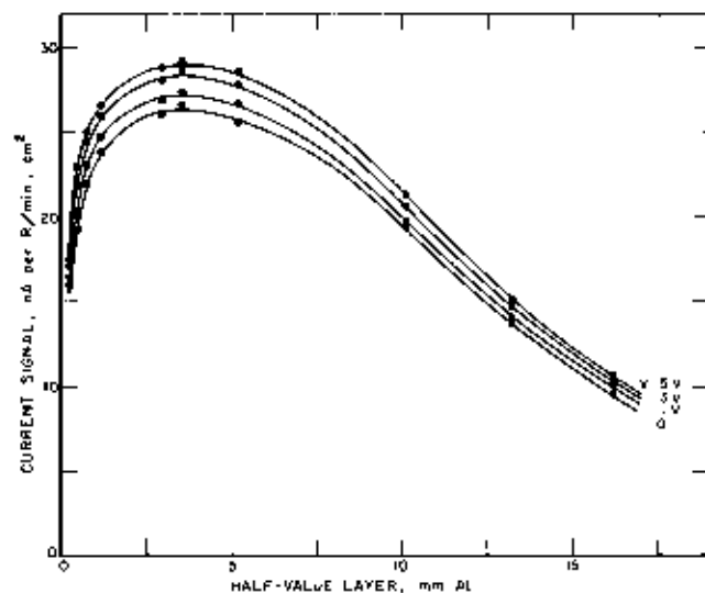
FIGURE 10. Dependence of current sensitivity (current signal at an exposure rate of 1 R/min and 1 cm 2 irradiated surface) on quality of moderately and lightly filtered x rays as measured with different voltages applied at the detector.
