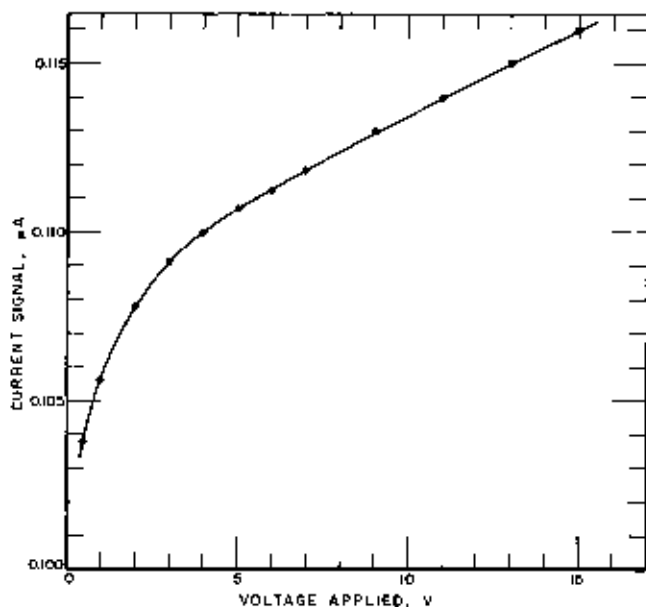
FIGURE 5. Voltage dependence of current signals produced by heavily filtered 100 kV x rays of 11.2 mm Al HVL at an exposure rate of approximately 2 R/min. Surface area of detector is approximately 2.5 cm 2 , R_L = 10^6 \Omega .
