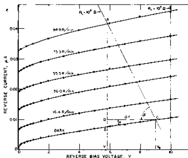
FIGURE 2. Reverse current-voltage characteristics of a silicon radiation detector of the diffused p-n junction type measured without irradiation and when fully irradiated with 30 kV x-rays of 0.09 mm Al HVL at different exposure rates with load lines indicated for two different load resistances.
