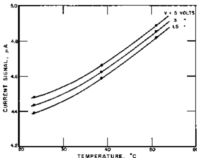
FIGURE 9. Temperature dependence of current signals measured with different voltages applied at the detector.
