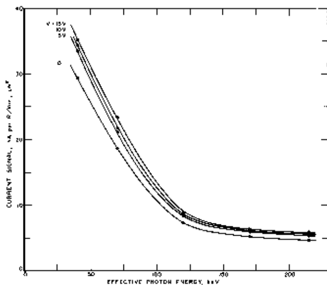
FIGURE 11. Dependence of current sensitivity (current signal at an exposure rate of 1 R/min and 1 cm 2 irradiated surface) on effective photon energy of heavily filtered x rays (see table 1 in part I) as measured with different voltages applied at the detector.
