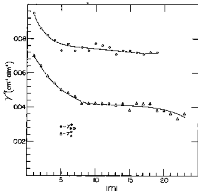
FIGURE 1.—A plot showing the broadening constants, \gamma^0 ( \text{cm}^{-1} \text{ atm}^{-1} ), for CO lines of the 2-0 band as a function of [m].
