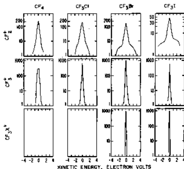
FIGURE 3. Ion current distribution in the ion beam for selected ions of the trifluoromethyl halides for 70-v electrons.
