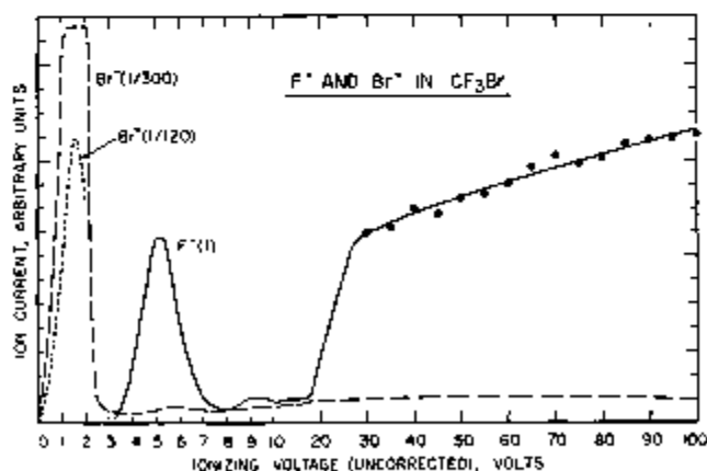
FIGURE 2. Ionization-efficiency curves for the \text{Br}^- and \text{F}^- ions of \text{CF}_3\text{Br} plotted on a linear scale.
