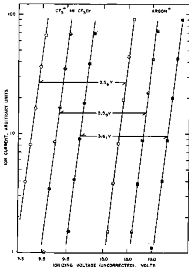
FIGURE 1. Repeat determinations of initial portions of the ionization-efficiency curves for the \text{CF}_3^+ ion of \text{CF}_3\text{Br} and the calibration gas, argon, plotted on a semilog scale.
