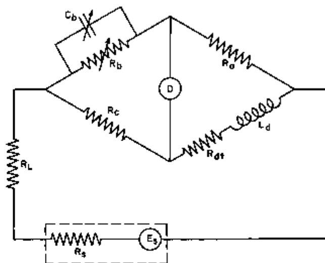
FIGURE 2. Maxwell-Wien bridge circuit.
