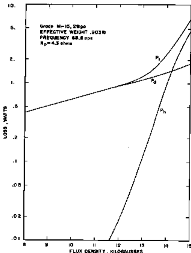
FIGURE 8. P_1 , P_h , and P_2 versus flux density for one specimen.
