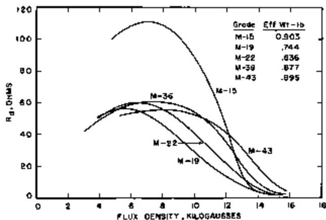
FIGURE 11. R_A versus flux density for five grades of materials.
