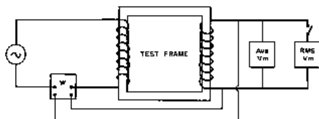
FIGURE 1. Connections for core-loss test, using wattmeter.
