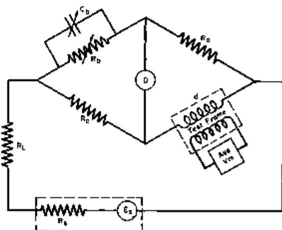
FIGURE 3. Maxwell-Wien bridge circuit for measuring core loss, using Epstein test frame.
