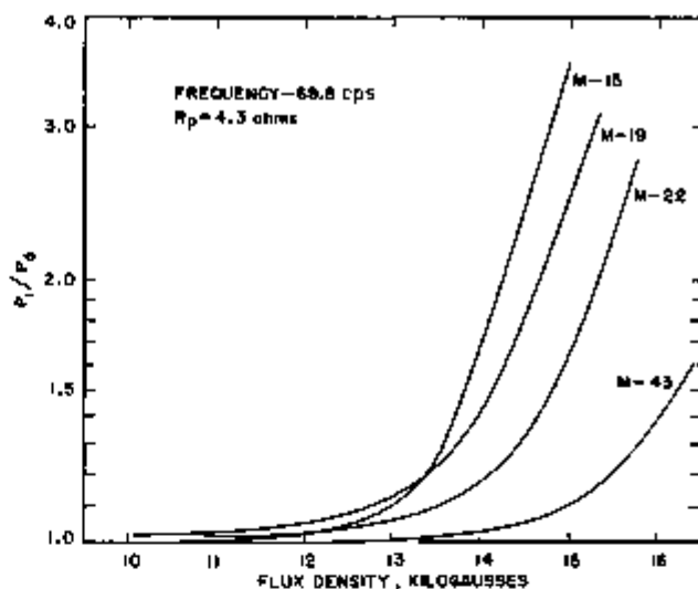
FIGURE 9. The ratio P_1/P_d versus flux density for four grades of materials.
