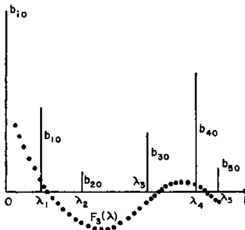
FIGURE 2. Attenuation behavior of algorithm II.
