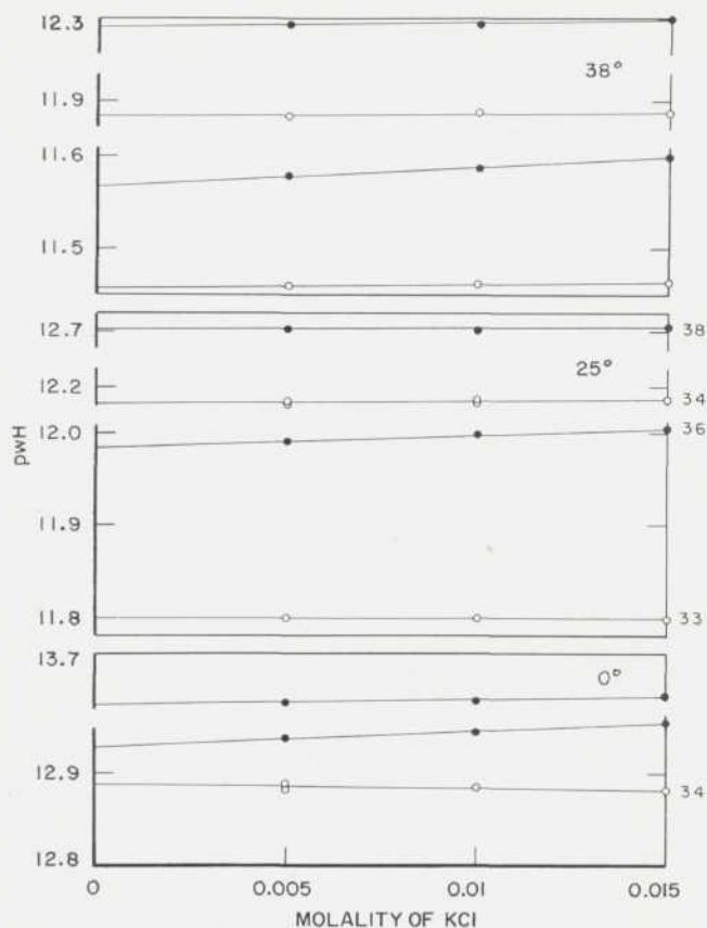
FIGURE 5. pH of trisodium phosphate and sodium hydroxide solutions as a function of the molality of added potassium chloride.
