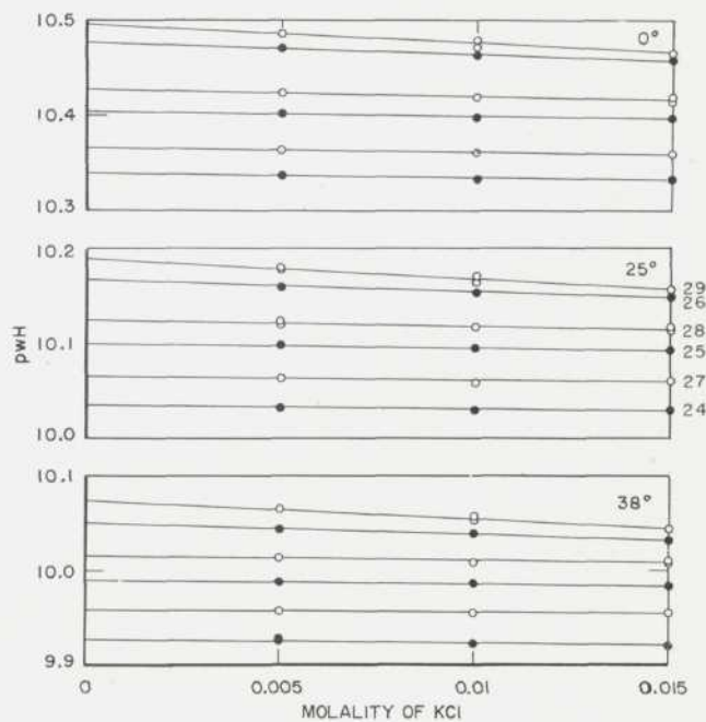
FIGURE 3. pH of bicarbonate-carbonate buffers as a function of the molality of added potassium chloride.
