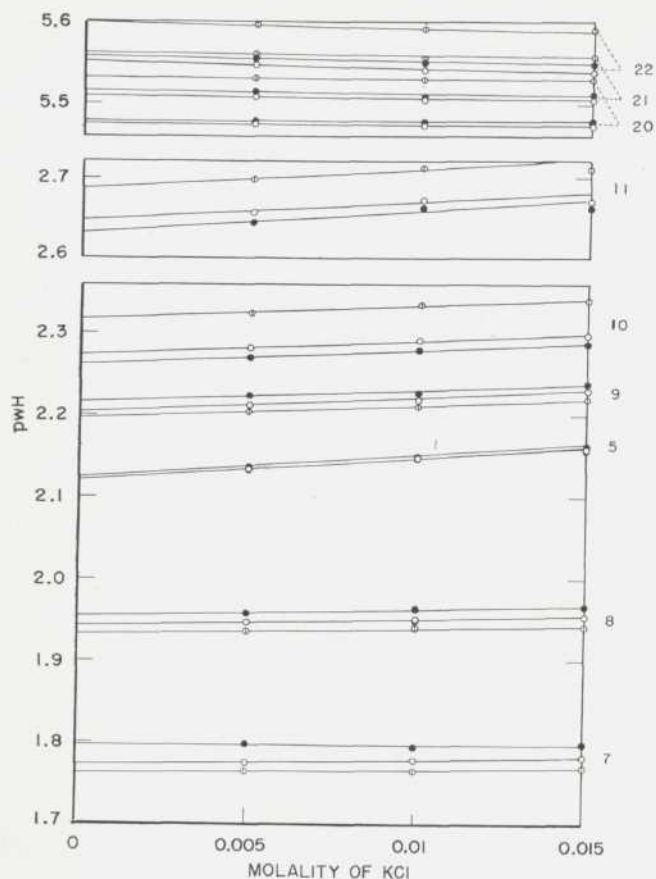
FIGURE 2. pH of acid solutions as a function of the molality of added potassium chloride.
