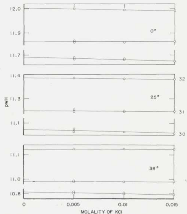
FIGURE 4. pH of sodium carbonate solutions as a function of the molality of added potassium chloride.
