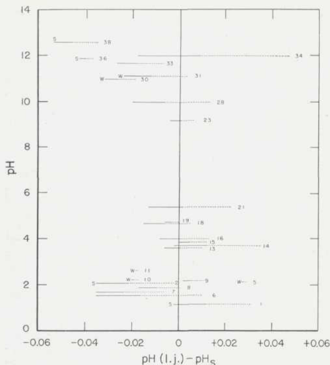
FIGURE 6. Liquid-junction error of the practical pH scale.
