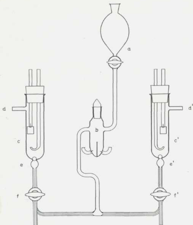
FIGURE 1. Cell vessel for emf measurements of cells of type II. a, Reservoir of saturated KCl; b, calomel electrode; c, c', hydrogen electrodes.
