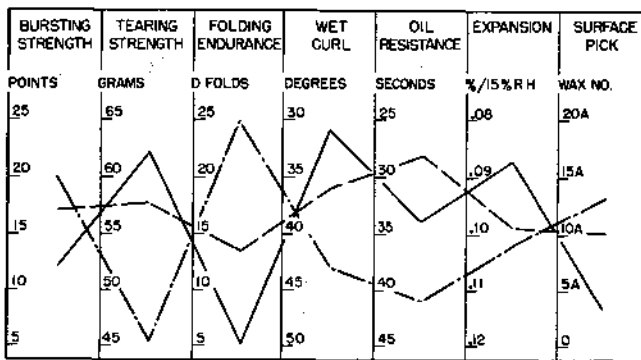
FIGURE 13. Effect of melamine resin in papers containing commercial hardwood soda pulp and coniferous sulfite pulp.
