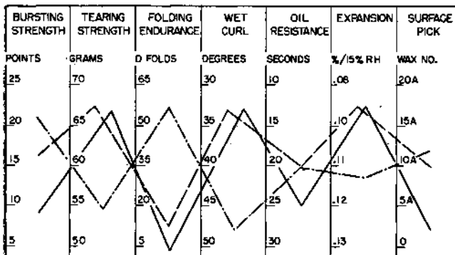
FIGURE 10. Effect of melamine resin in papers containing paper-birch sulfite pulp (FPL item 10).
