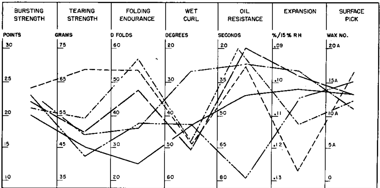
FIGURE 2. For papers containing 3 percent of melamine resin, the physical properties of experimental papers composed of 75-percent hardwood fibers and 25-percent sulfite softwood fibers are better in most instances than the papers composed of 50-percent commercial soda hardwood fibers and 50-percent commercial sulfite softwood fibers.
