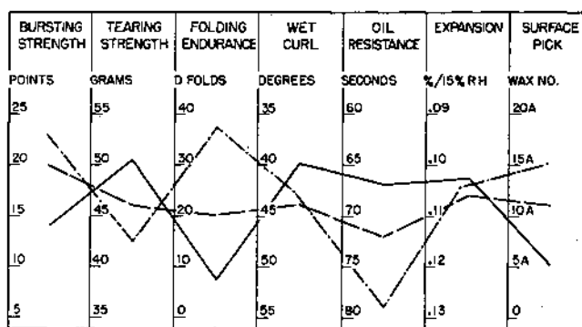
FIGURE 7. Effect of melamine resin in papers containing aspen sulfite pulp (FPL item 16).
