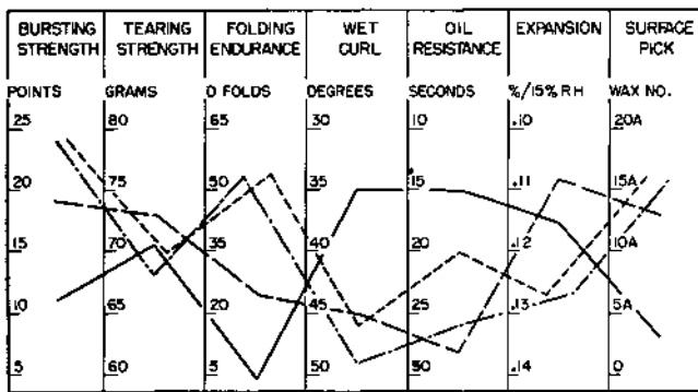
FIGURE 9. Effect of melamine resin in papers containing black gum sulfite pulp (FPL item 8).
