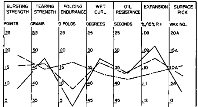
FIGURE 12. Effect of melamine resin in papers containing Douglas-fir neutral sulfite pulp (FPL item 13).
