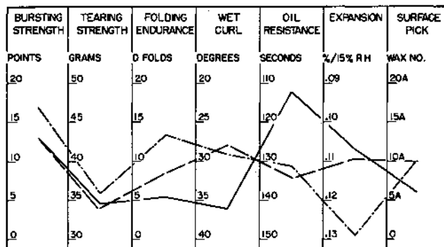
FIGURE 4. Effect of melamine resin in papers containing peroxide-bleached aspen groundwood pulp (FPL item 2).
