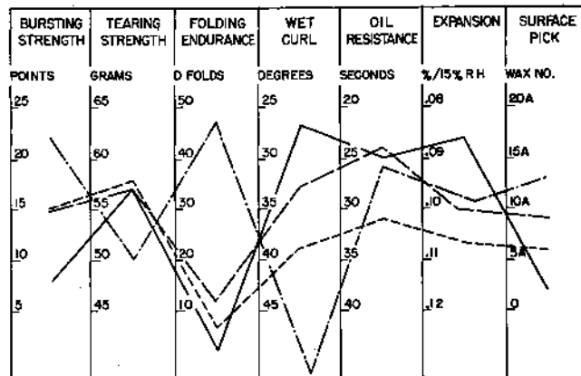
FIGURE 5. Effect of melamine resin in papers containing aspen sulfate pulp (FPL item 7).
