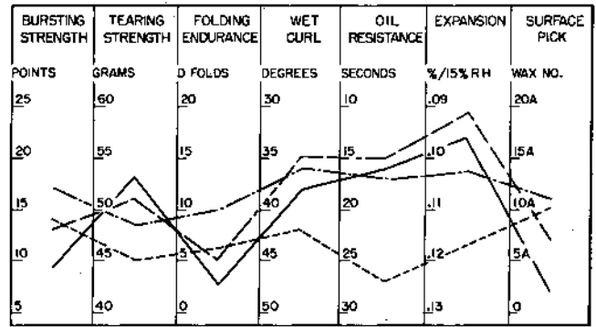
FIGURE 11. Effect of melamine resin in papers containing beech sulfate pulp (FPL item 12).
