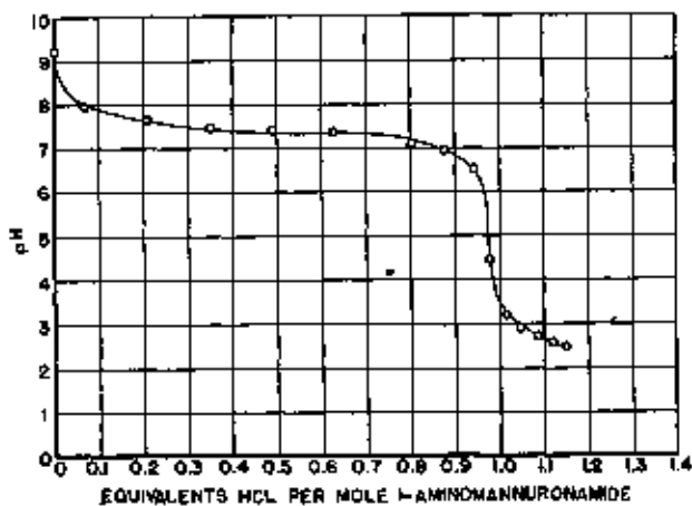
FIGURE 1. pH titration curves for 1-aminomannuronamide. 0.1 N HCl added portionwise to 75 ml of a solution containing 0.275 g of 1-aminomannuronamide.
