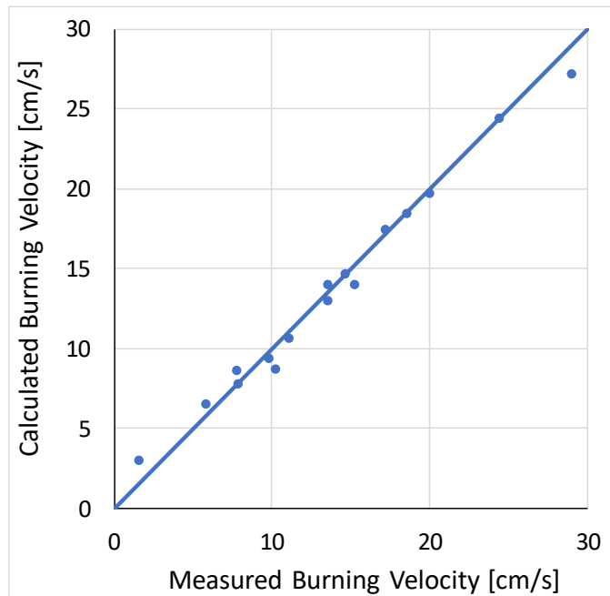
Figure 4.2-8. Calculated vs. measured laminar burning velocity (peak over all \phi ) of twenty-one refrigerant/N 2 /O 2 flames for which experimental data are available in the literature [66-68]
