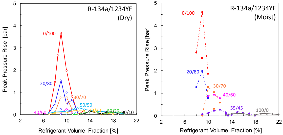
Figure 4.2-5. Explosion pressure in the JHPGL test for binary blends of HFC-134a with HFO-1234yf as function of volume fraction the blend in air. Different curves show results for varying volume fractions of HFC-134a/HFO-1234yf in the blend (left frame: dry air; right: moist).
