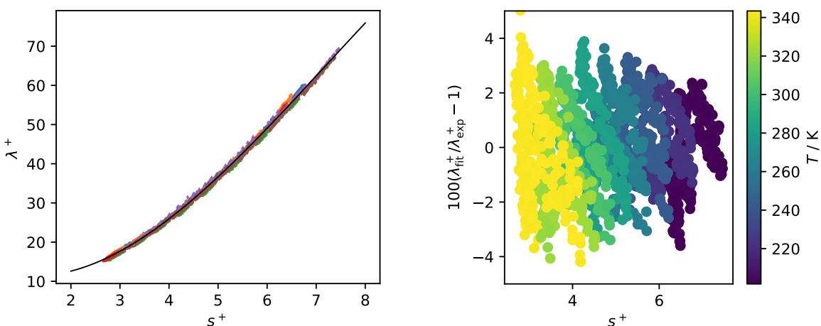
Figure A.1-19. Entropy scaling model for the thermal conductivity of the three blends studied here; (a) plus-scaled thermal conductivity \lambda_+ as a function of reduced scaled residual entropy s_+ , the different symbols denote the different measured blends; (b) relative deviations in \lambda_+
