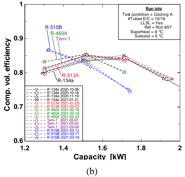
Figure 4.3-7. Compressor volumetric efficiency (a) without LLSL-HX and (b) with LLSL-HX
