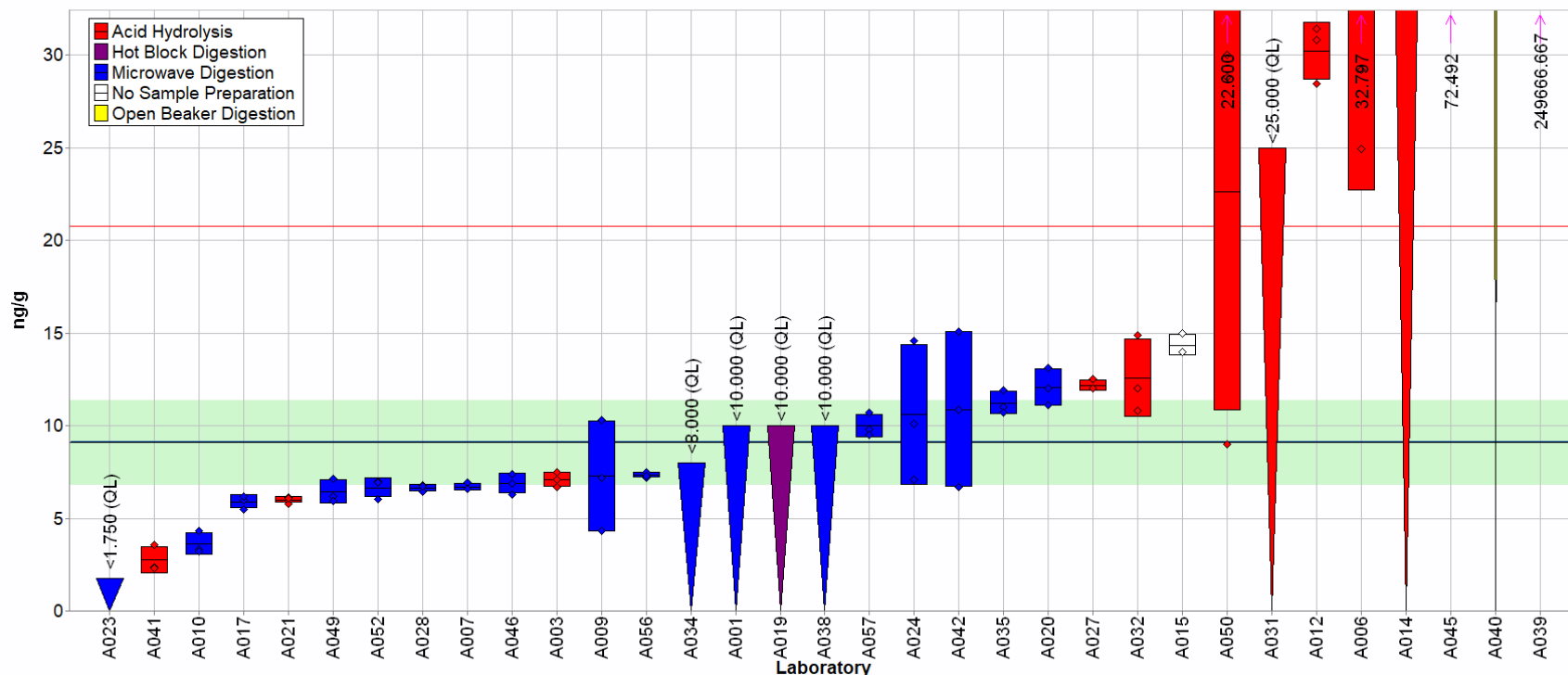
Fig. 3-5. Lead in Baby Food A (data summary view – sample preparation method).
