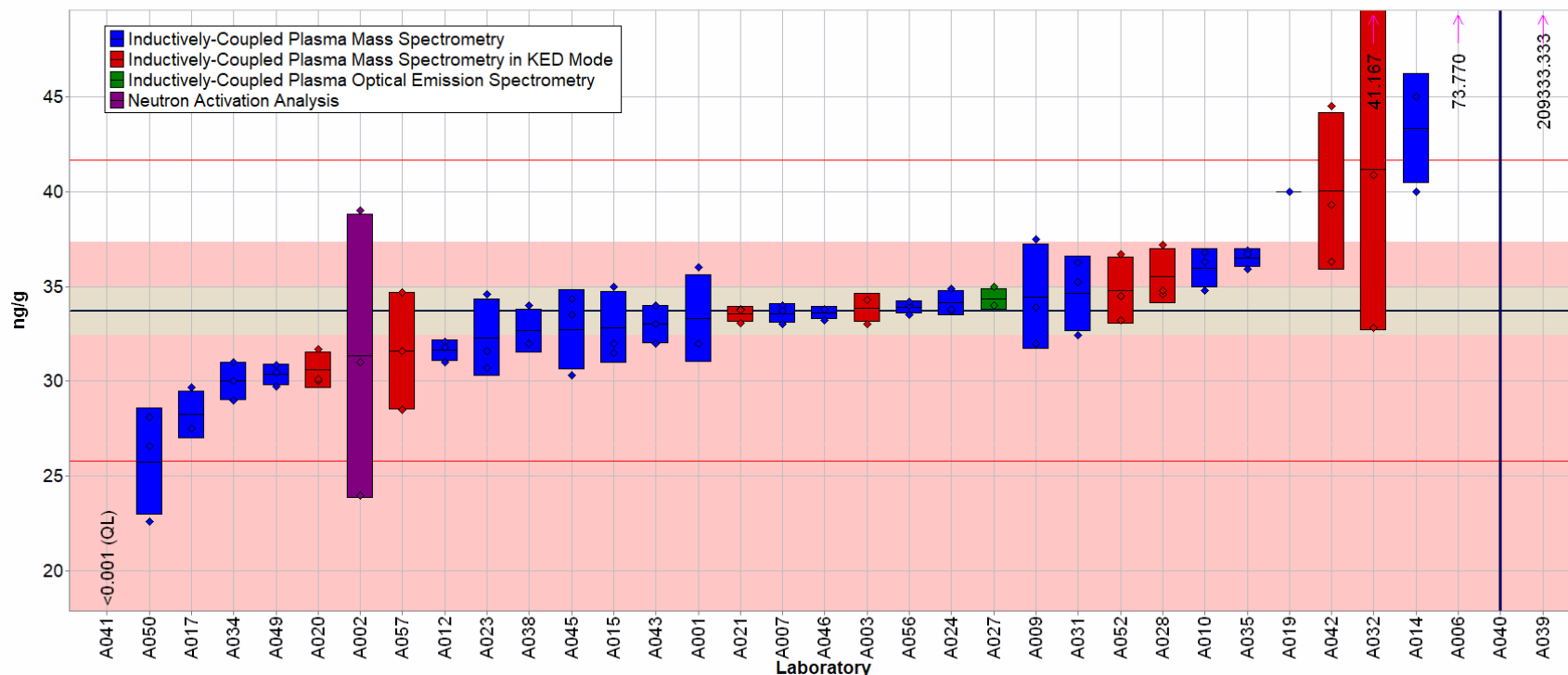
Fig. 3-9. Arsenic in Baby Food A (data summary view – analytical method).
