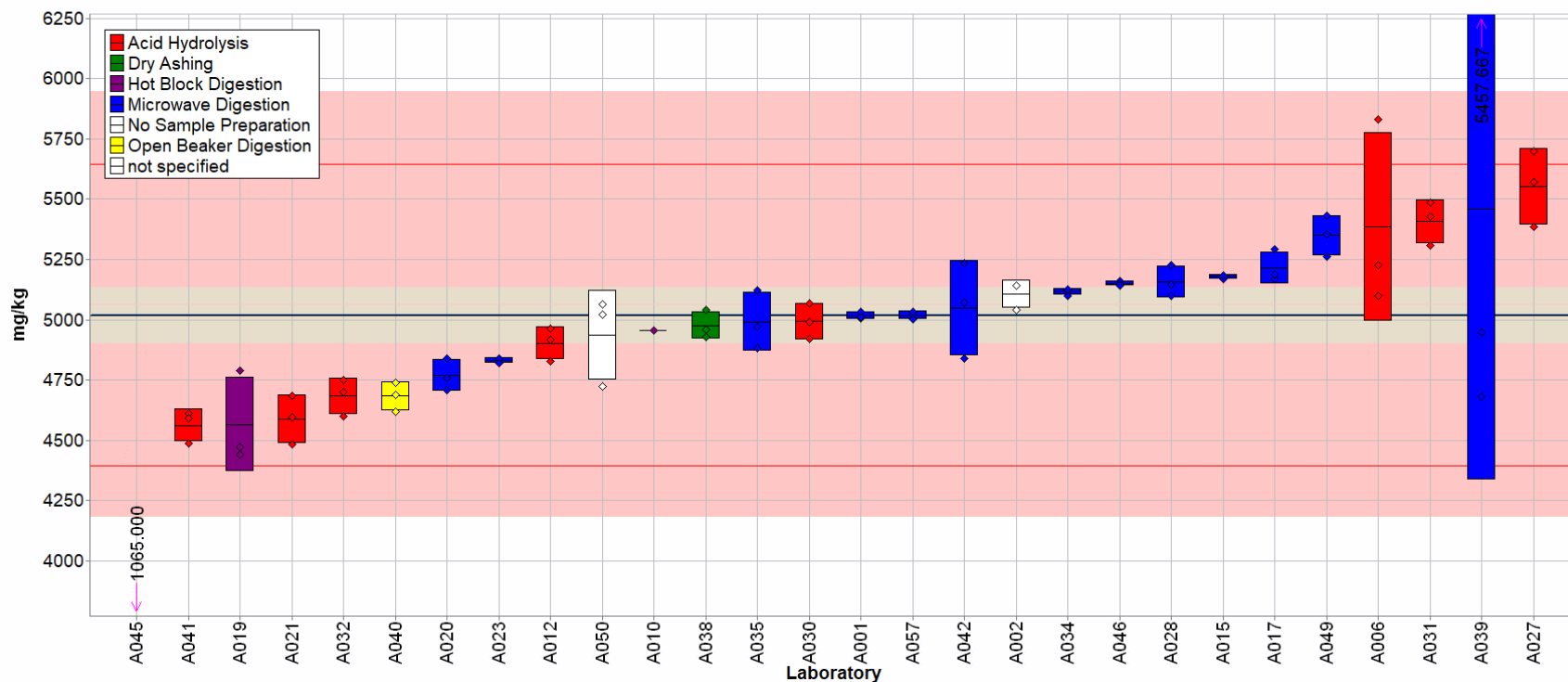
Fig. 2-1. Calcium in SRM 1849b (data summary view – sample preparation method).
