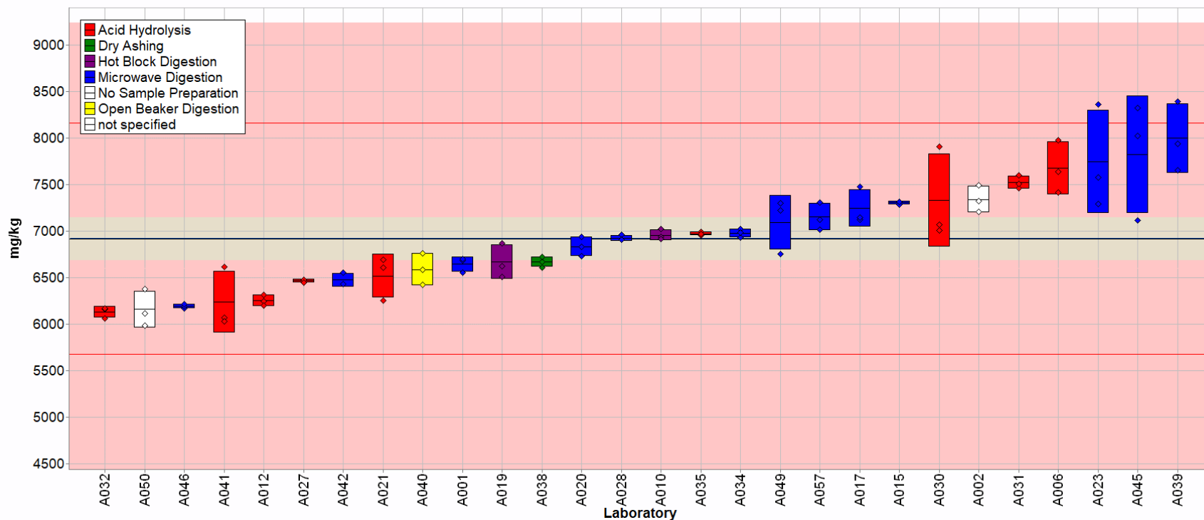
Fig. 2-6. Potassium in RM 8260 (data summary view – sample preparation method).
