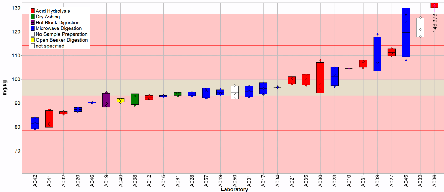
Fig. 2-4. Iron in RM 8260 (data summary view – sample preparation method).
