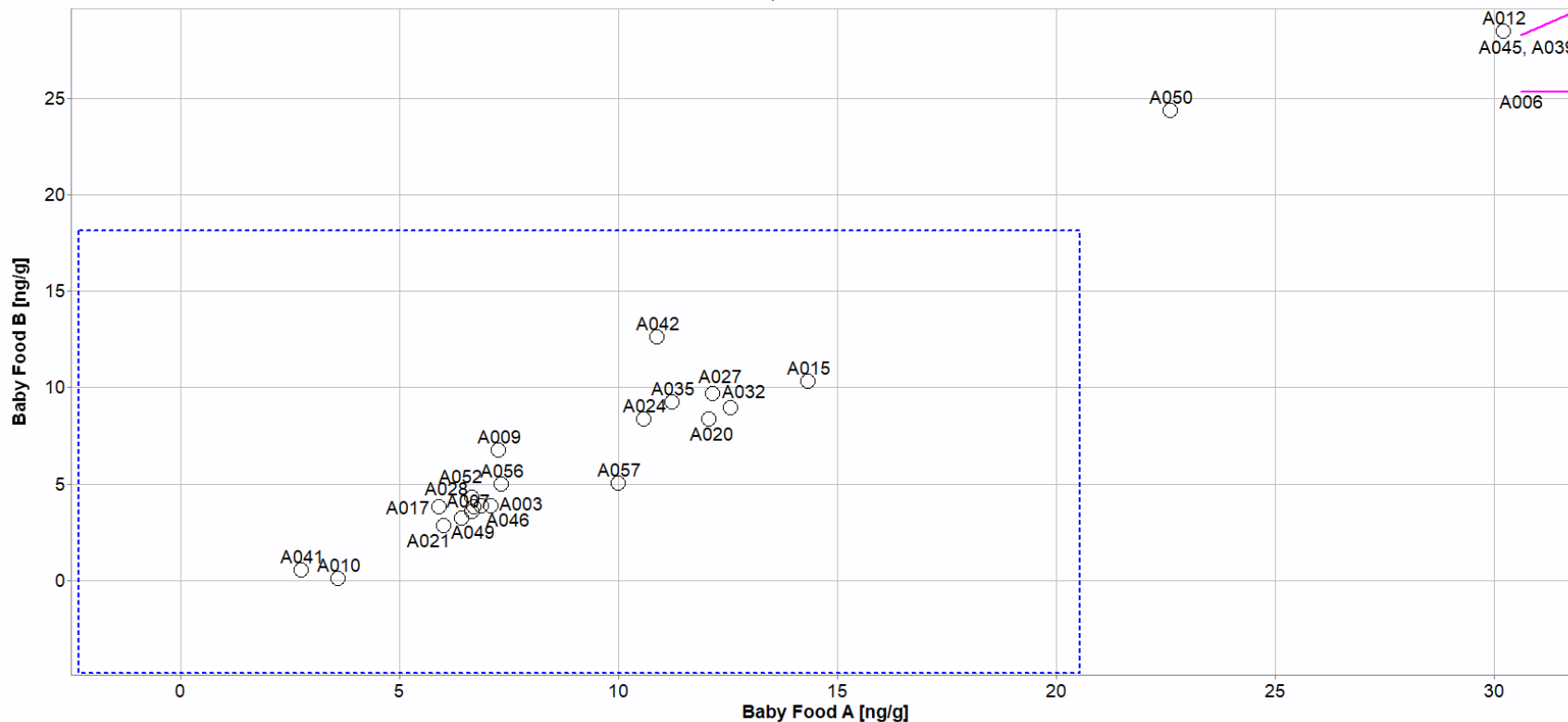
Fig. 3-19. Laboratory means for lead in Baby Food A and Baby Food B (sample/sample comparison view).
