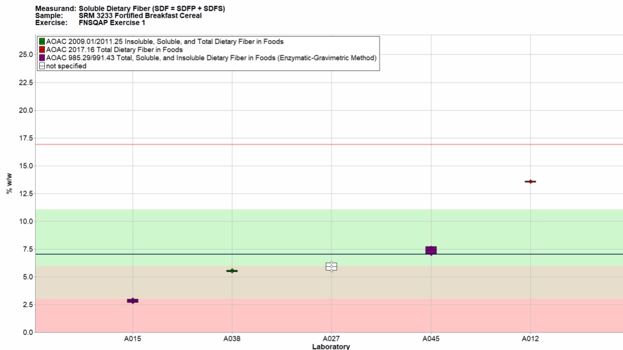
Fig. 8-7. Soluble dietary fiber (SDF) in SRM 3233 (data summary view – analytical method).
