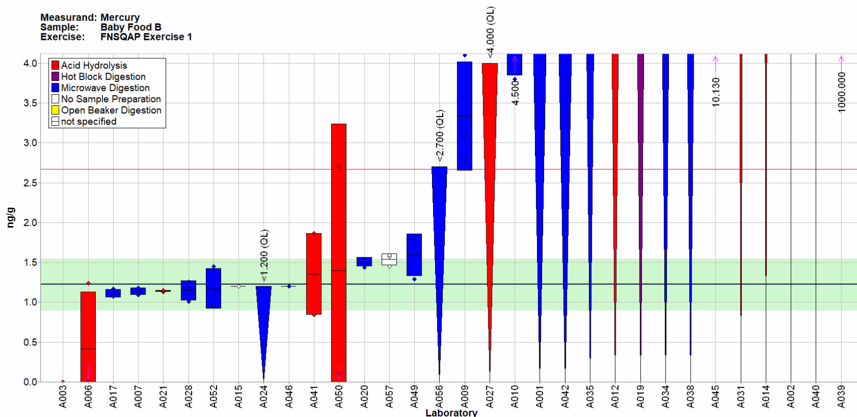
Fig. 3-8. Mercury in Baby Food B (data summary view – sample preparation method).
