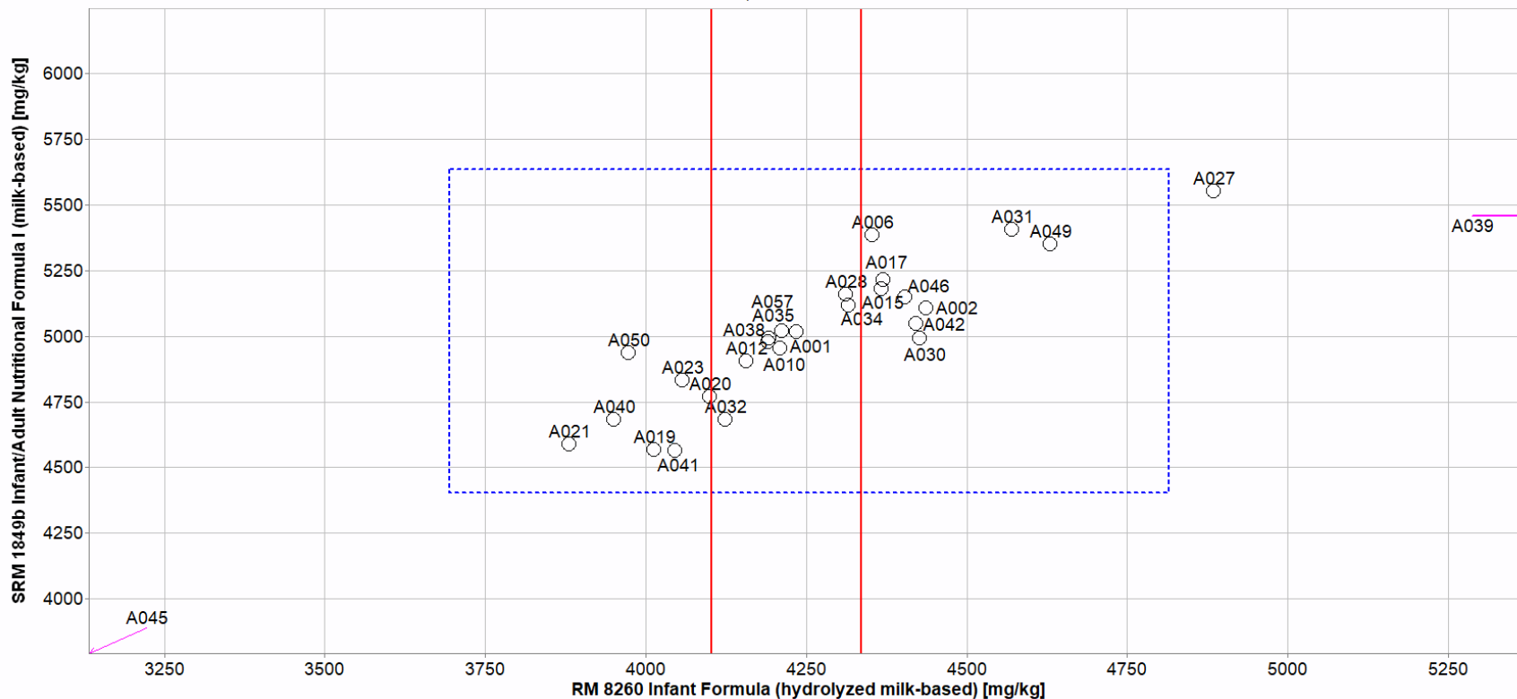
Exercise: FNSQAP Exercise 1, Measurand: Calcium No. of laboratories: 28, Correlation coefficient: 0.9
