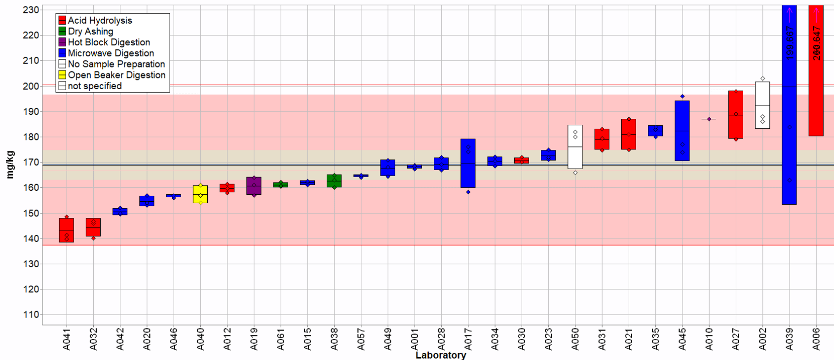
Fig. 2-3. Iron in SRM 1849b (data summary view – sample preparation method).
