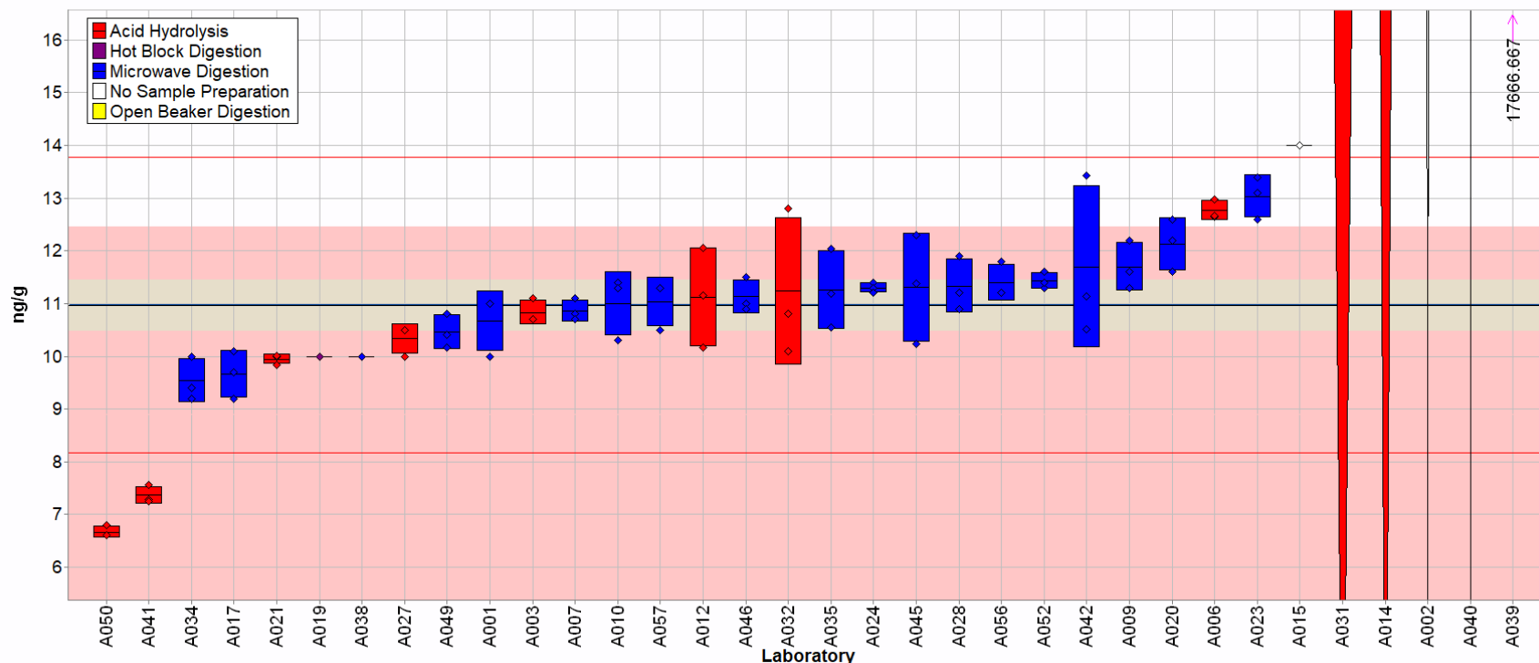
Fig. 3-4. Cadmium in Baby Food B (data summary view – sample preparation method).
