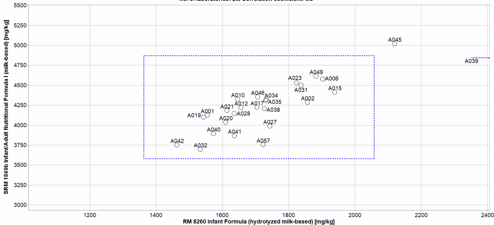
Fig. 2-20. Laboratory means for sodium in RM 8260 and SRM 1849b (sample/sample comparison view).
