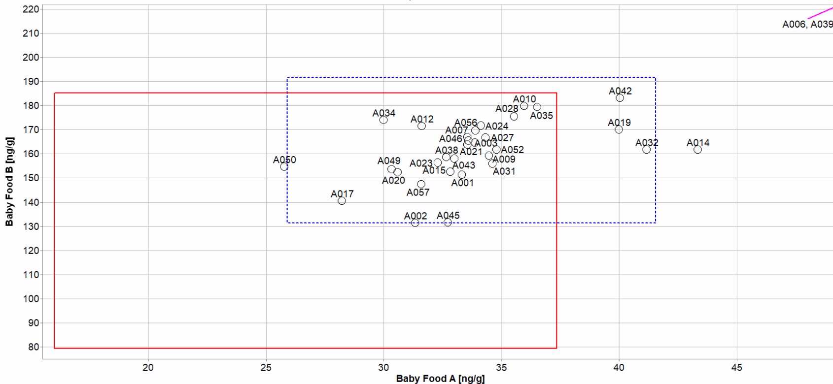
Fig. 3-17. Laboratory means for arsenic in Baby Food A and Baby Food B (sample/sample comparison view).
