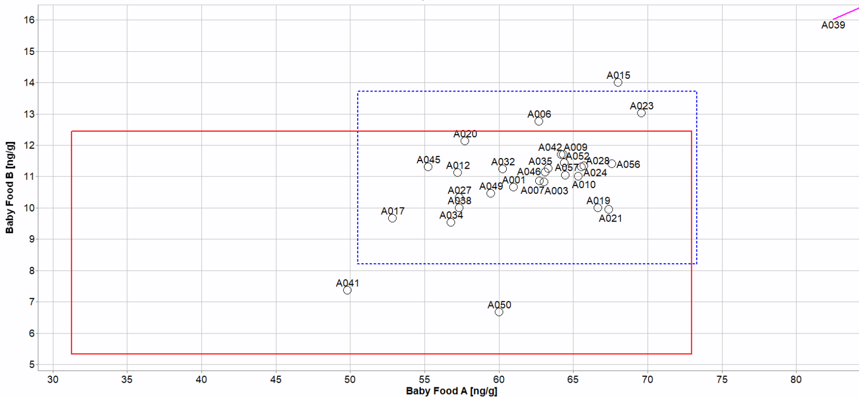
Fig. 3-18. Laboratory means for cadmium in Baby Food A and Baby Food B (sample/sample comparison view).
