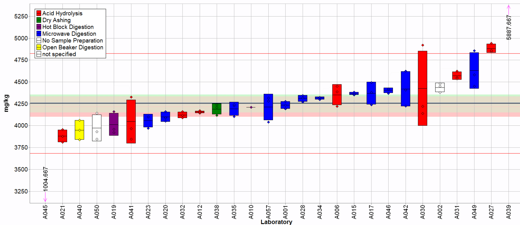
Fig. 2-2. Calcium in RM 8260 (data summary view – sample preparation method).
