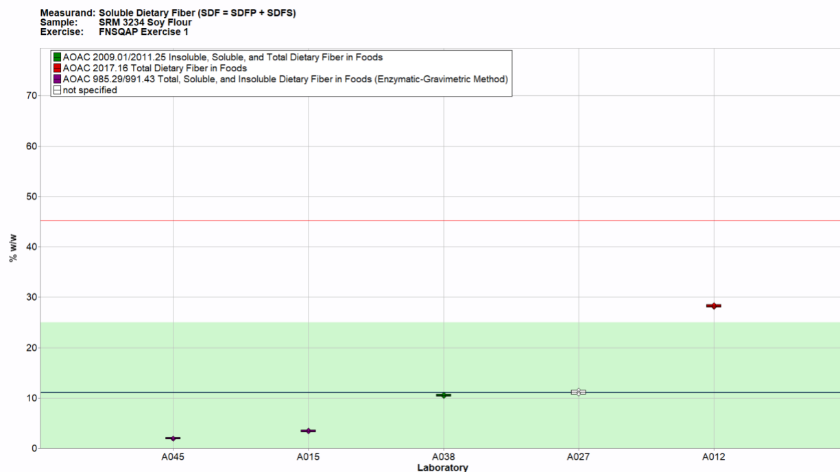
Fig. 8-8. Soluble dietary fiber (SDF) in SRM 3234 (data summary view – analytical method).
