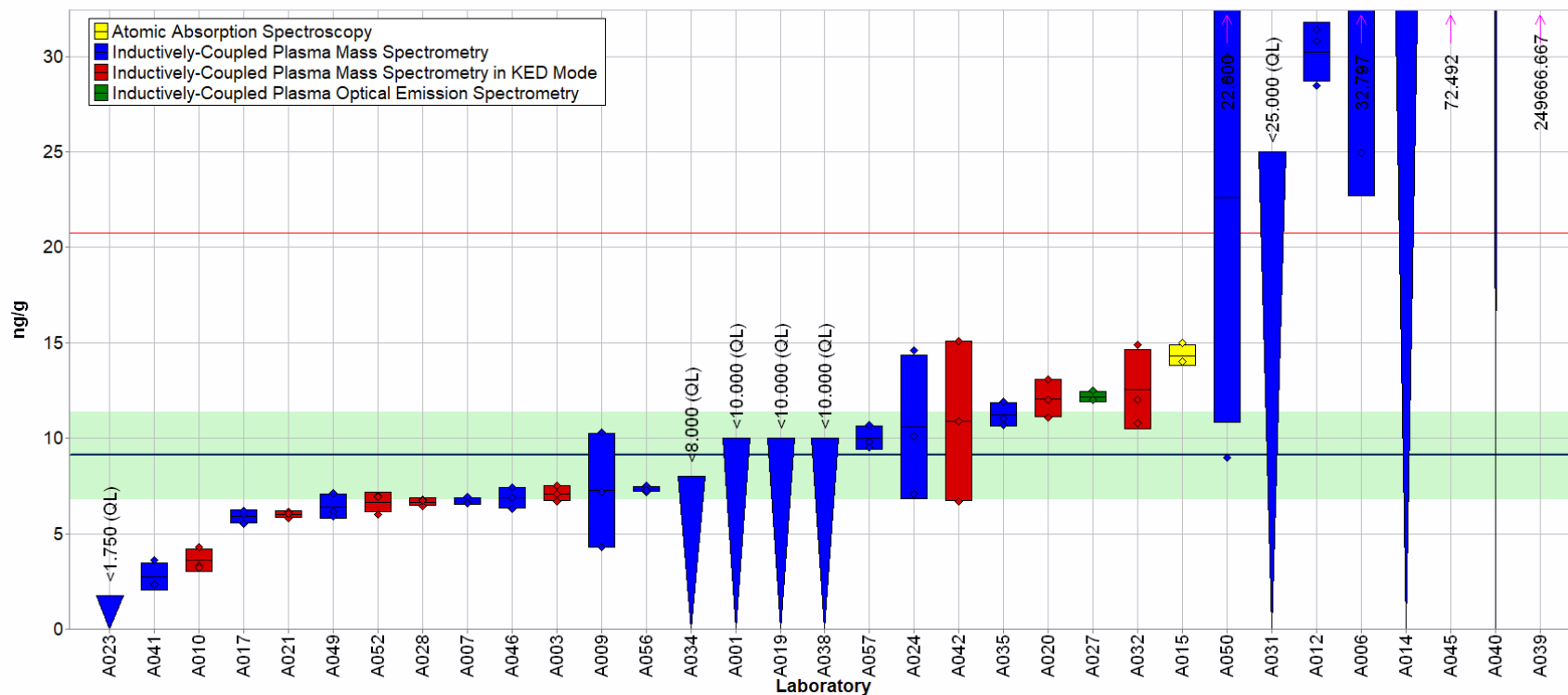
Fig. 3-13. Lead in Baby Food A (data summary view – analytical method).
