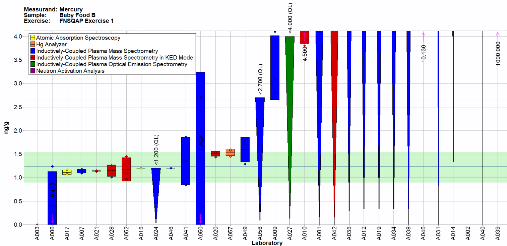
Fig. 3-16. Mercury in Baby Food B (data summary view – analytical method).
