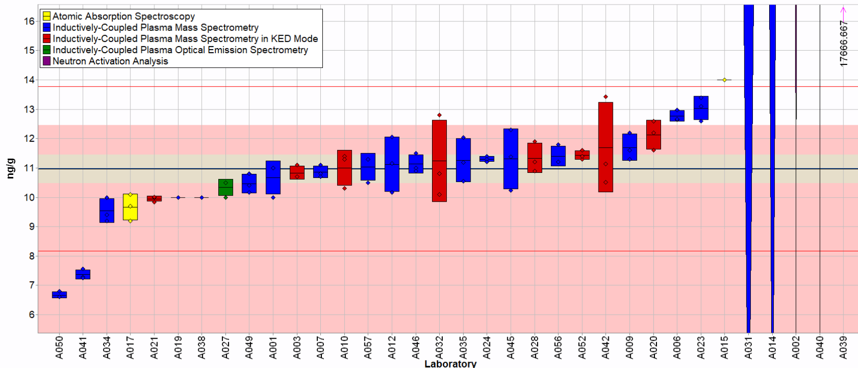
Fig. 3-12. Cadmium in Baby Food B (data summary view – analytical method).
