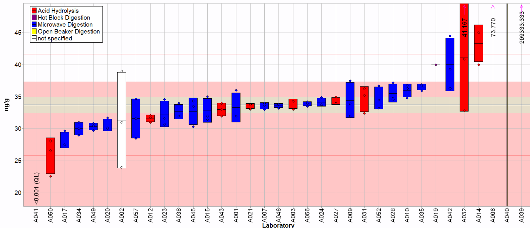
Fig. 3-1. Arsenic in Baby Food A (data summary view – sample preparation method).
