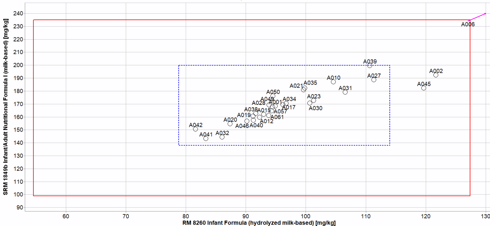
Exercise: FNSQAP Exercise 1, Measurand: Iron No. of laboratories: 29, Correlation coefficient: 0.9
