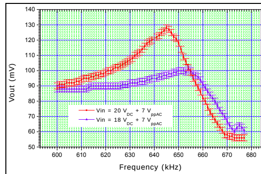
Figure 6: Electrical readout of the cantilever's oscillation amplitude.
