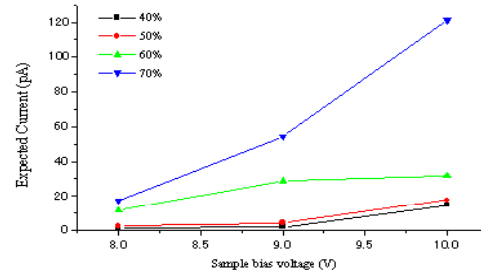
Fig. 4 Expected current from volume of fabricated dots (10 s).
