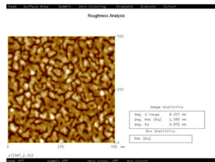
Figure 5. AFM images of the surfaces of a thin (~ 8 nm) aluminum layer deposited on oxidized silicon
