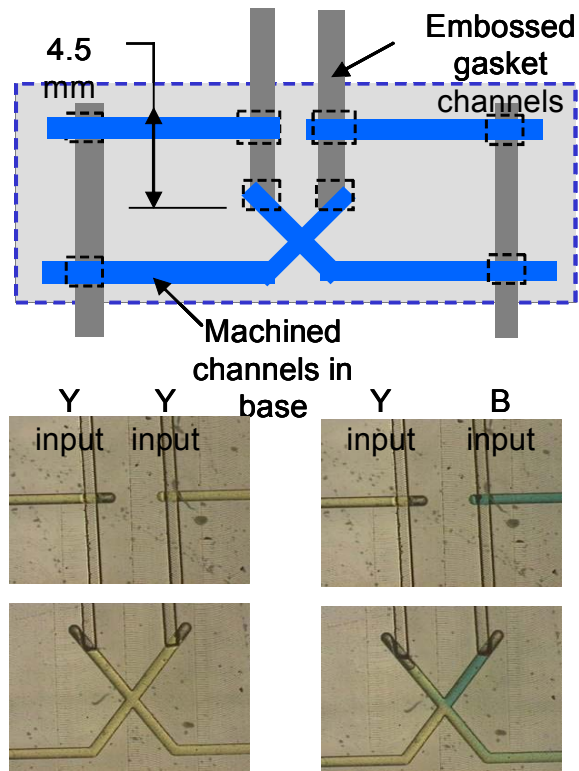
Figure 8 : Gasket/machined channel flow
