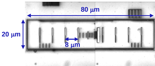
Fig. 3. Markers of a nominal 8 \mu m pitch.
