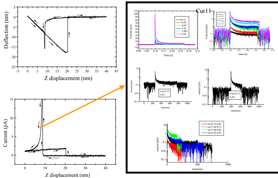
Figure 4. Current detection during oxidation
