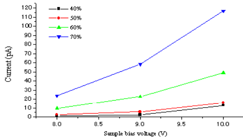
Fig. 3 Relation between total current for oxidation (10 s) and applied voltage at various humidity.
