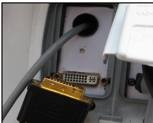
Figure 35: Locate the DVI-D bulkhead port on the trailer exterior. Connect the exterior monitor cable.
