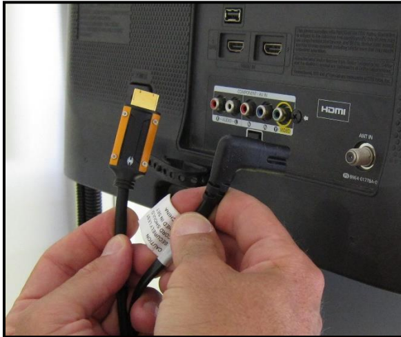
Figure 19: Connect the HDMI and power cable to the external field view monitor. The HDMI cable is attached to the internal bulkhead.
