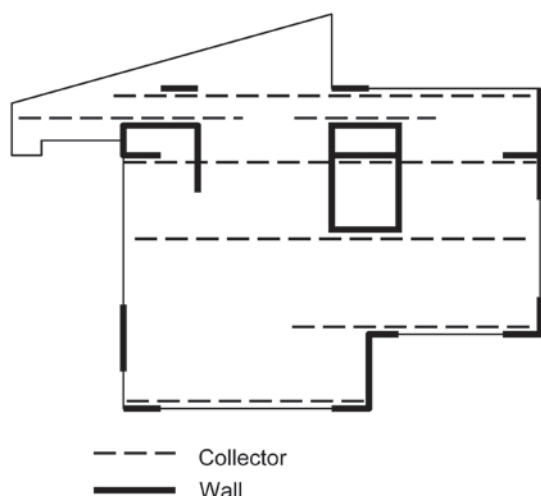
Figure 6-4 – Irregularly-shaped diaphragm.
