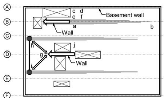
Figure 6-11 – Challenging design conditions.
