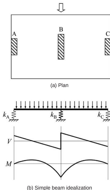
Figure 6-1 – Equivalent beam-on-springs model.
