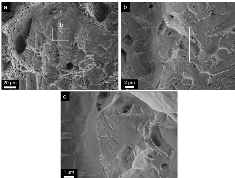
a) Mixed mode fracture and inclusion lift-outs, b-c) cleavage fracture surface.
