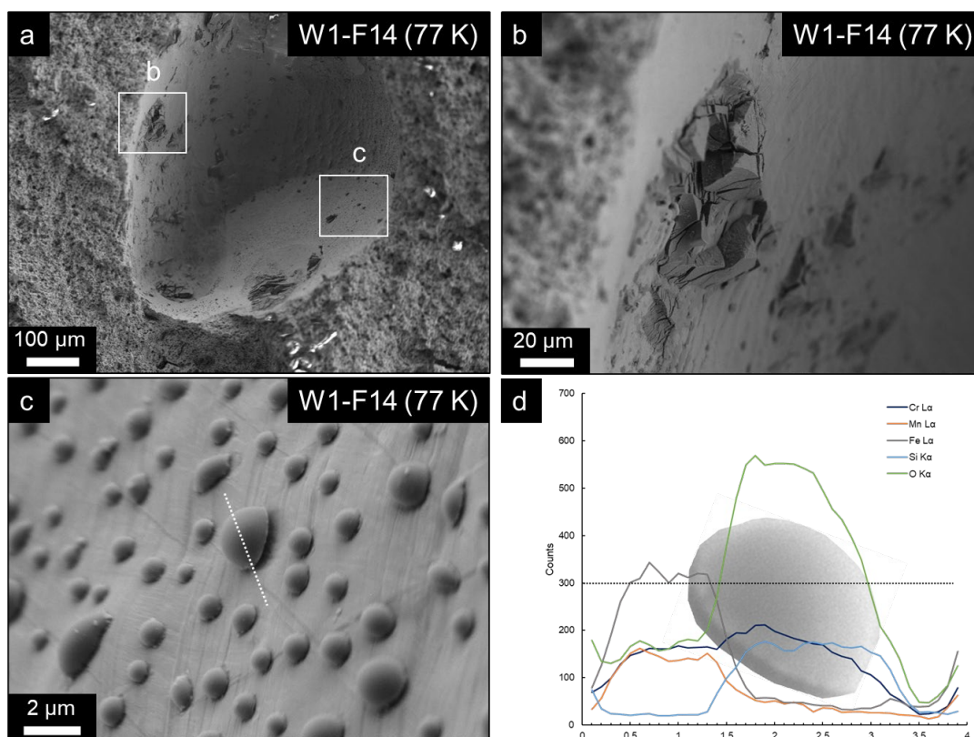
Figure 19 – a) Wormhole morphology at higher magnification, b) signs of residual material from the pre-formation, c) hemispherical inclusions on the surface of the pore cavity with dashed line indicating region of EDS line scan, d) EDS line scan of the hemispherical inclusion.
