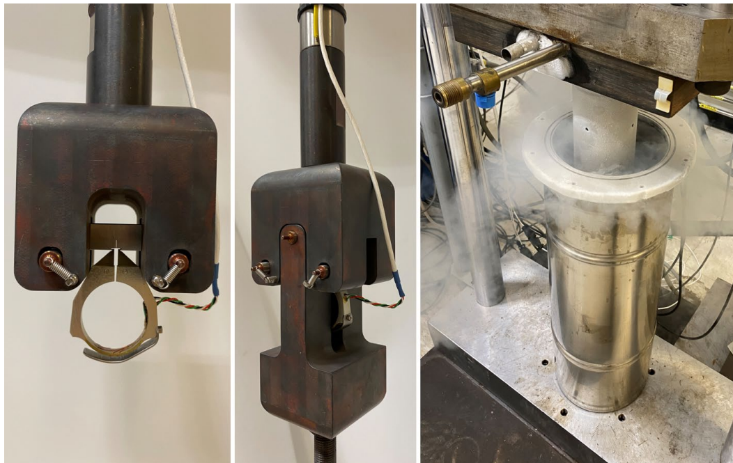
Figure 3 – (Left) Fracture toughness specimen placed in the upper fixture with the clip gage attached and (middle) lower fixture placed over the specimen and 3 rd loading pin inserted above the specimen. (Right) The sheath that protects the experimental setup and enables load bearing on the specimen is lowered into a double-walled cylinder filled with LN2.
