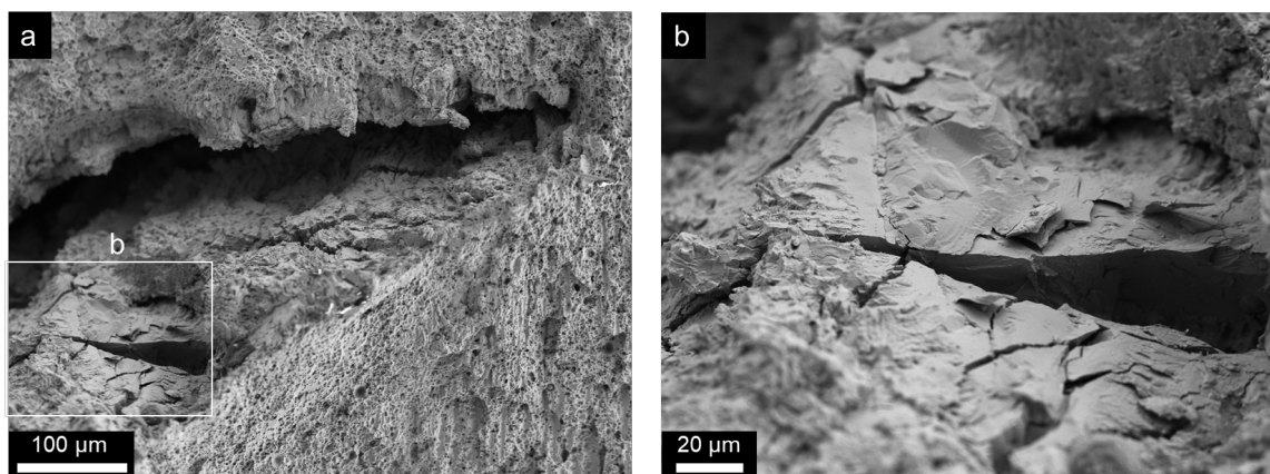
a) Crack jump, b) cleavage fracture
