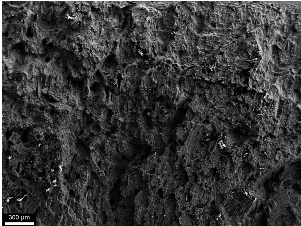
Large FOV displaying lack of fusion porosity.
