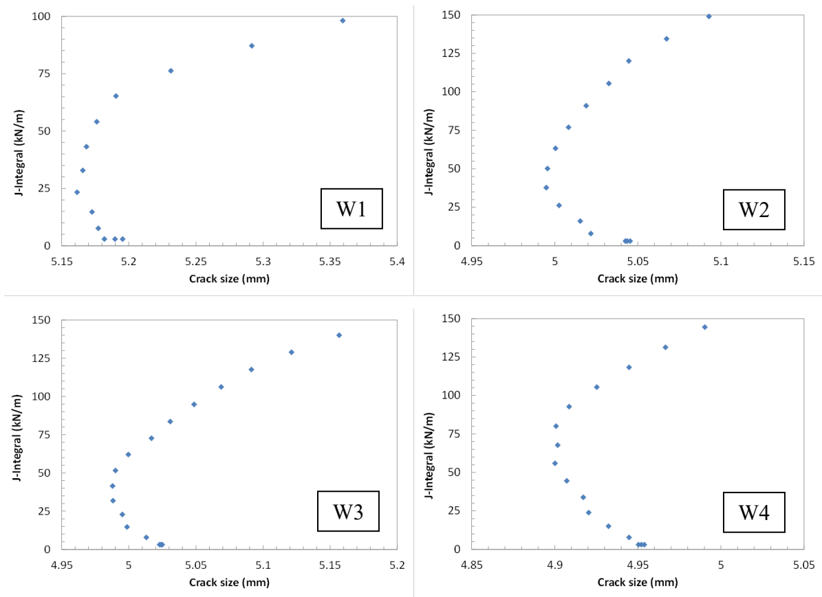
Figure 39 - Examples of apparent negative crack growth observed at 77 K on all investigated welds.
