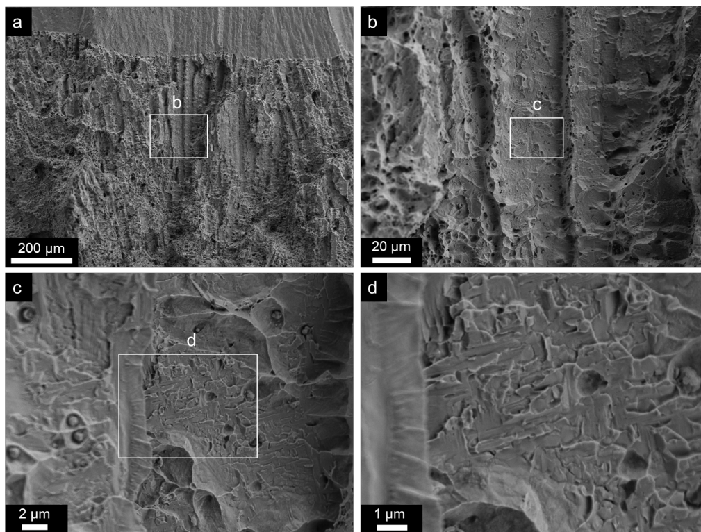
a) Crack paths near the precracked region, b) enlarged view, c—d) cleavage facets.
