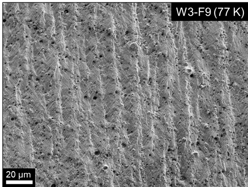
Figure 17 – Representative SE image of the precracked region of a weld specimen.
