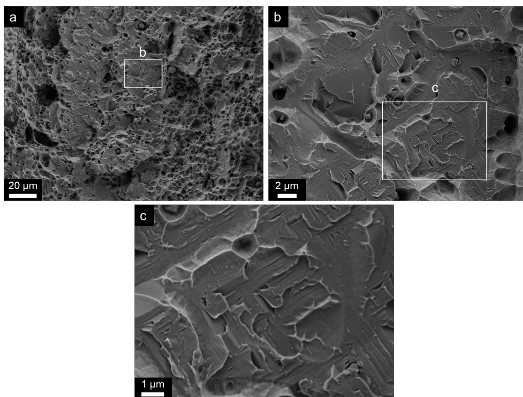
a) Crack paths showing brittle fracture, b—c) higher magnification of the cleavage facets.
