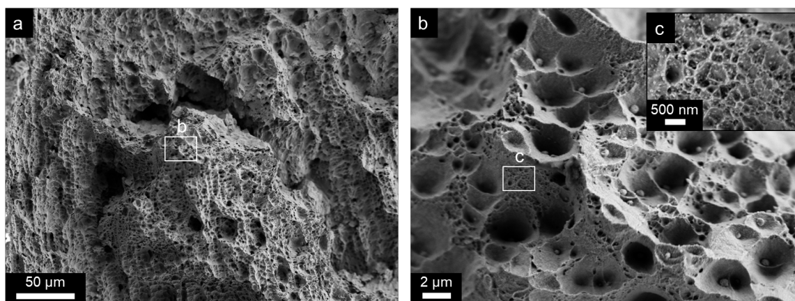
a) Crack jump, b) MVC, c) nanovoids.
