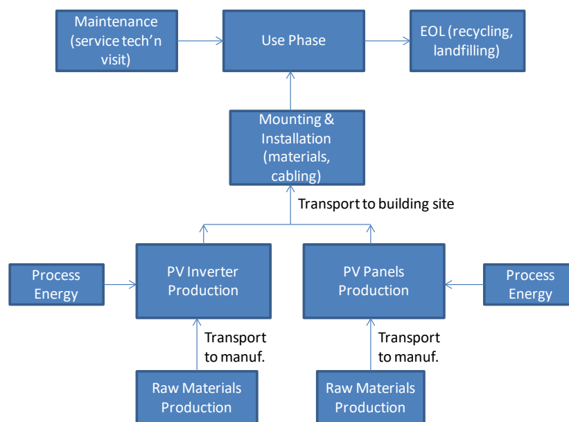
Figure 4-2 Solar Photovoltaic System Boundaries
