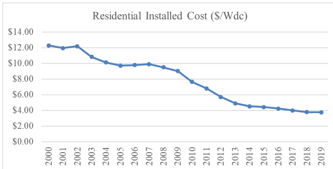
Figure 1-2 Residential Solar Gross Installed Cost Per Watt - Direct Current ( W_{dc} ) (2000-2019)
