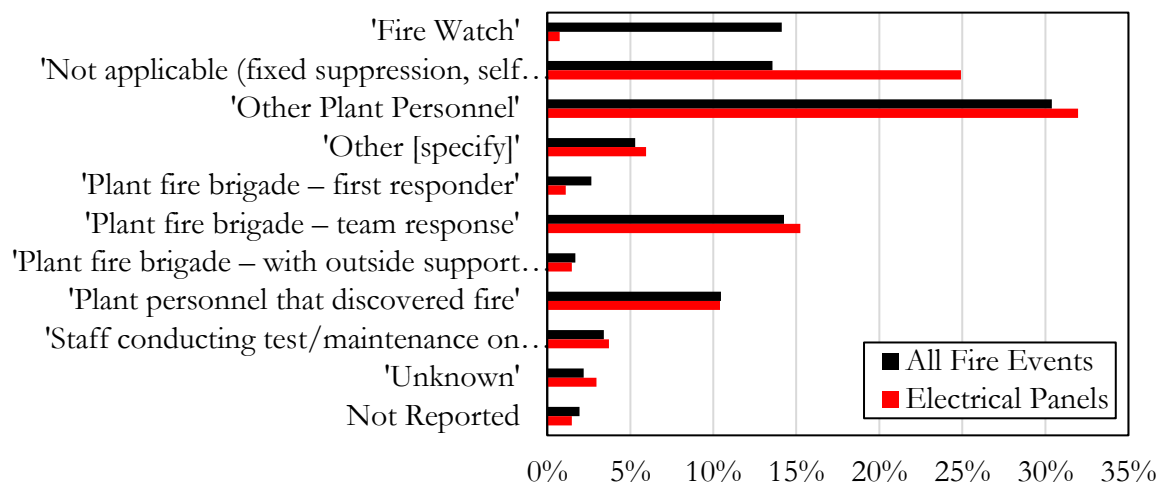
Figure 20. Fire Extinguishment method of fires reported in the FEDB: comparison between all reported events and those starting in electrical panels.
