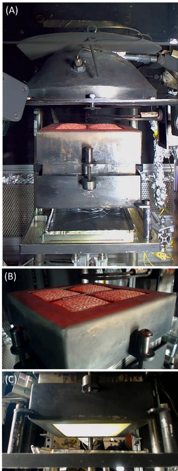
Figure 1. Pictures showing the setup used in the Cube test: A, wide view; B, top view, and; C, bottom view. A detailed description of Cube test components is reported elsewhere [27].
