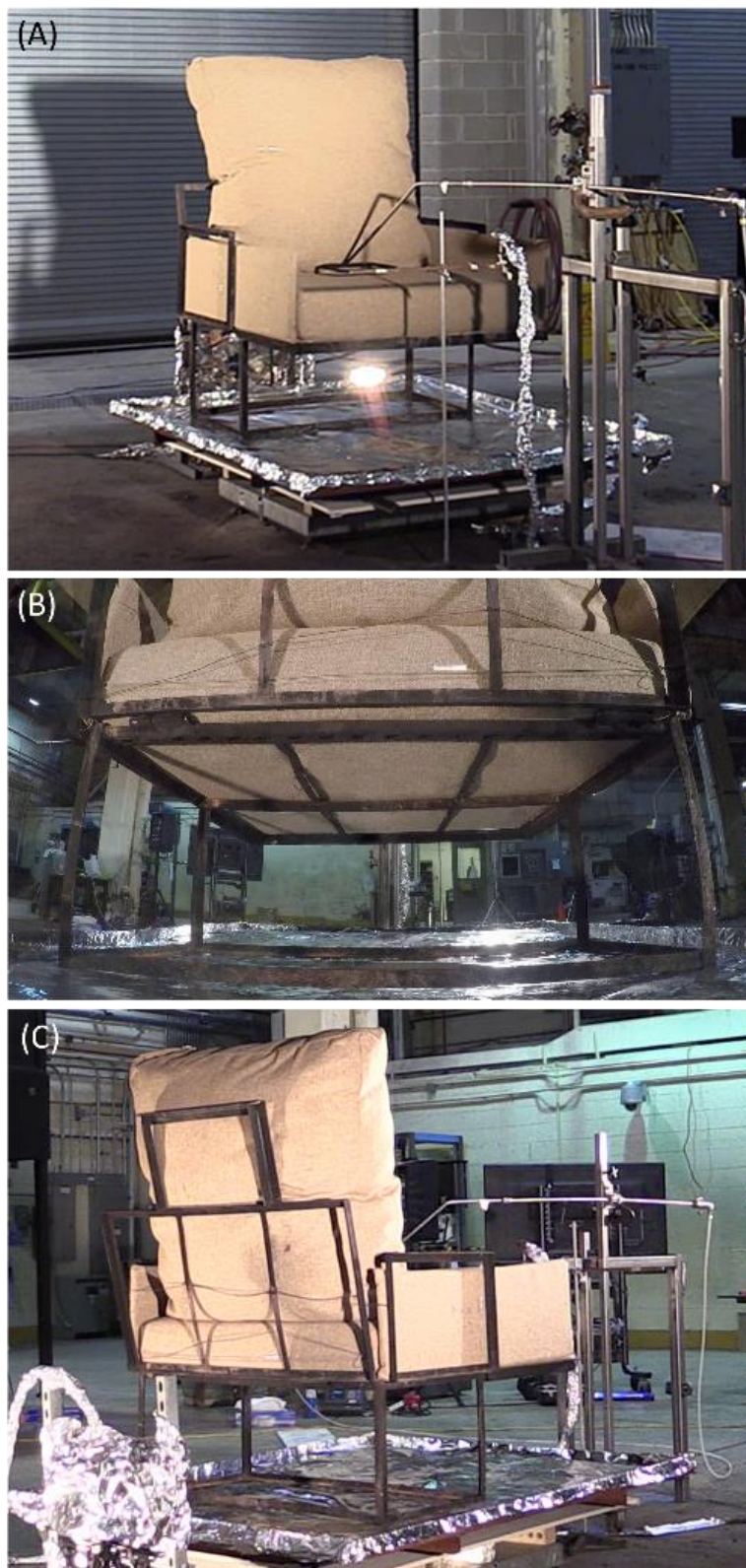
Figure 2. Pictures showing the setup used in the full-scale chair mock-ups: A, front view; B, bottom view, and; C, rear view.
