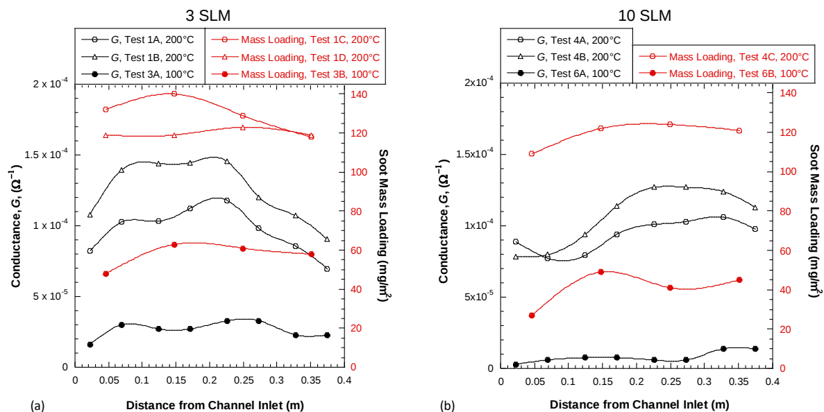
Fig. 21. Final conductance and gravimetric soot mass loading as a function of distance for vertical orientation at both \Delta T = 200^\circ\text{C} and 100^\circ\text{C} for (a) 3 SLM and (b) 10 SLM.
