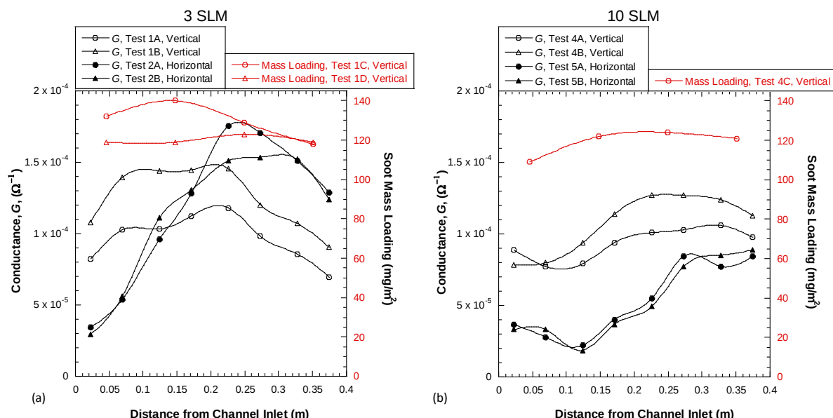
Fig. 20. Final sensor conductance and gravimetric soot mass loading as a function of distance for \Delta T = 200^\circ\text{C} at both vertical and horizontal conditions for (a) 3 SLM and (b) 10 SLM.
