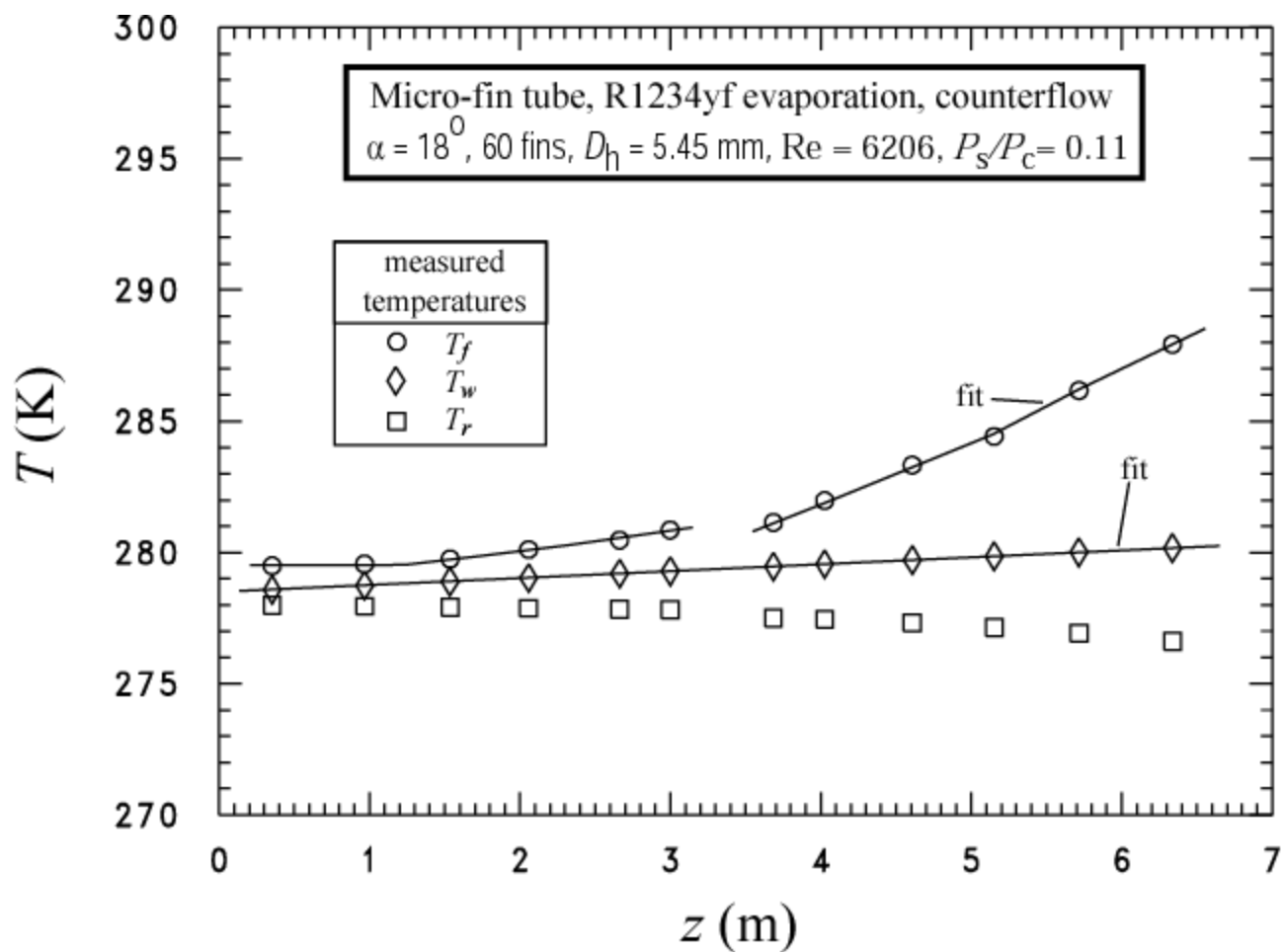
Figure 5. Counterflow temperature profiles for a R1234yf test
