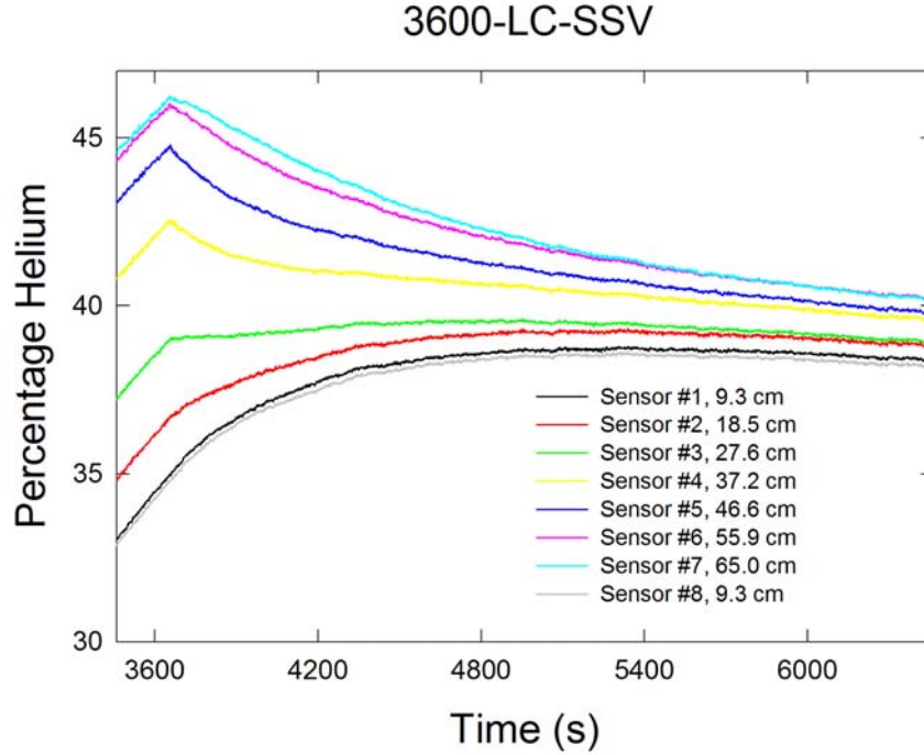
Figure 21. Helium volume percent measurements recorded at eight locations within the \frac{1}{4} -scale garage equipped with a single 2.4 \text{ cm} \times 2.4 \text{ cm} vent are shown for a period ranging from 200 s before to 2800 s after the flow was halted for a one hour helium release near the floor at the center of the garage.
