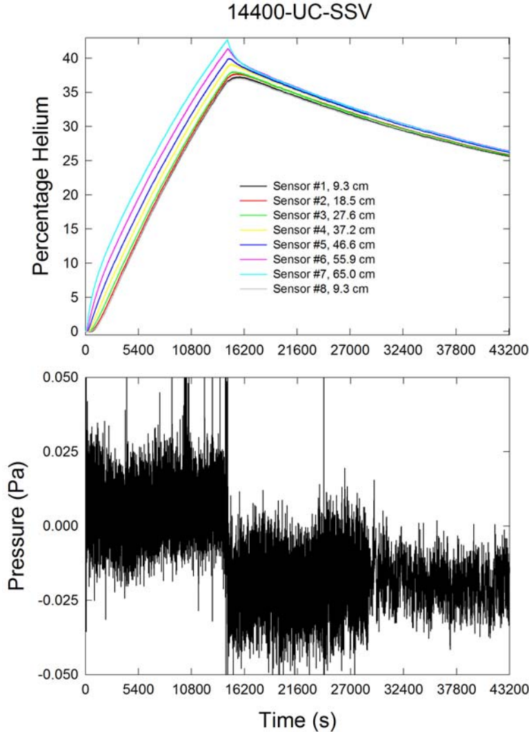
Figure 42. The upper plot shows helium volume percent as a function of time at eight locations for a four hour release of helium from the upper center position into the \frac{1}{4} -scale garage with a single centered 2.4 \text{ cm} \times 2.4 \text{ cm} opening in the front face. The lower plot shows the differential pressure across the face.
