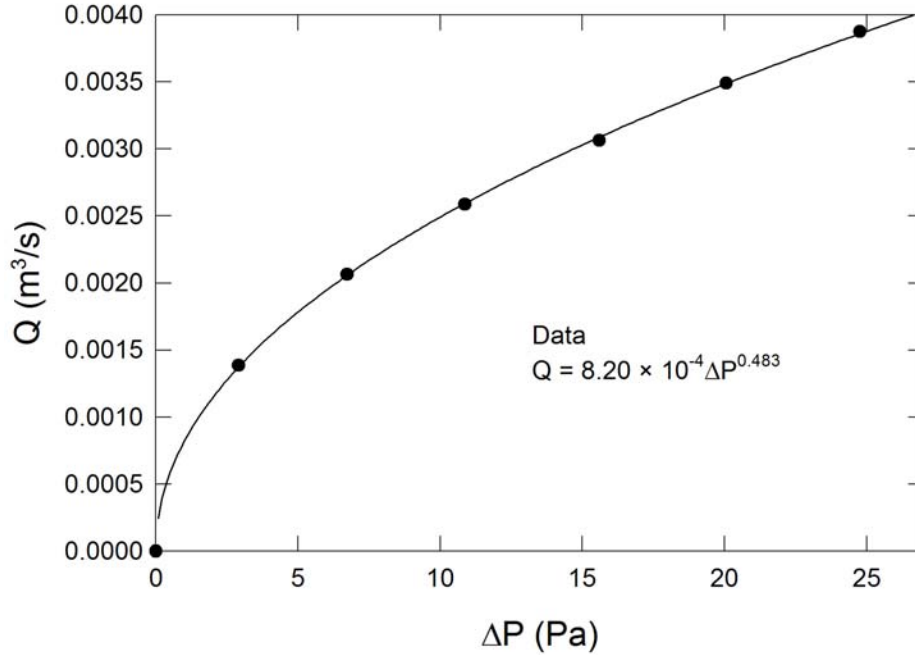
Figure 18. Values of air flow rate are plotted against the measured differential pressure for a fan tests for the reduced-scale garage with two 2.15 cm × 2.15 cm openings in the front wall. The solid line is the result of a non-linear least squares curve fit to Eq. (2).
