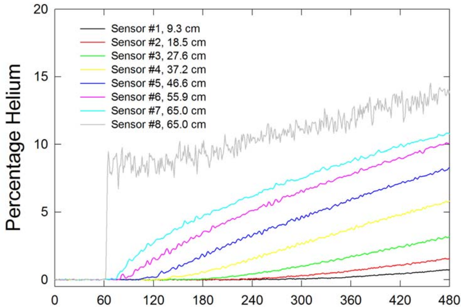
Figure 25. Helium volume percent measurements recorded at eight locations within the \frac{1}{4} -scale garage equipped with upper and lower 2.15 cm \times 2.15 cm vents are shown for the initial period of a one hour helium release near the floor at the center of the garage.
