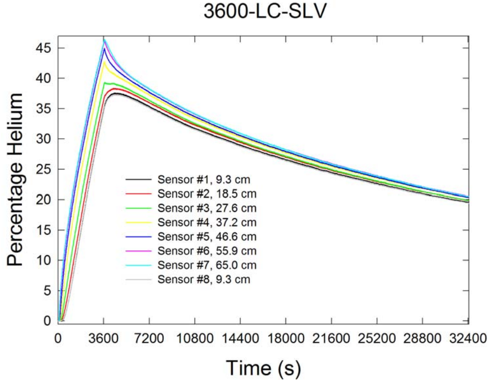
Figure 23. Helium volume percent measurements recorded at eight locations within the \frac{1}{4} -scale garage equipped with a single 3.05 cm \times 3.05 cm vent are shown for the initial period of a one hour helium release near the floor at the center of the garage.
