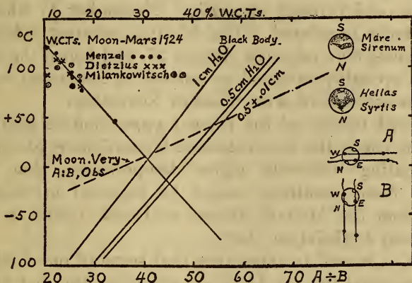
FIG. 1.—Planetary temperatures as derived from the ratio ( A+B ) of the spectral components of planetary radiation, and from the water-cell transmissions (W. C. Ts.). Also illustration of markings on the Martian surface and methods of setting the thermocouples on the planetary image
