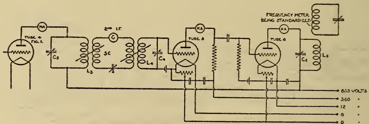
FIG. 2.—Extension of harmonic amplifier shown in Figure 1 to obtain frequencies to 4,000 kc
