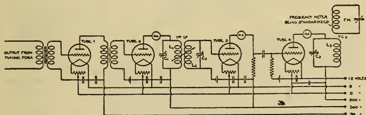
FIG. 1.—Circuit diagram of harmonic amplifier as used to obtain low frequencies (8–450 kc)
