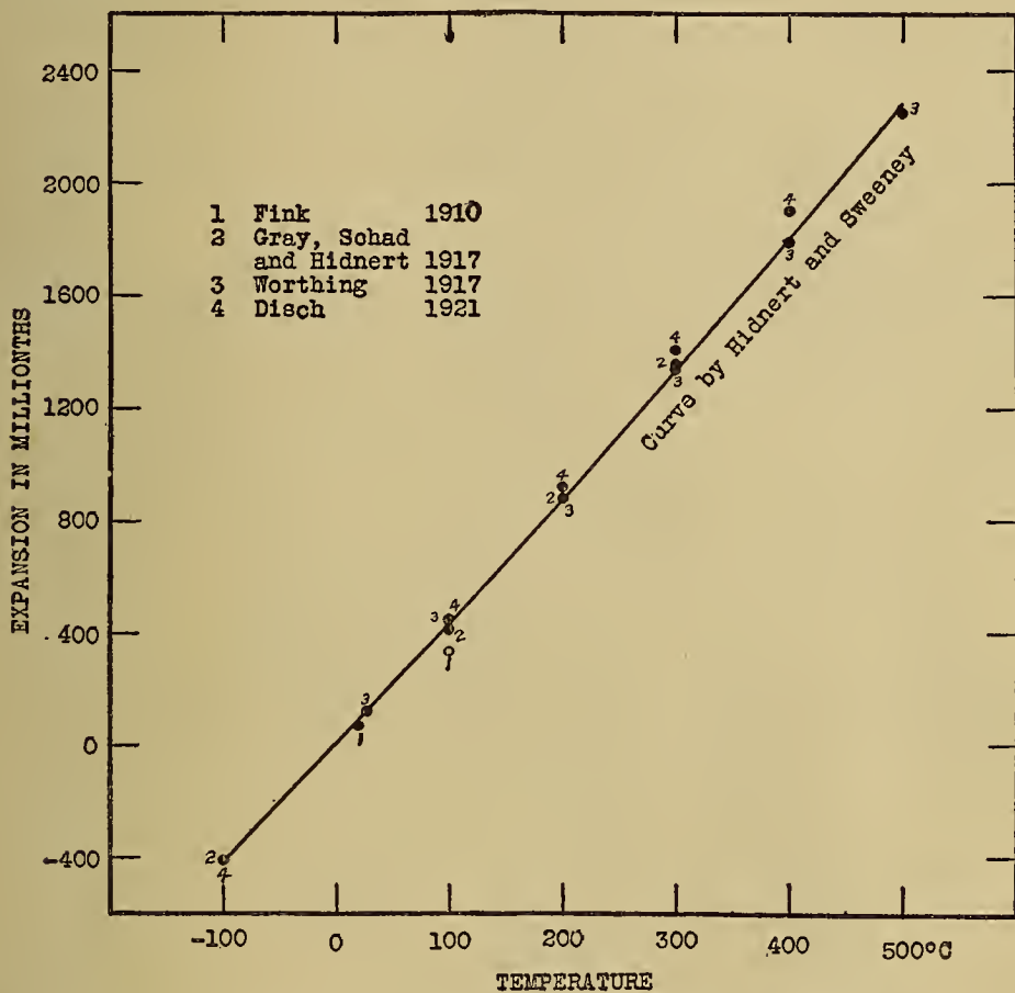
FIG. 2.—Comparison of expansion curve obtained in the present investigation on tungsten with data from previous observers
