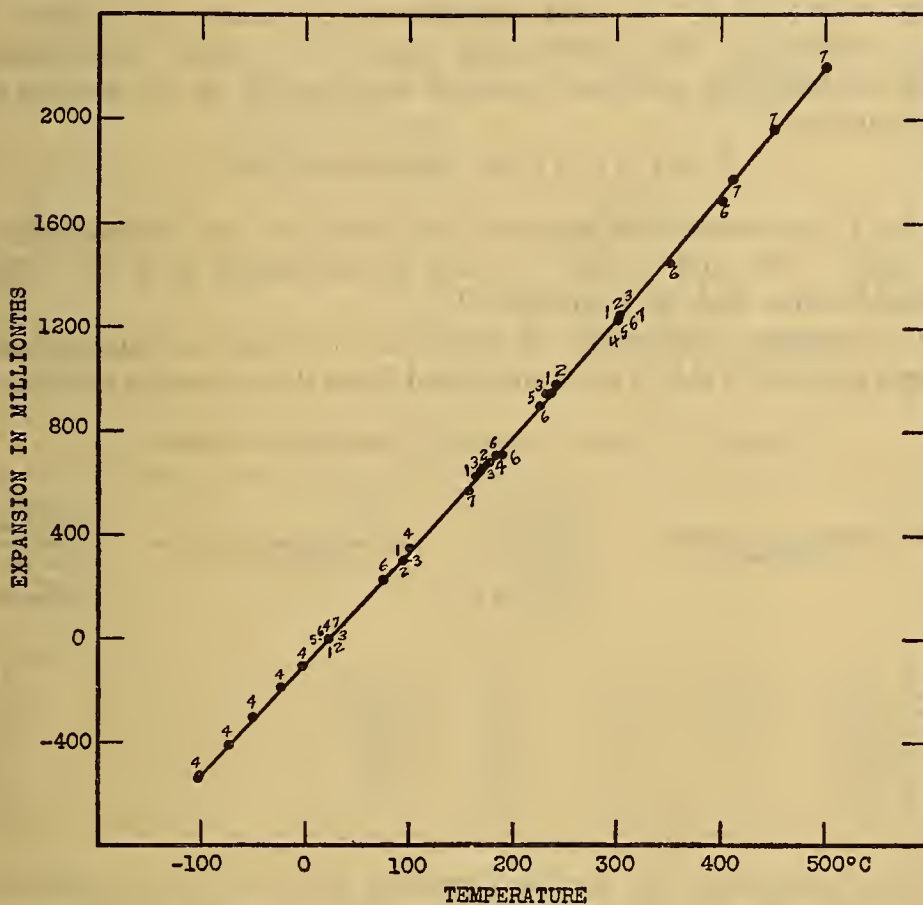
FIG. 1.—Linear expansion of tungsten (99.98 per cent)
