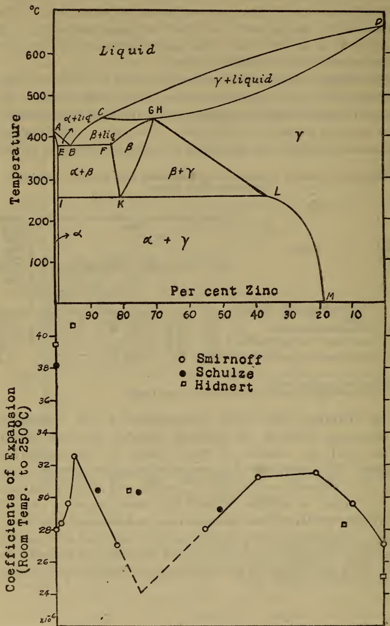
FIG. 16.—Comparison of coefficients of expansion of aluminum-zinc alloys and their relation to the equilibrium diagram
