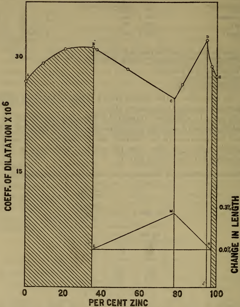
FIG. 1.—Average coefficients of expansion of aluminum-zinc alloys from 25 to 250° C., and the changes in length at the transformation temperature, 260 to 270° C. (Smirnoff)
