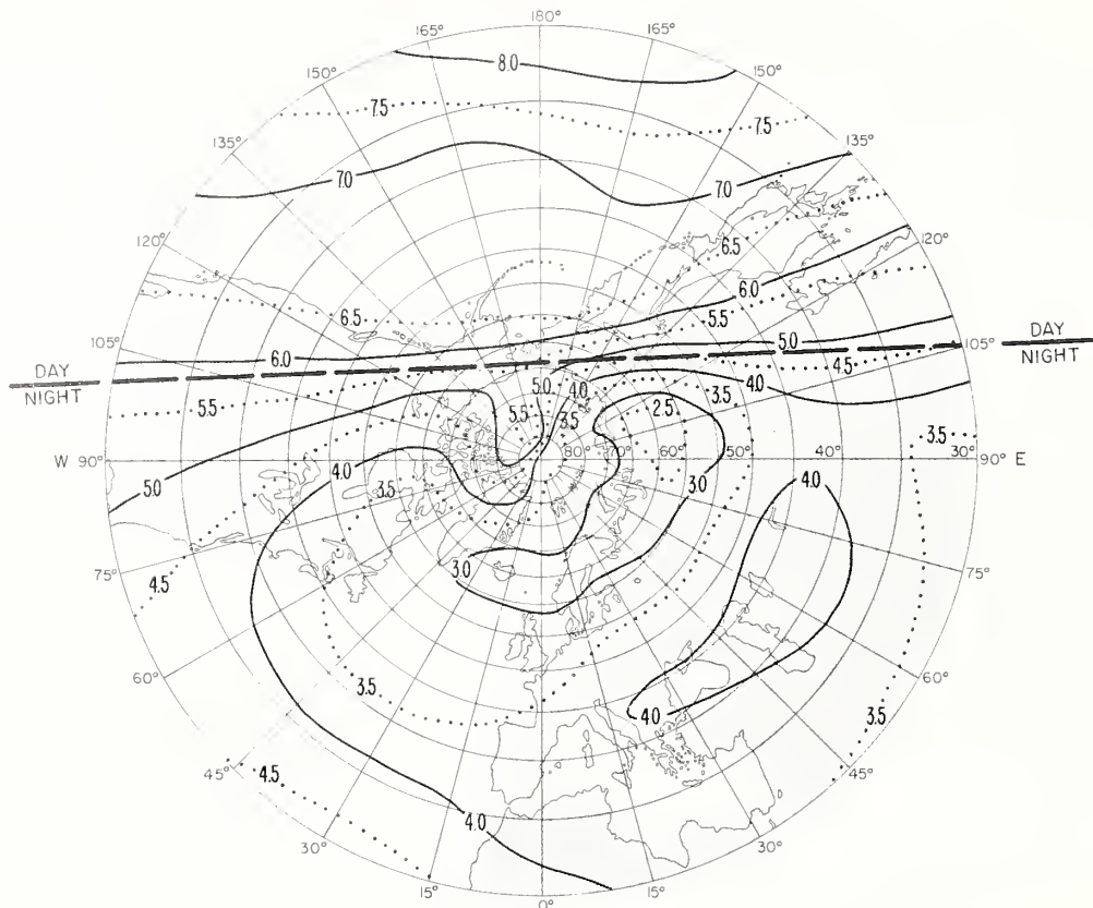
FIG 13A. PREDICTED MEDIAN MUF(ZERO)F2 (Mc/s)
