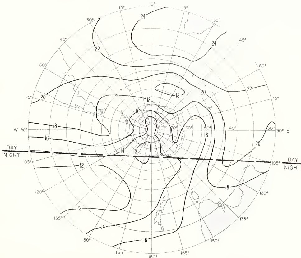
FIG. I6B. PREDICTED MEDIAN MUF(4000)F2 (Mc/s)
