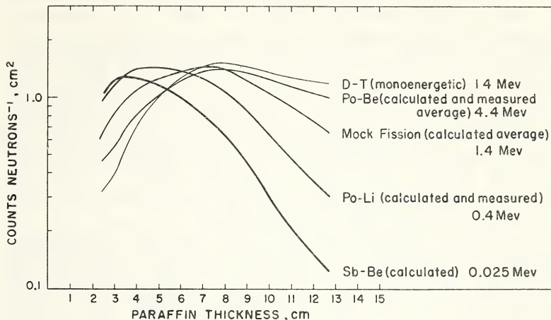
FIGURE 23. Counting rate for a \text{BF}_3 proportional counter covered by various thicknesses of paraffin for five different neutron sources, corrected to an isotropic flux distribution (Hess and Smith, 1958).
