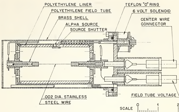
FIGURE 16. Drawing for the absolute fast neutron dosimeter.
