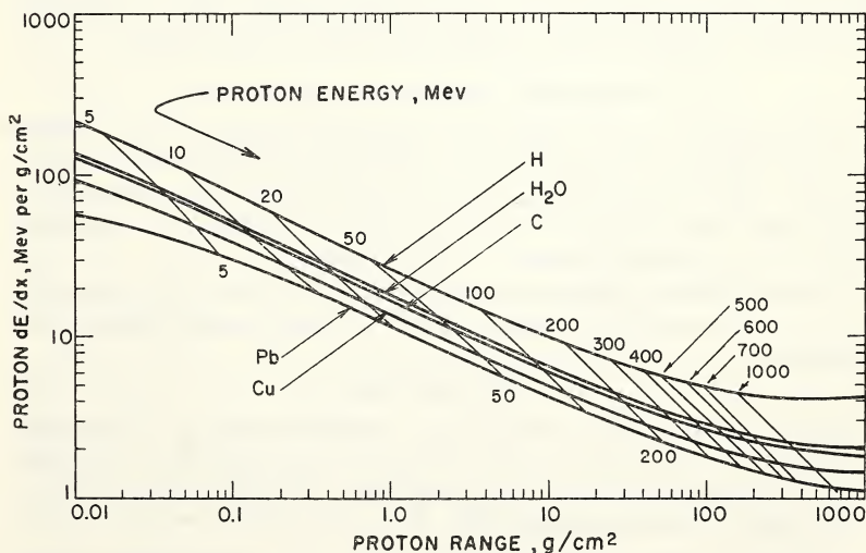
FIGURE 13. Energy loss for protons in Mev per g per \text{cm}^2 as a function of residual range in various materials with the constant energy lines indicated (Rich and Madey, 1954).
