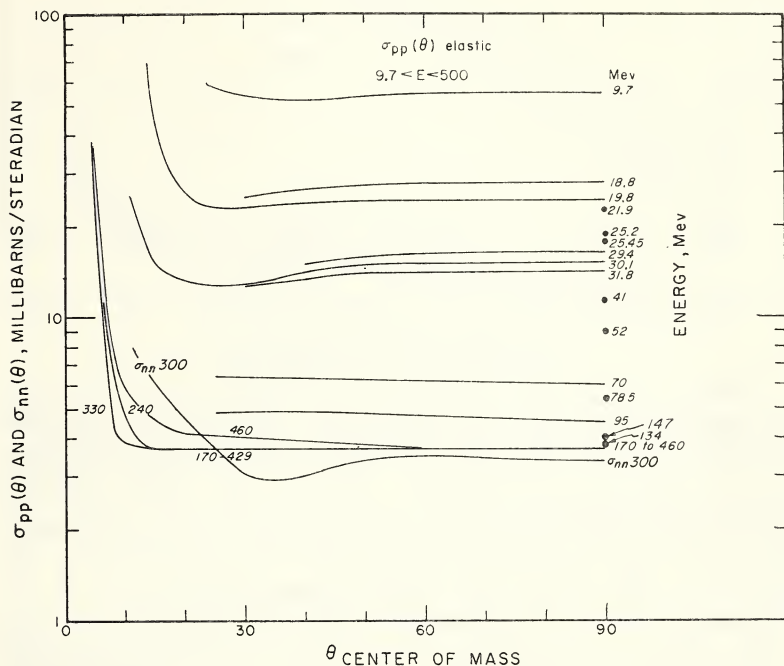
FIGURE 10. Cross sections for p - p and n - n scattering as a function of center-of-mass angle in millibarns per steradian as a function of energy from 10 Mev to 460 Mev for p - p and at 300 Mev for n - n (Hess, 1958).
