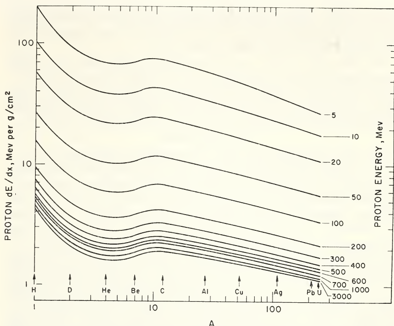
FIGURE 12. Energy loss for protons in Mev per g per \text{cm}^2 as a function of attenuating material for energies from 5 Mev to 3,000 Mev (Rich and Madey, 1954).
