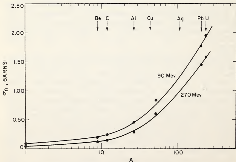
FIGURE 6. Nonelastic neutron cross sections for elements heavier than hydrogen.
