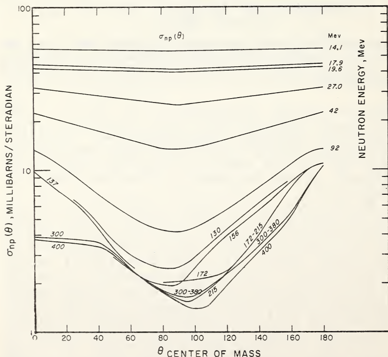
FIGURE 9. Cross sections for n - p scattering as a function of center-of-mass neutron angle in millibarns per steradian as a function of energy from 14 Mev to 400 Mev (Hess, 1958).
