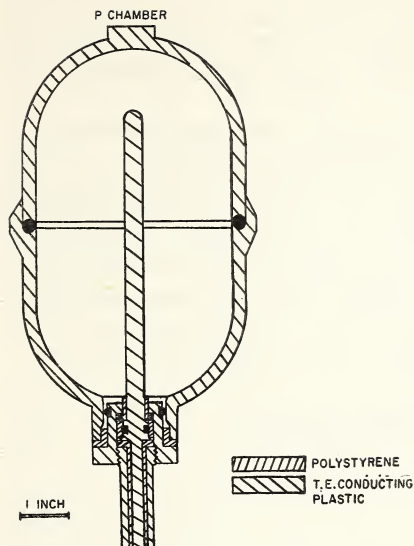
FIGURE 14. Schematic of a large size (high sensitivity) tissue equivalent ionization chamber.
