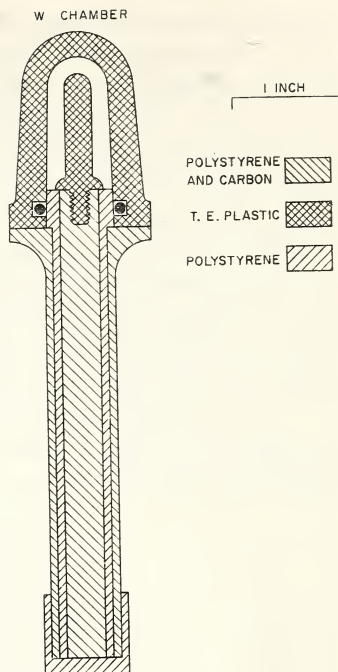
FIGURE 15. Schematic of a small size (low sensitivity) tissue equivalent ionization chamber.
