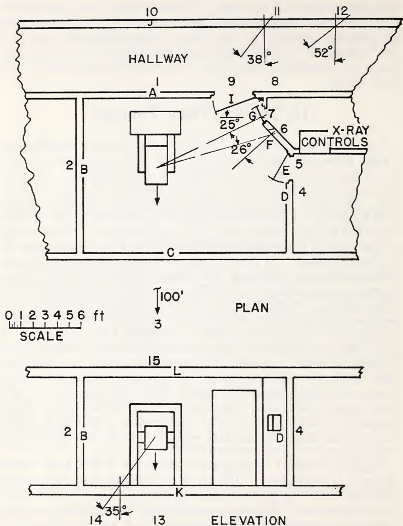
FIGURE 6. Plan and elevation views of sample 250-kvp therapy installation.
