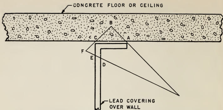
FIGURE 1. Example of wall joint (for section 4.7)
