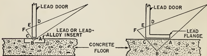
FIGURE 2. Example of door baffle (for section 4.9)
