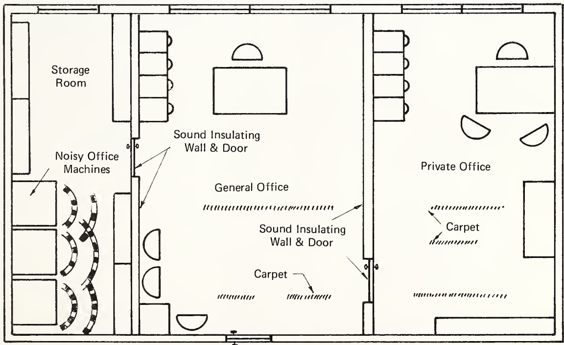
Fig. 8-2. A WELL-PLANNED OFFICE COMPLEX WHICH AFFORDS PRIVACY AND A QUIET ENVIRONMENT
