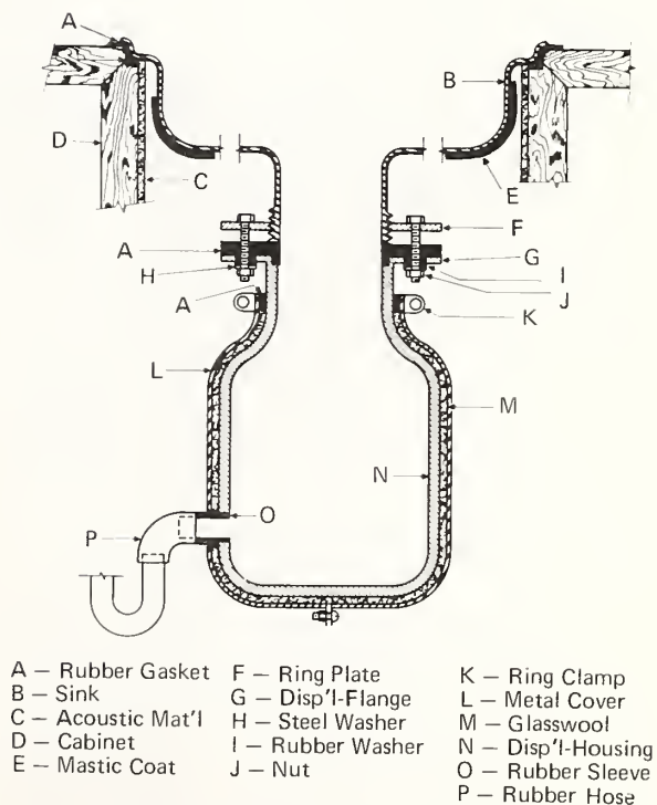
Fig. 4-8. DESIGN AND INSTALLATION OF A GARBAGE DISPOSER FOR QUIET OPERATION
