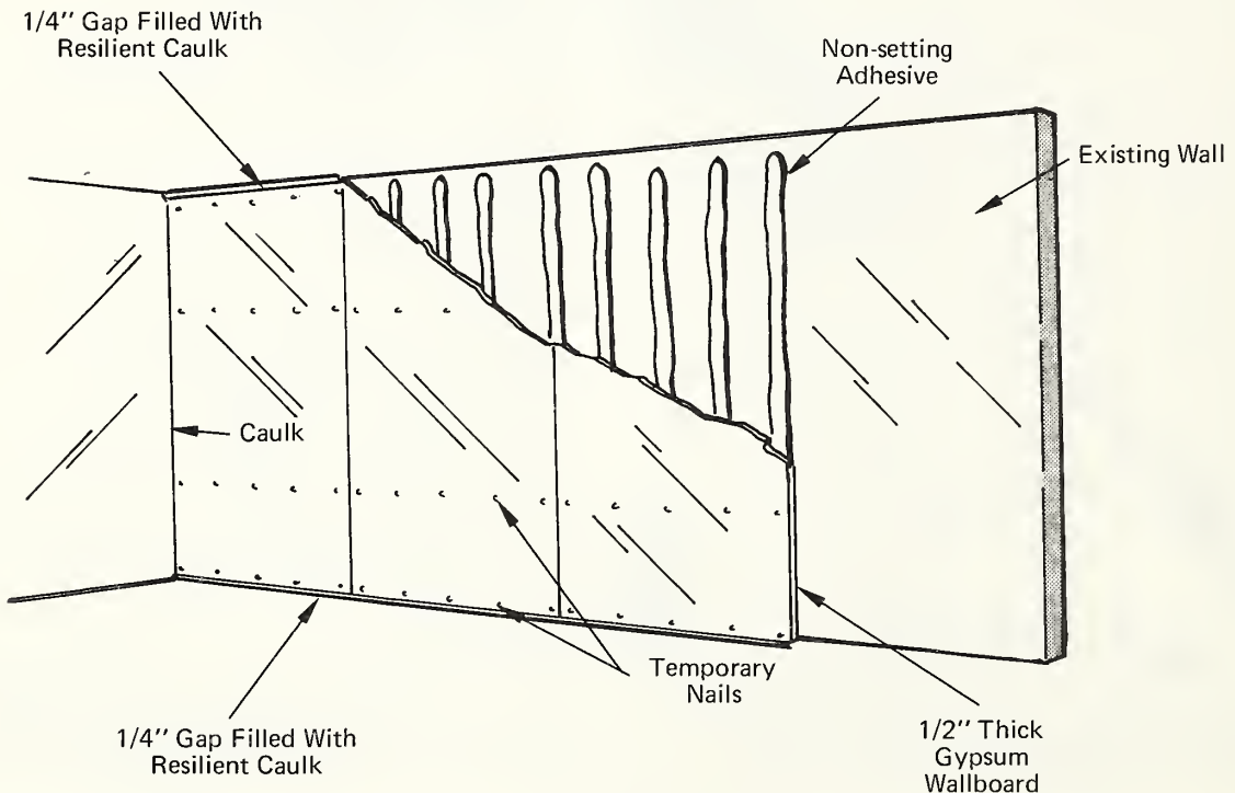
Fig. 4-13. IMPROVING THE SOUND INSULATION OF AN EXISTING WALL
