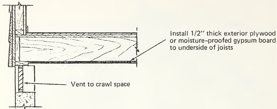
A—Added Floor Construction
