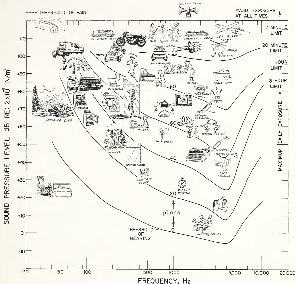
Fig. 1-1. COMMON SOUND SOURCES PLOTTED AT THEIR DOMINANT FREQUENCIES AND LEVELS AS TYPICALLY HEARD BY THE OBSERVER
