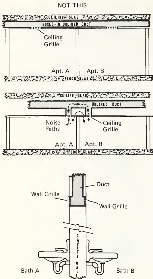
Fig. 4-24. METHODS OF CONTROLLING CROSS TALK AND THE TRANSMISSION OF FLANKING NOISE IN DUCTS
