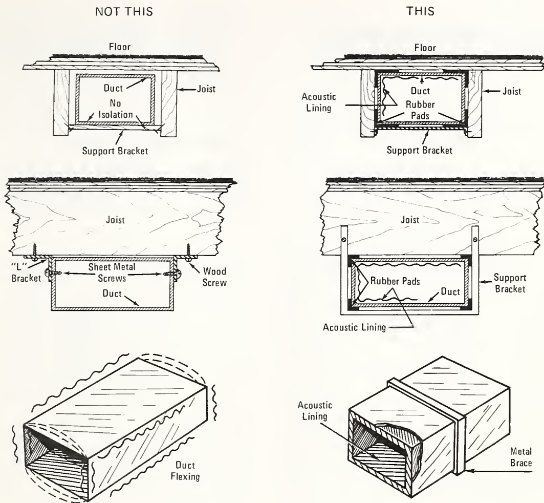
Fig. 4-23. METHODS OF REDUCING NOISE DUE TO AIR FLOW AND VIBRATION IN DUCT SYSTEMS
