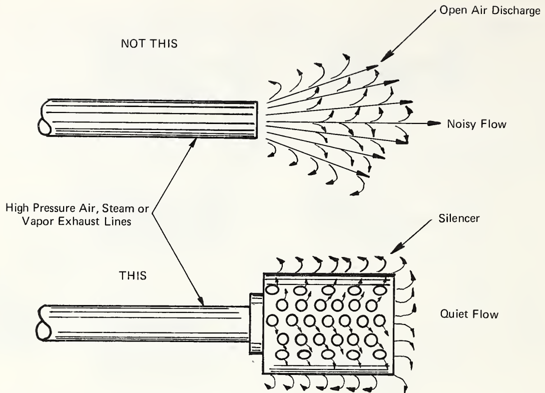
Fig. 3-17. SILENCER FOR HIGH PRESSURE EXHAUST LINE
