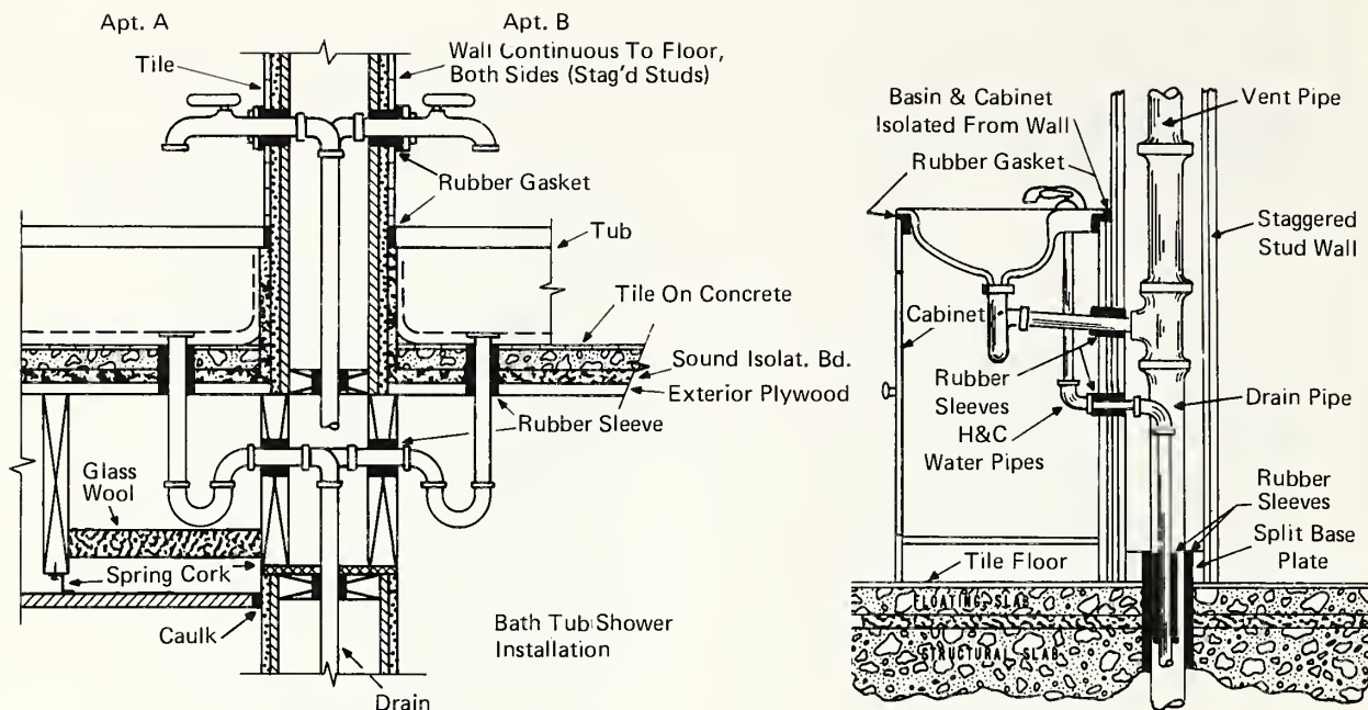
Fig. 4-27. PROPER INSTALLATION OF BATH TUBS AND WASH BASINS
