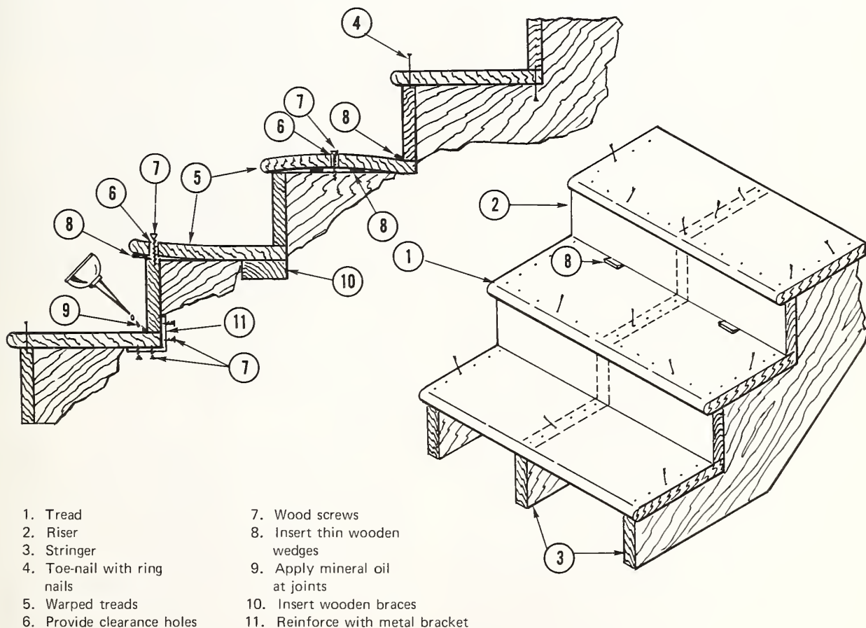
Fig. 4-20. TECHNIQUES FOR THE CONTROL OF STAIR SQUEAKING
