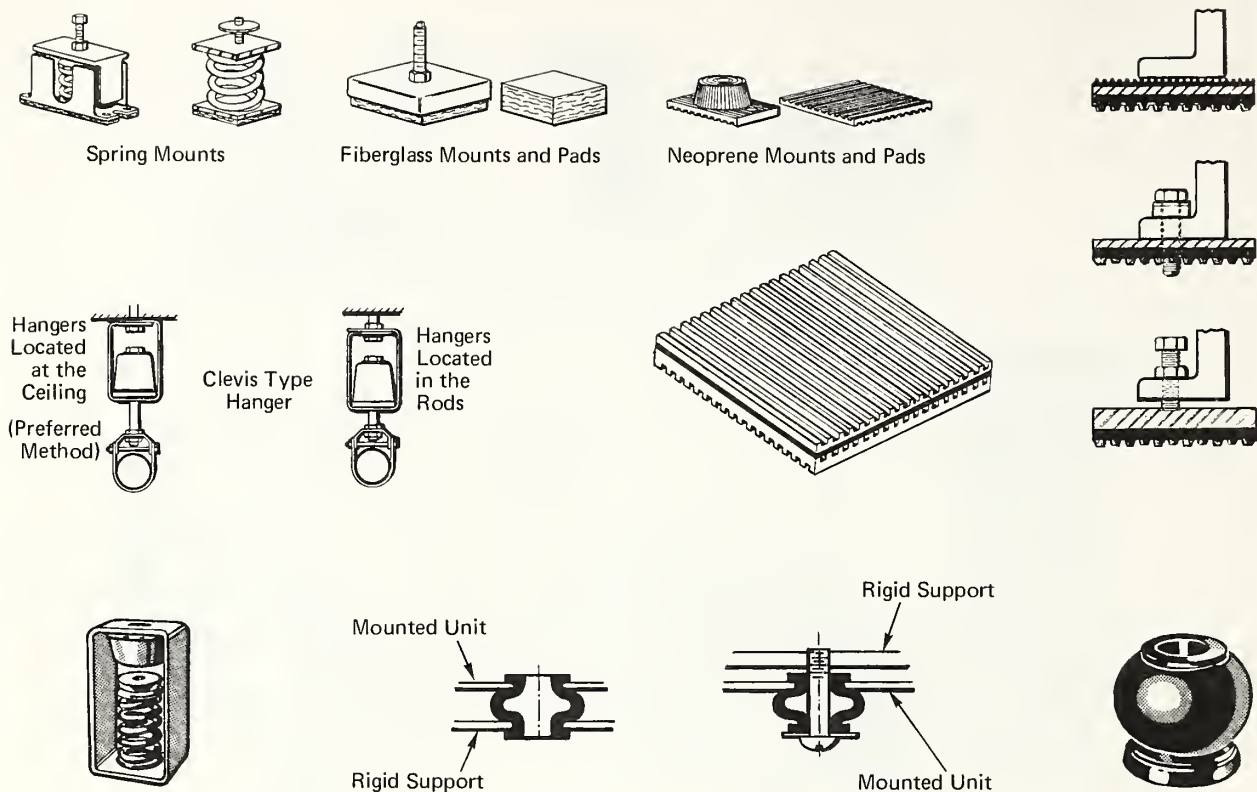
Fig. 3-19. VARIOUS TYPES OF VIBRATION ISOLATORS
