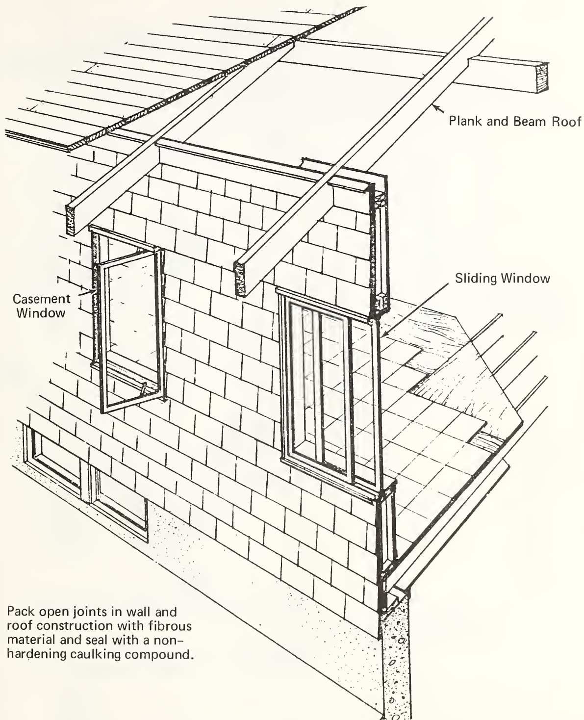
Fig. 5-8. HOUSE WITH A BASEMENT AND PLANK AND BEAM ROOF
