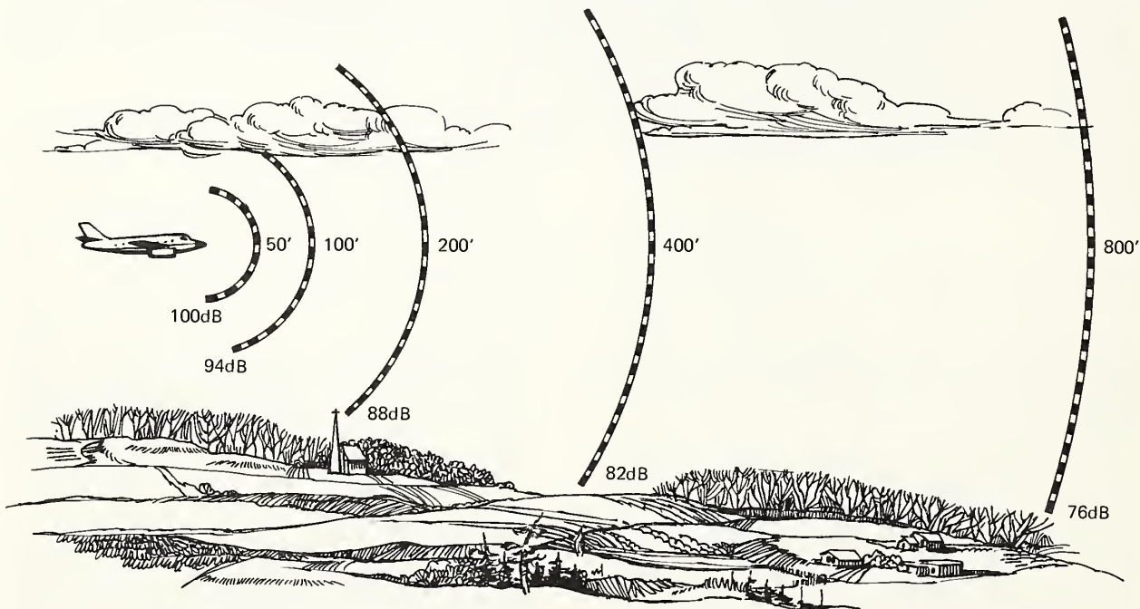
Fig. 3-14a. REDUCTION IN NOISE LEVEL WITH DISTANCE FROM A POINT SOURCE
