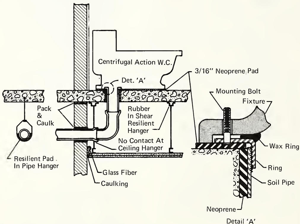
Fig. 4-28. PROPER INSTALLATION OF A TOILET FOR QUIET OPERATION
