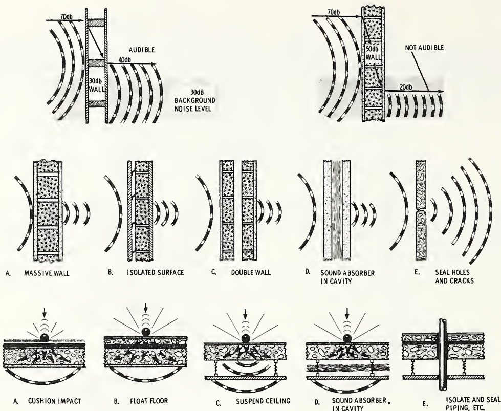
Fig. 4-5. METHODS OF CONTROLLING AIRBORNE AND IMPACT SOUND TRANSMISSION THROUGH WALLS AND FLOORS
