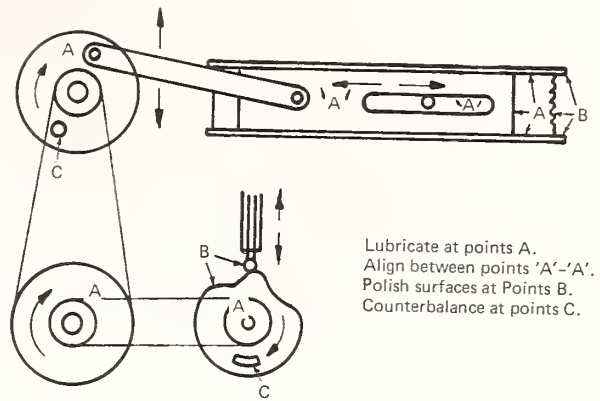
Fig. 3-4. REDUCING FRICTION OF ROTATING AND SLIDING PARTS TO DECREASE NOISE RADIATION
