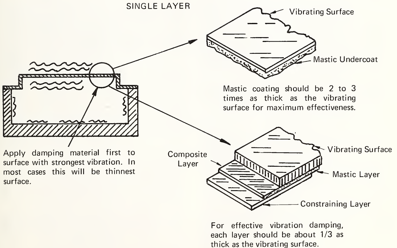
Fig. 3-9. REDUCING VIBRATION WITH DAMPING MATERIALS
