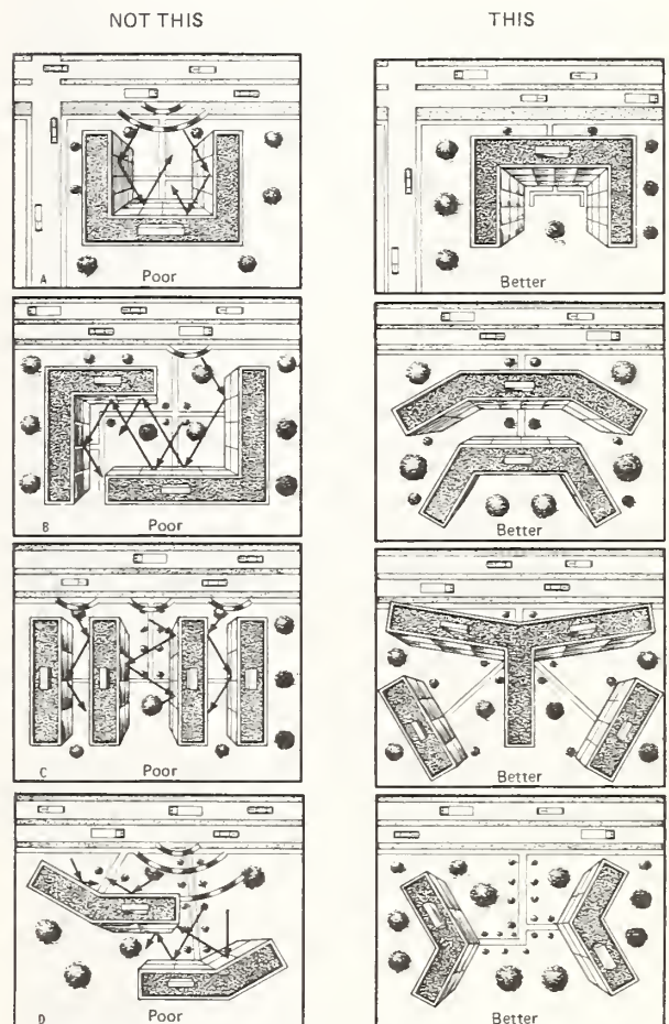
Fig. 6-4. ORIENTATION OF APARTMENT BUILDINGS FOR OPTIMUM ACOUSTICAL SHIELDING
