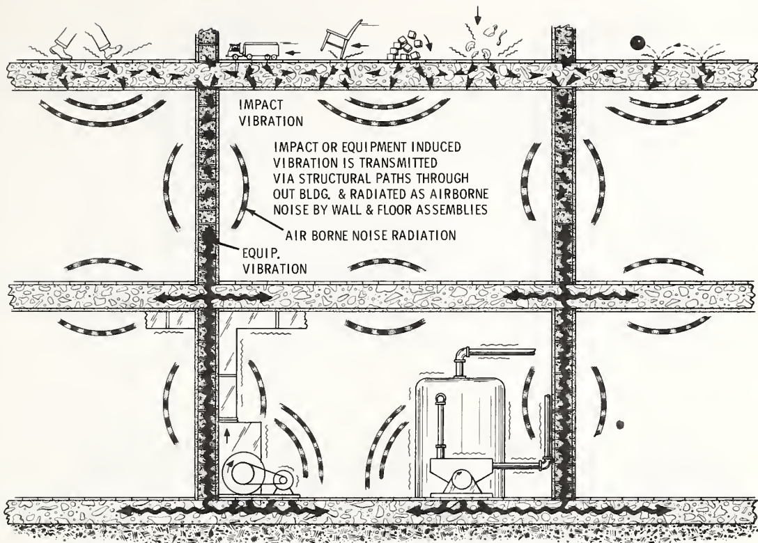
Fig. 4-4. COMMON STRUCTURE-BORNE NOISE AND VIBRATION PATHS IN BUILDINGS
