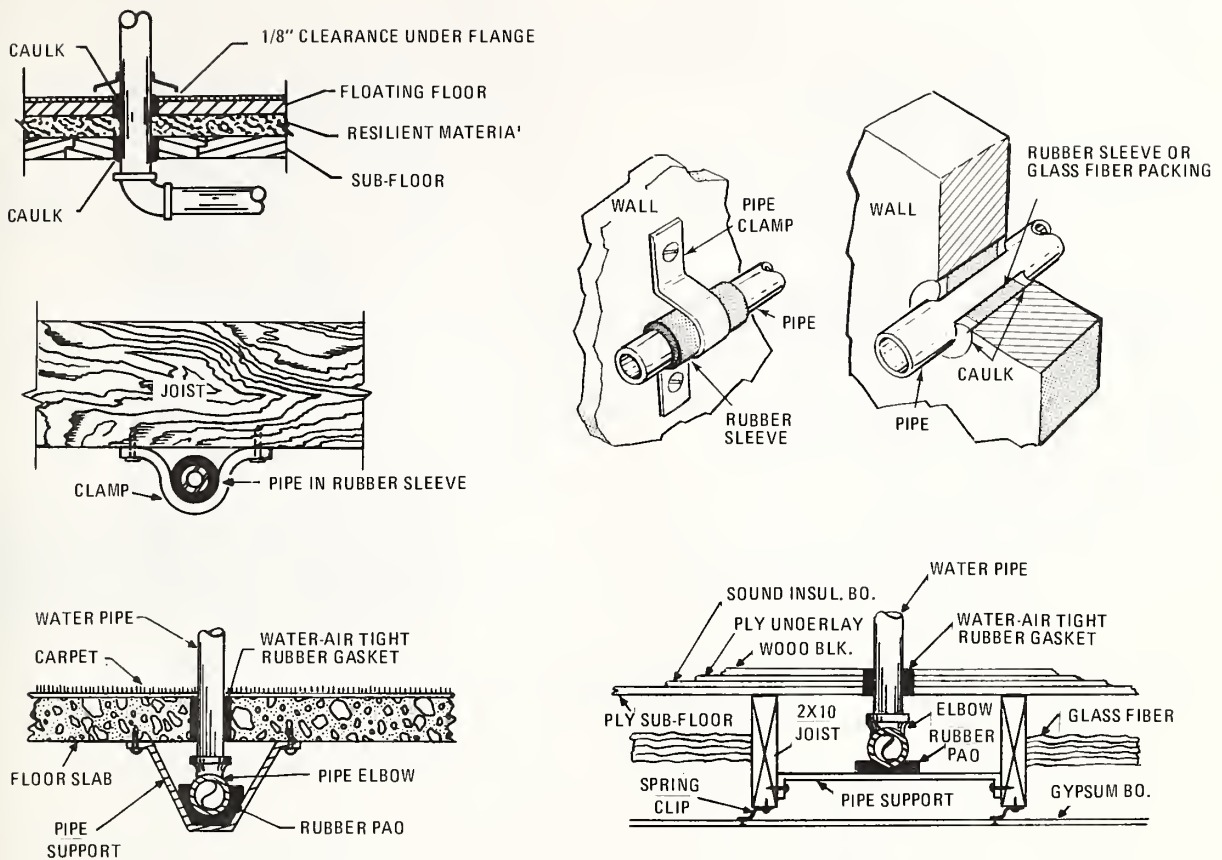
Fig. 4-26. METHODS OF INSTALLING PIPES FOR QUIET OPERATION
