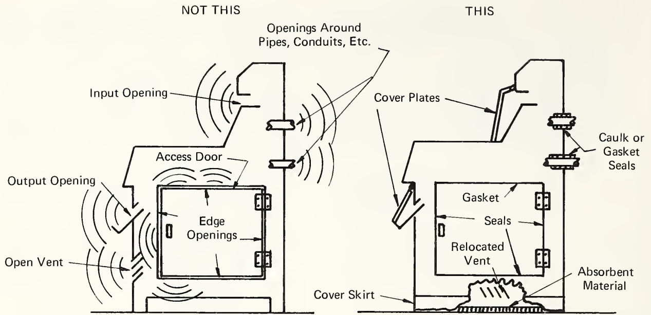
Fig. 3-10. TECHNIQUES FOR REDUCING THE RADIATION OF NOISE FROM OPENINGS IN A MACHINE
