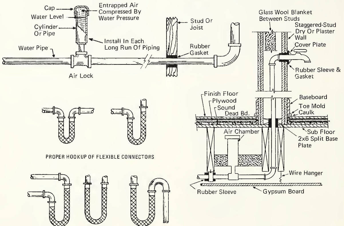
Fig. 4-25. TECHNIQUES FOR CONTROLLING NOISE IN PLUMBING SYSTEMS
