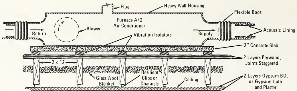
ATTIC INSTALLATION
