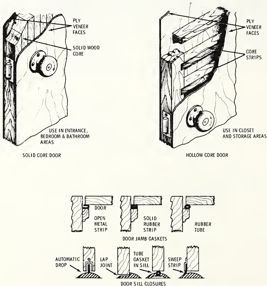
Fig. 4-7. PROPER INSTALLATION OF SOUND INSULATING DOORS
