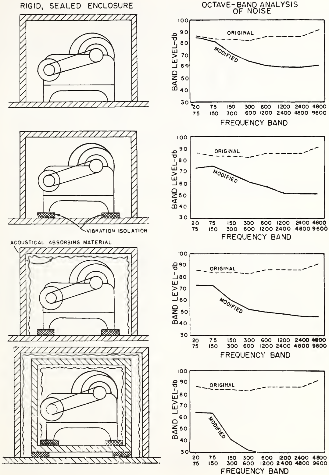
Fig. 3-20 EFFECTIVENESS OF VARIOUS NOISE REDUCTION TECHNIQUES
