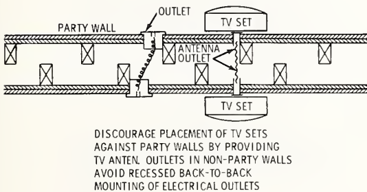
Fig. 4-15. PROPER INSTALLATION OF CABINETS AND ELECTRICAL OUTLETS IN WALLS
