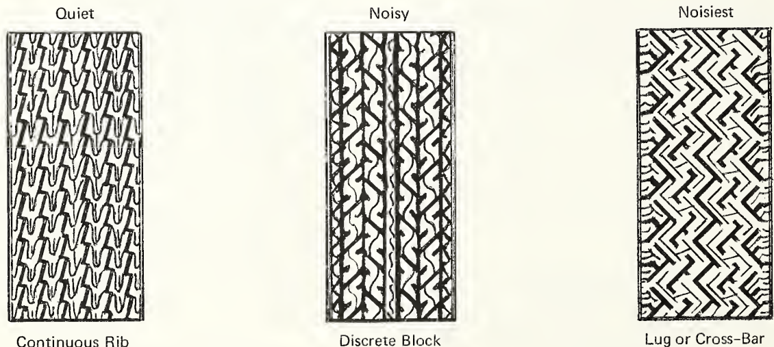
Fig. 9-1. BASIC TIRE TREAD DESIGNS IN ORDER OF RELATIVE NOISINESS
