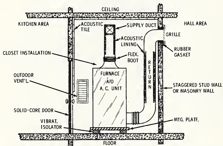
RECOMMENDED DESIGN OF CLOSET AND INSTALLATION OF FURNACE UNIT
