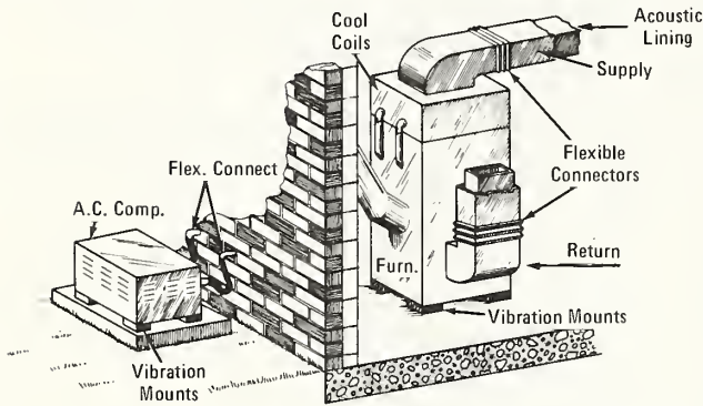
BASEMENT INSTALLATION
