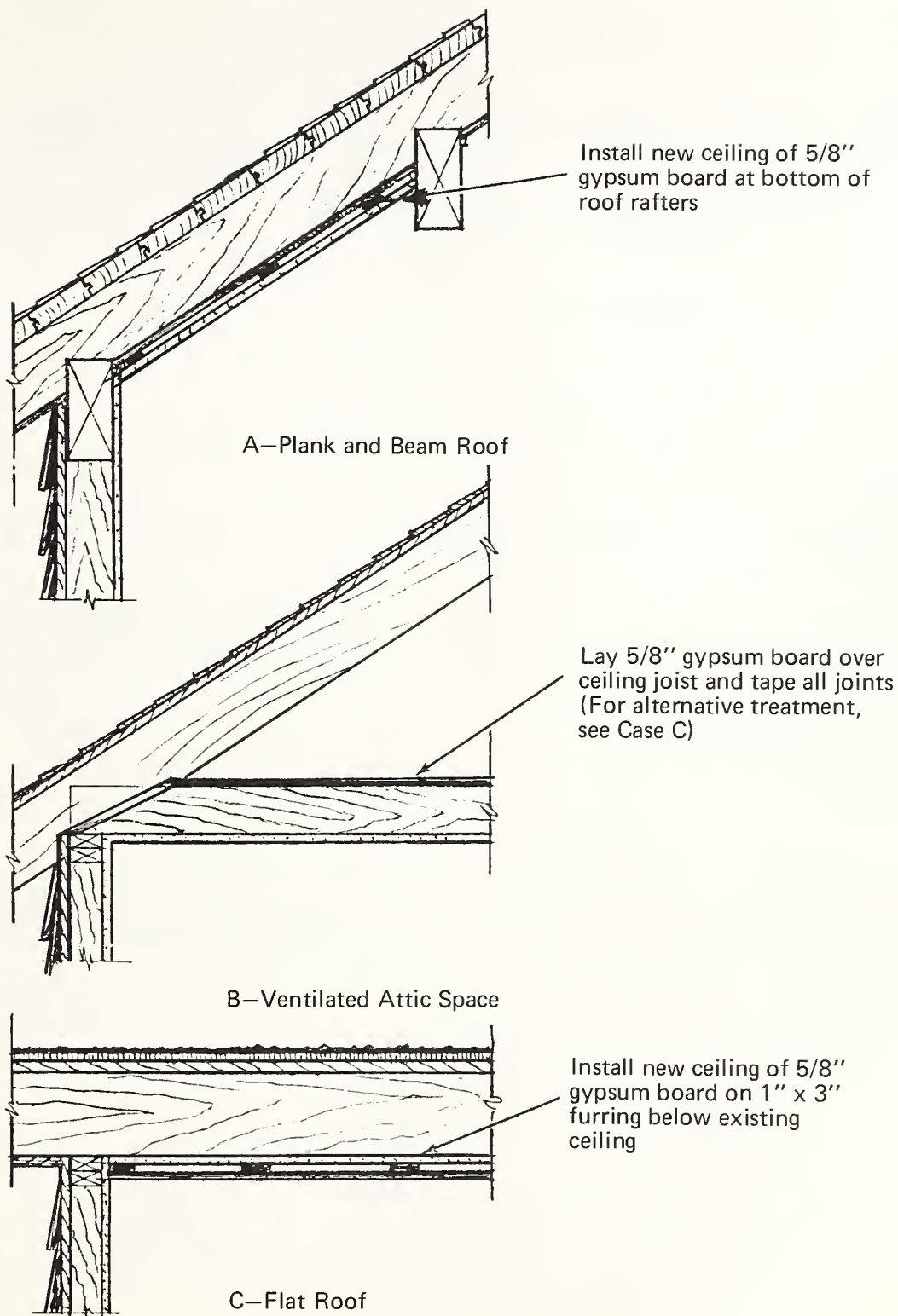
Fig. 5-10. ROOF AND CEILING MODIFICATIONS
