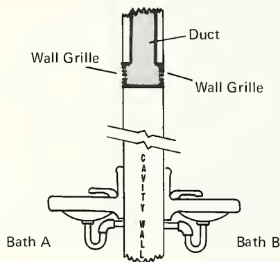
Fig. 4-24. METHODS OF CONTROLLING CROSS TALK AND THE TRANSMISSION OF FLANKING NOISE IN DUCTS
