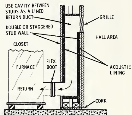
RECOMMENDED DESIGN OF CLOSET AND INSTALLATION OF FURNACE UNIT
