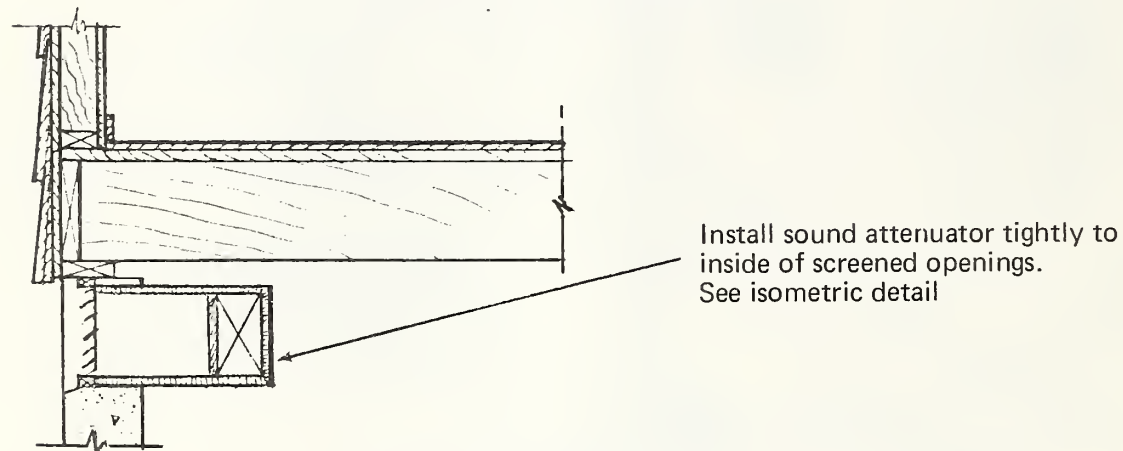
B—Vent Attenuators
