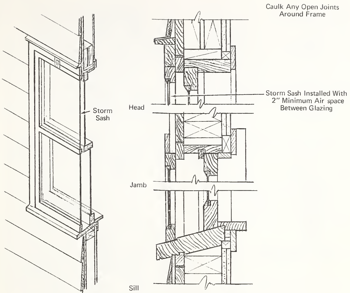
Fig. 5-1. DETAILS OF A DOUBLE-HUNG WINDOW WITH A STORM SASH
