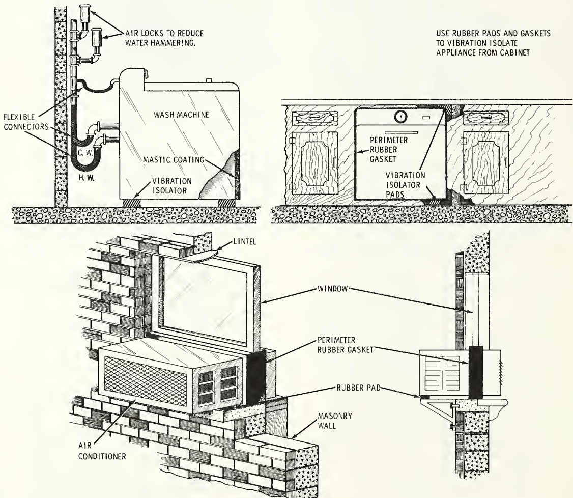
Fig. 4-10. PROPER INSTALLATION OF APPLIANCES FOR QUIET OPERATION
