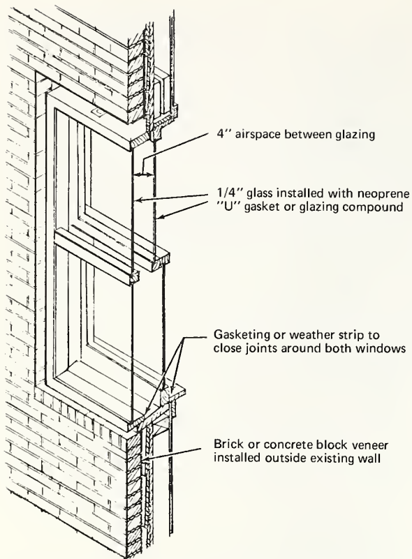
Fig. 5-2. INSTALLATION OF BRICK VENEER AND DOUBLE 1/4-INCH WINDOW GLAZING
