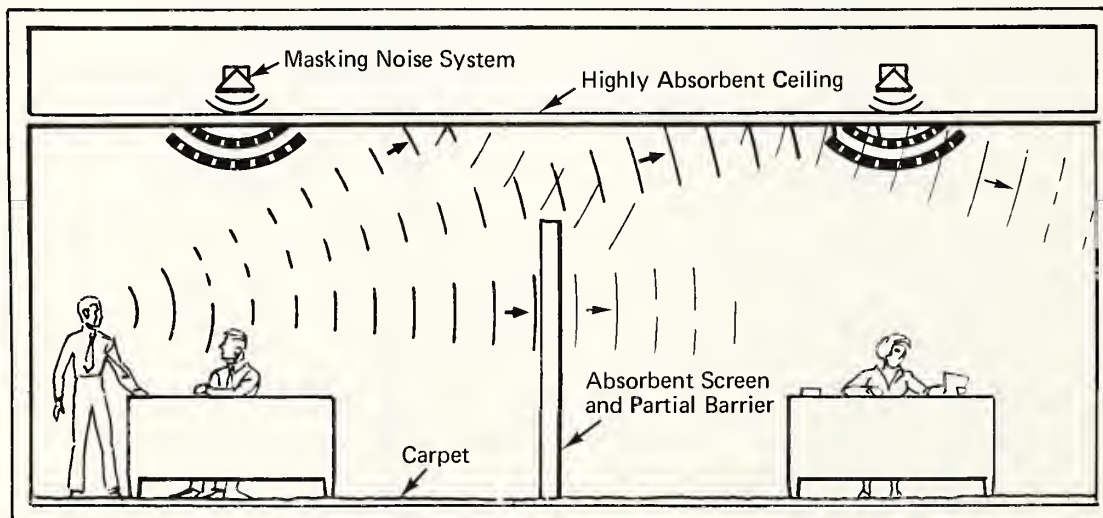
Fig. 8-3. FACTORS CONTROLLING SPEECH PRIVACY IN OPEN-PLAN OFFICES: ACOUSTICAL CEILING, SCREEN AND CARPET MINIMIZE SOUND REFLECTION. PARTIAL BARRIER ATTENUATES AND DEFLECTS DIRECT SOUND. MASKING NOISE RENDERS INTRUDING SPEECH UNINTELLIGIBLE.
