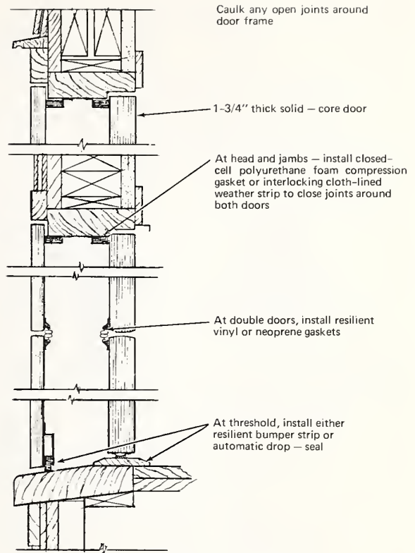
Fig. 5-5. DETAILS OF DOOR MODIFICATIONS
