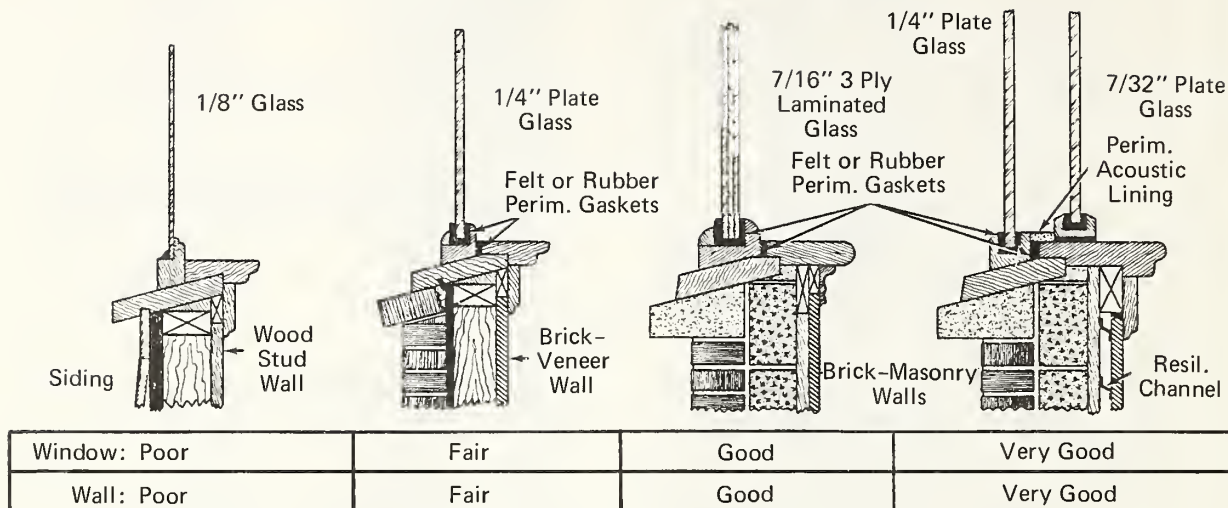
Fig. 5-6. SOUND INSULATION EFFECTIVENESS OF VARIOUS WINDOW-WALL ASSEMBLIES
