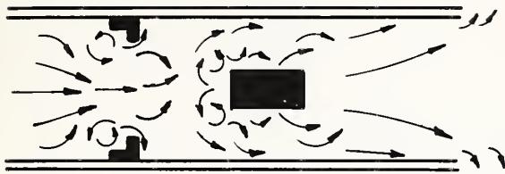
Turbulence Caused by Rectangular Devices
