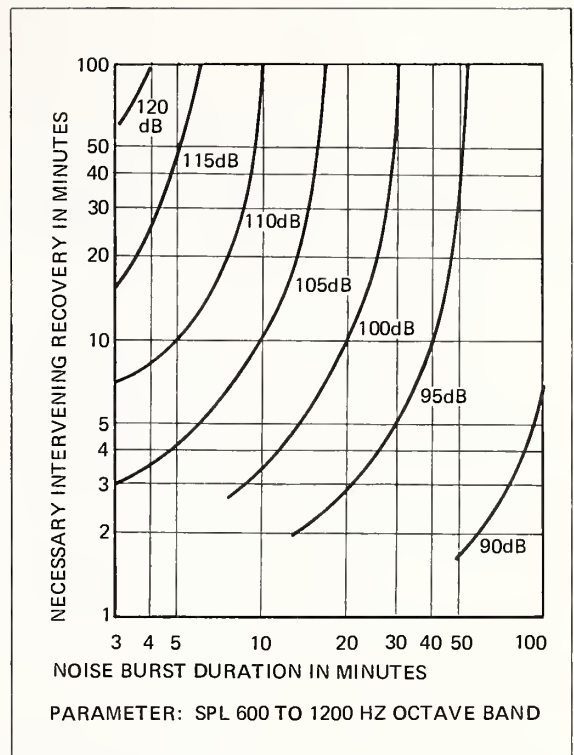
Fig. 2-3. RECOVERY TIMES AND MAXIMUM EXPOSURE ALLOWED TO REMAIN BELOW PROPOSED DAMAGE-RISK LIMITS (WARD, 1966)
