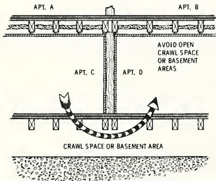
Fig. 4-16. METHODS OF CONTROLLING FLANKING SOUND TRANSMISSION PATHS
