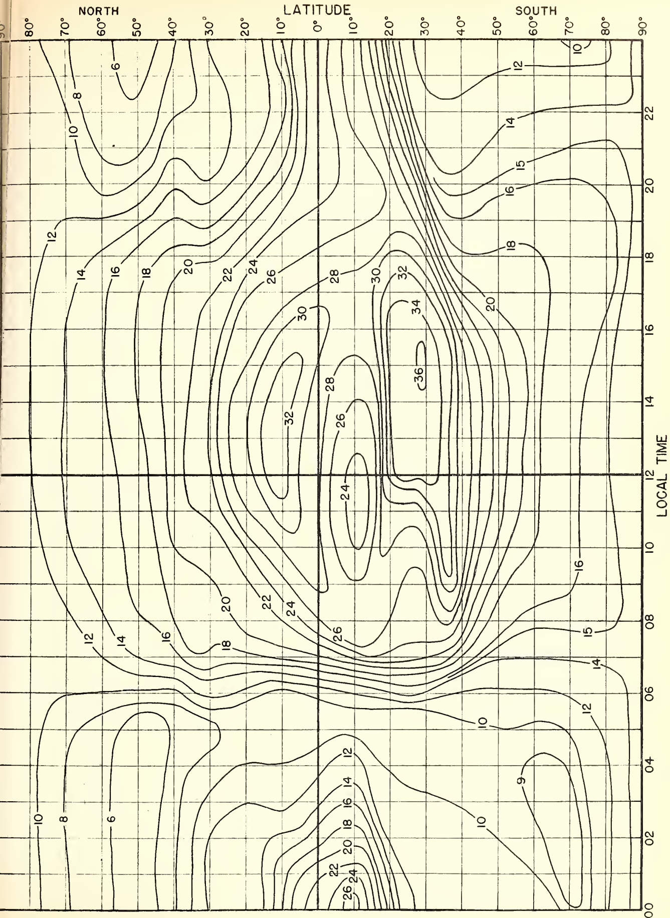
Fig.6. F 2 4000-MUF, IN Mc, W ZONE, PREDICTED FOR MARCH 1945.
