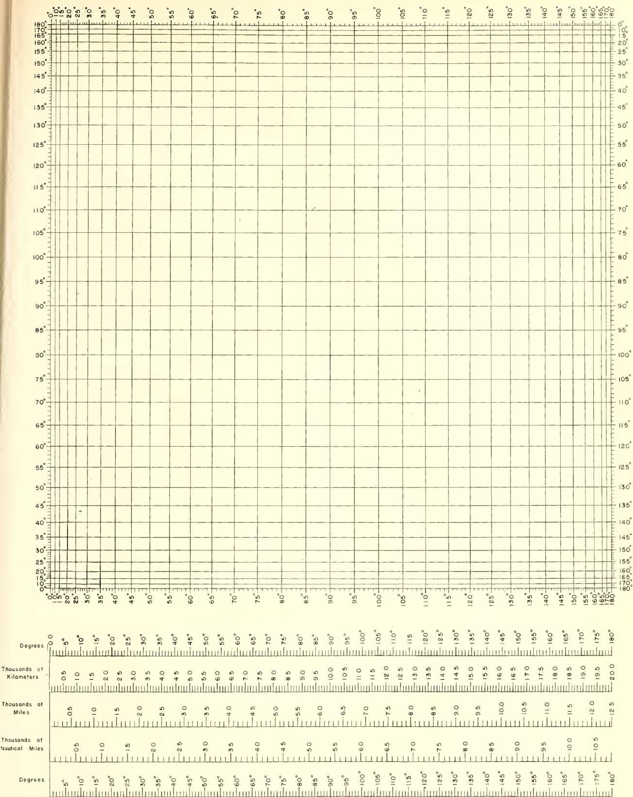
Fig 4. NOMOGRAM (AFTER D'OCAGNE) FOR OBTAINING GREAT-CIRCLE DISTANCES, BEARINGS, LATITUDE AND LONGITUDE OF TRANSMISSION CONTROL POINTS, SOLAR ZENITH ANGLES. CONVERSION SCALE FOR VARIOUS DISTANCE UNITS.
