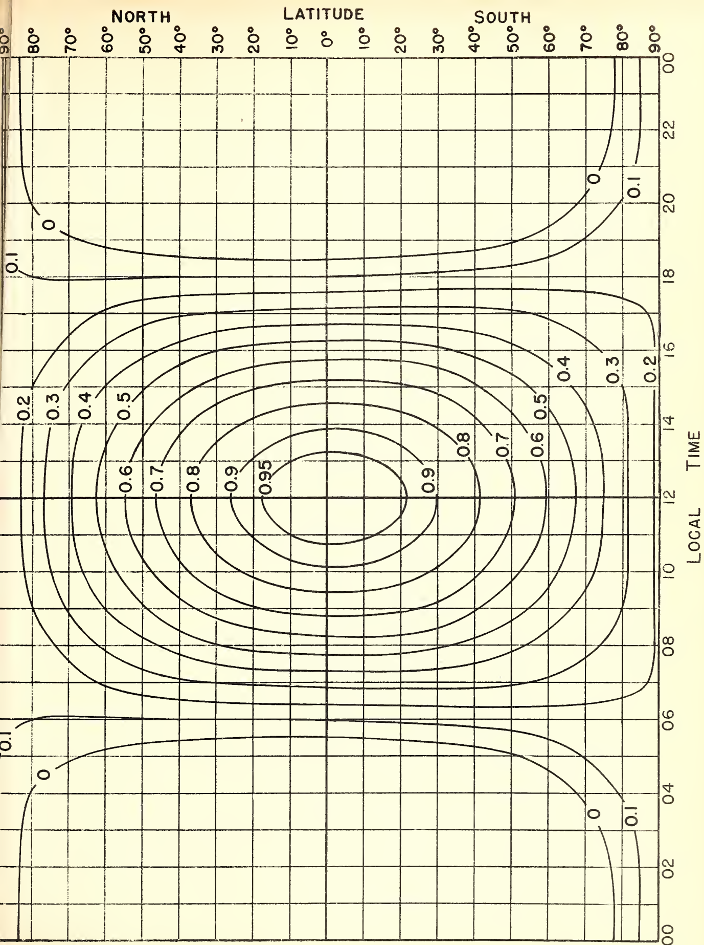
Fig.16 ABSORPTION INDEX CHART (EXCLUDING AURORAL ABSORPTION) FOR MARCH.
