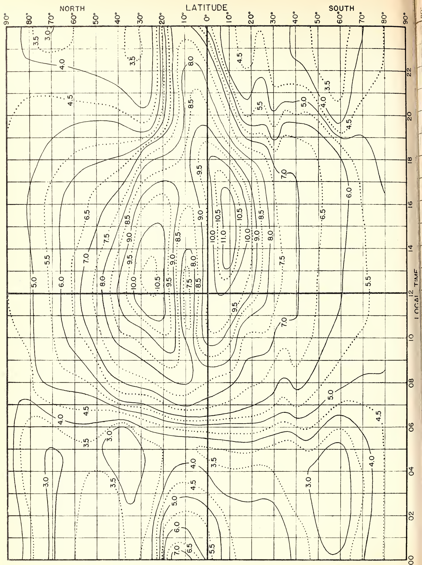
Fig. 9. F 2 ZERO-MUF, IN Mc, E ZONE, PREDICTED FOR MARCH 1945.
