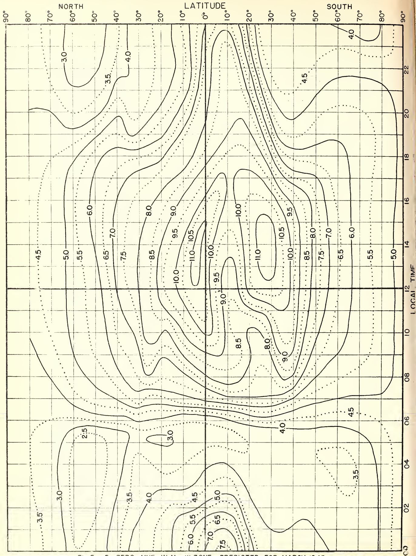
Fig-5. F_2 ZERO-MUF, IN Mc, W ZONE, PREDICTED FOR MARCH 1945
