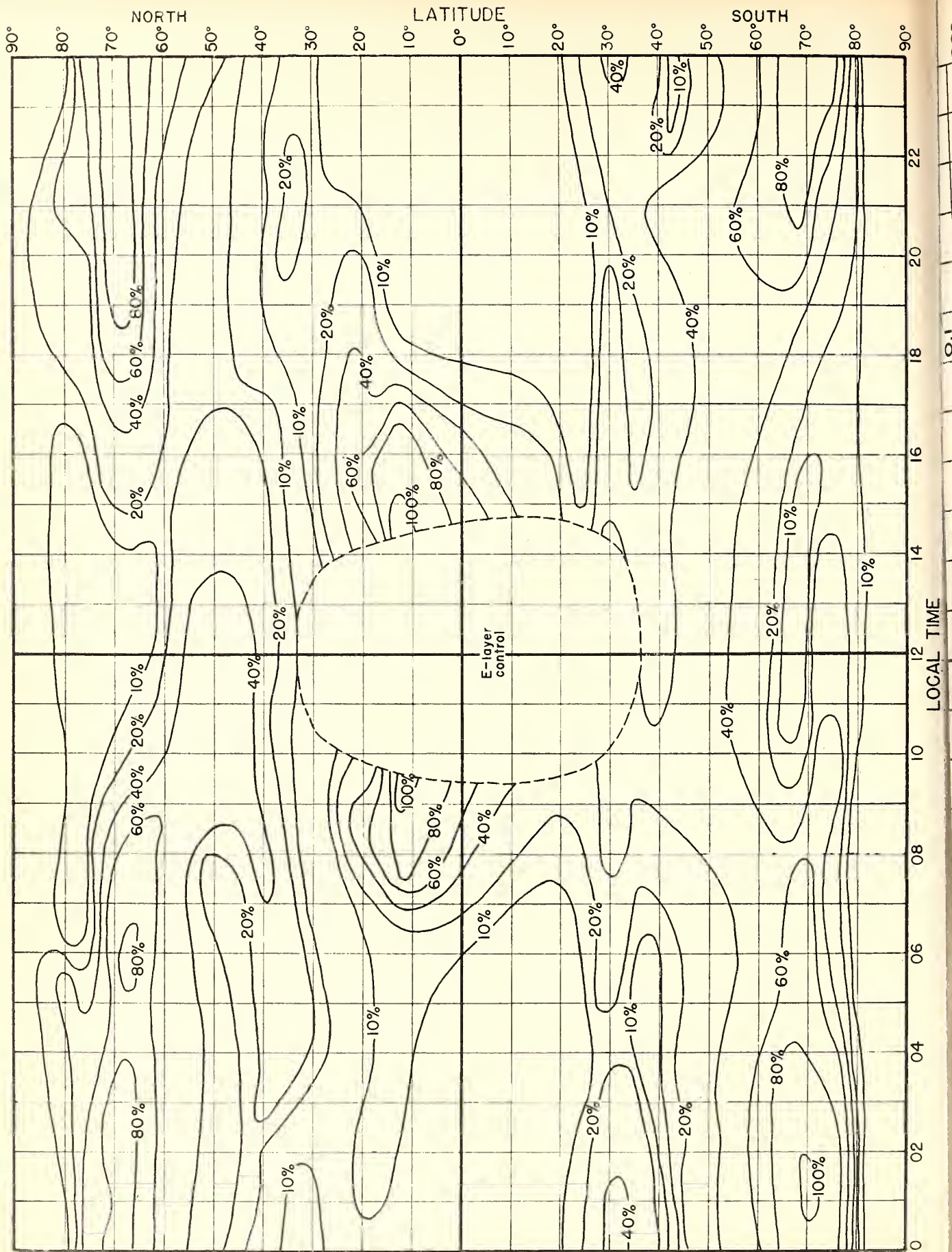
Fig. 15. PERCENTAGE OF TIME OCCURRENCE FOR E_s IN EXCESS OF 15 Mc, PREDICTED FOR MARCH, 1945.
