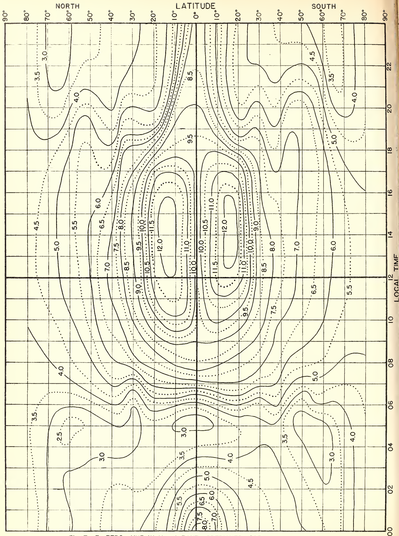
Fig. 7. F_2 ZERO-MUF, IN Mc, I ZONE, PREDICTED FOR MARCH 1945.
