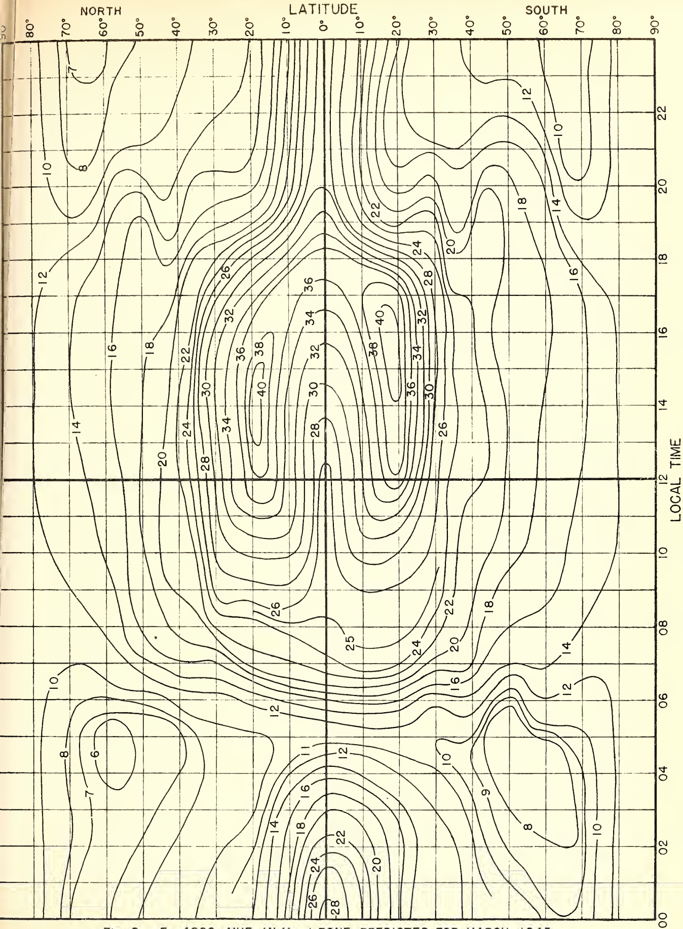
Fig. 8. F_2 4000-MUF, IN Mc, I ZONE, PREDICTED FOR MARCH 1945.
