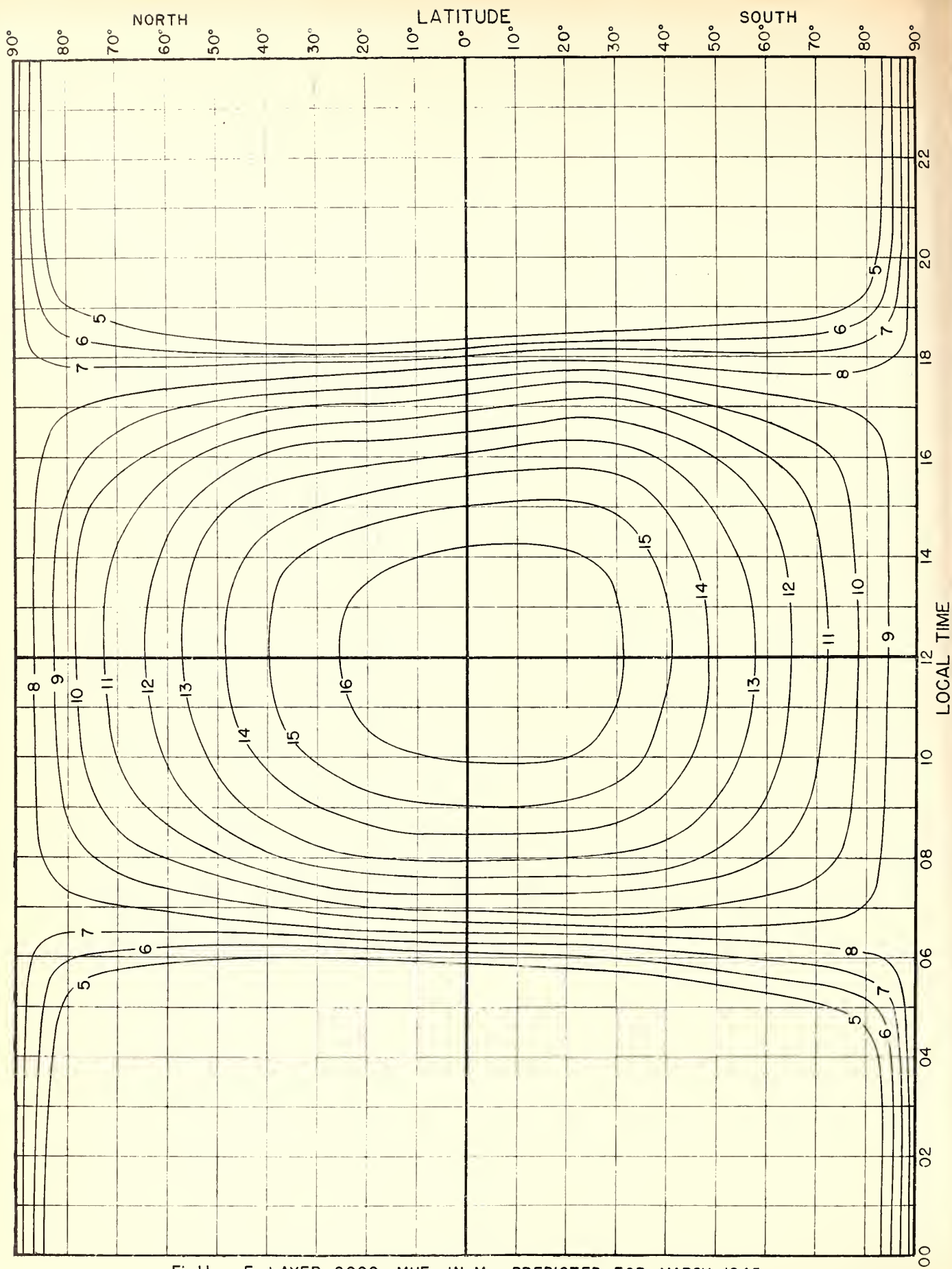
Fig.11. E-LAYER 2000-MUF, IN Mc, PREDICTED FOR MARCH 1945.
