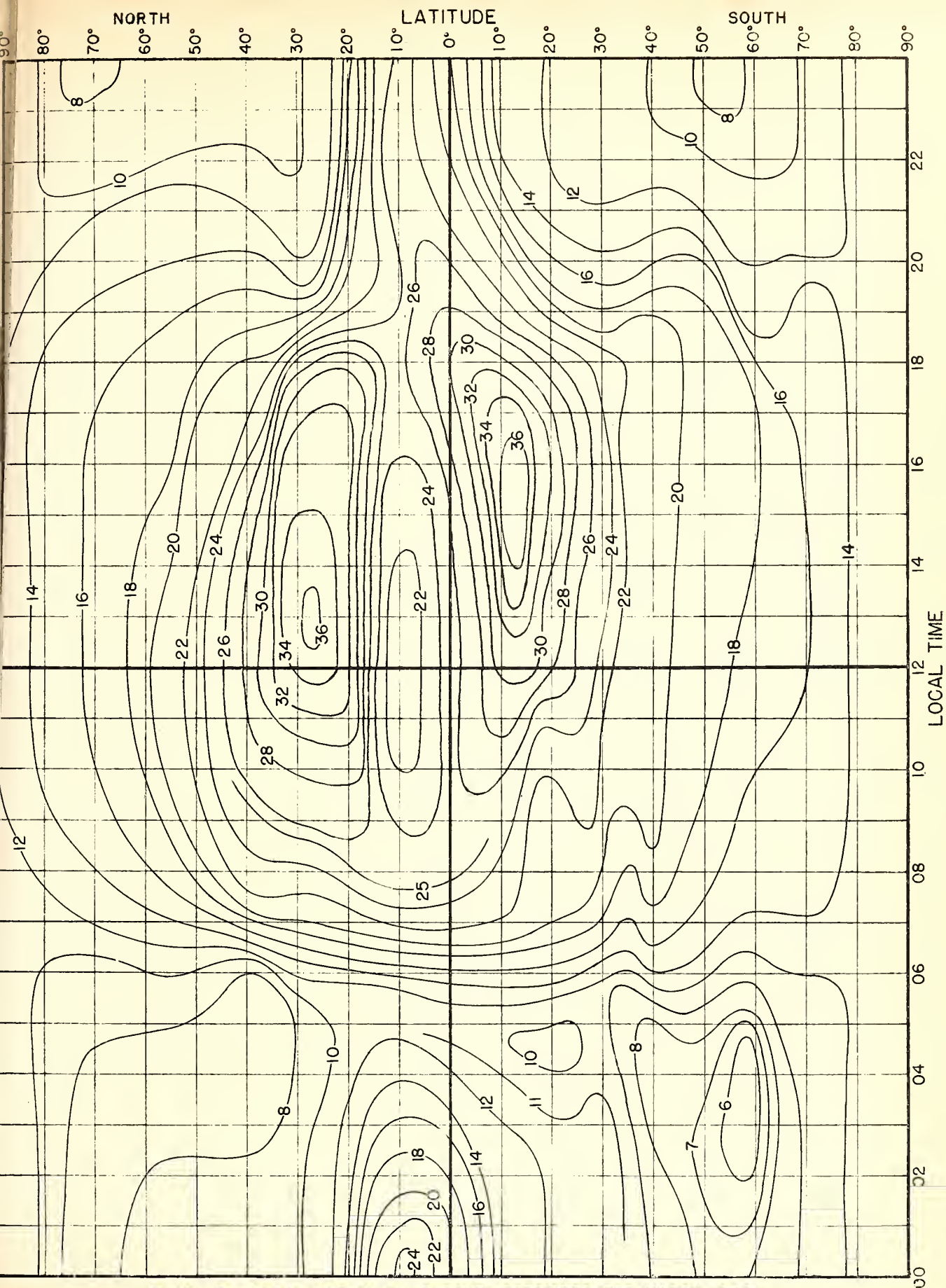
Fig. 10. F_2 4000-MUF, IN Mc, E ZONE, PREDICTED FOR MARCH 1945.
