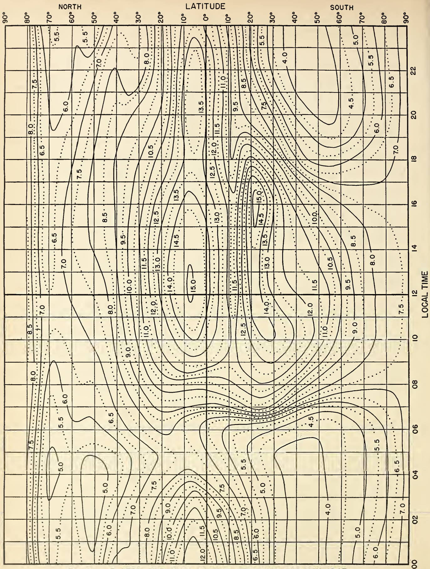
Fig. 5. F 2 ZERO-MUF, IN Mc, W ZONE, PREDICTED FOR MAY 1947
