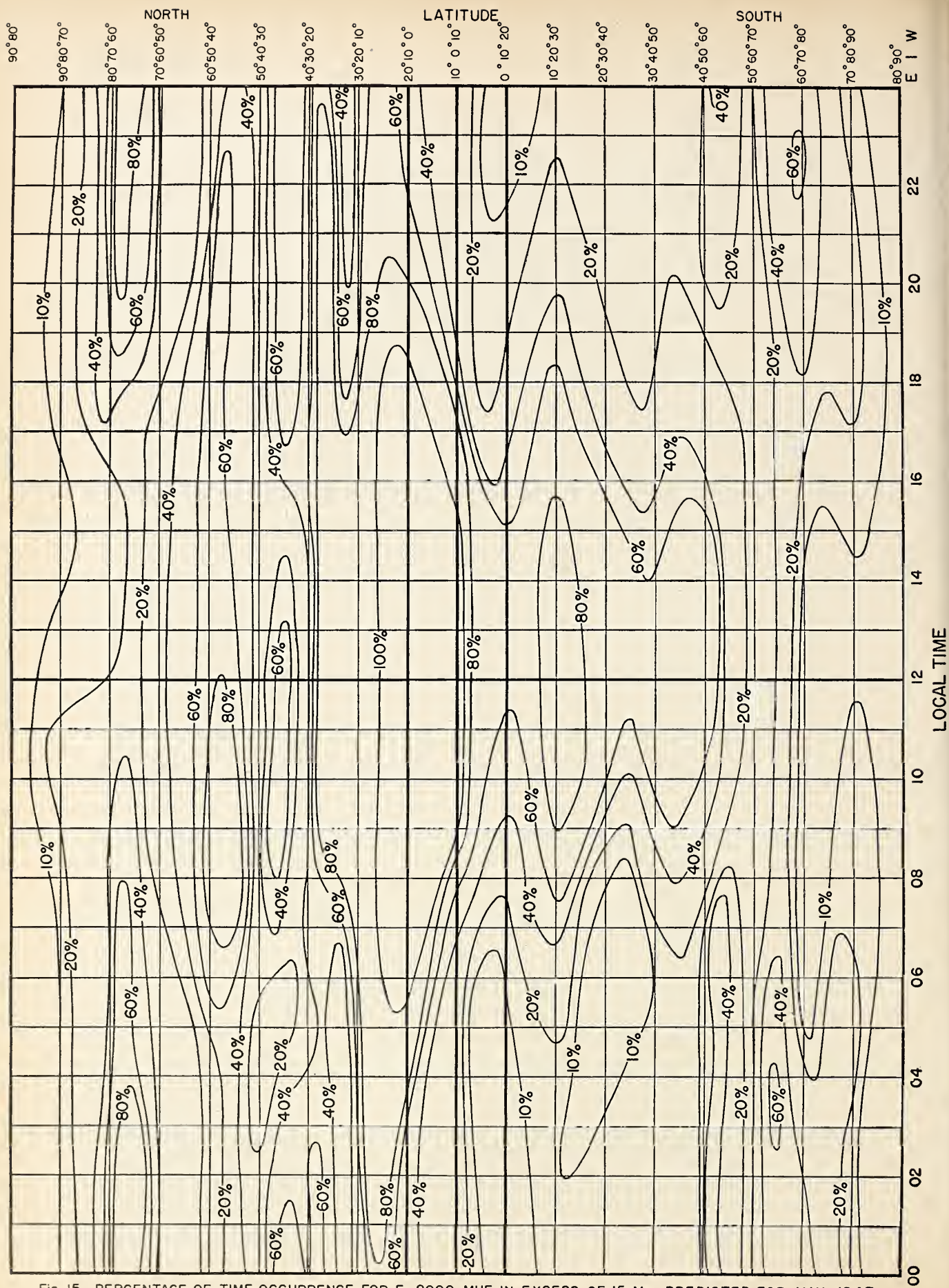
Fig. 15. PERCENTAGE OF TIME OCCURRENCE FOR E_s 2000-MUF IN EXCESS OF 15 Mc, PREDICTED FOR MAY 1947.
