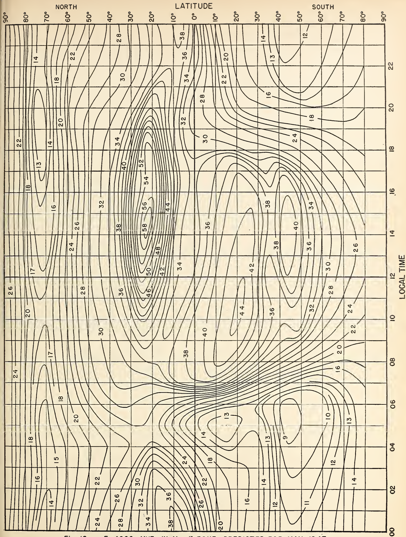
Fig. 10. F 2 4000-MUF, IN Mc, E ZONE, PREDICTED FOR MAY 1947
