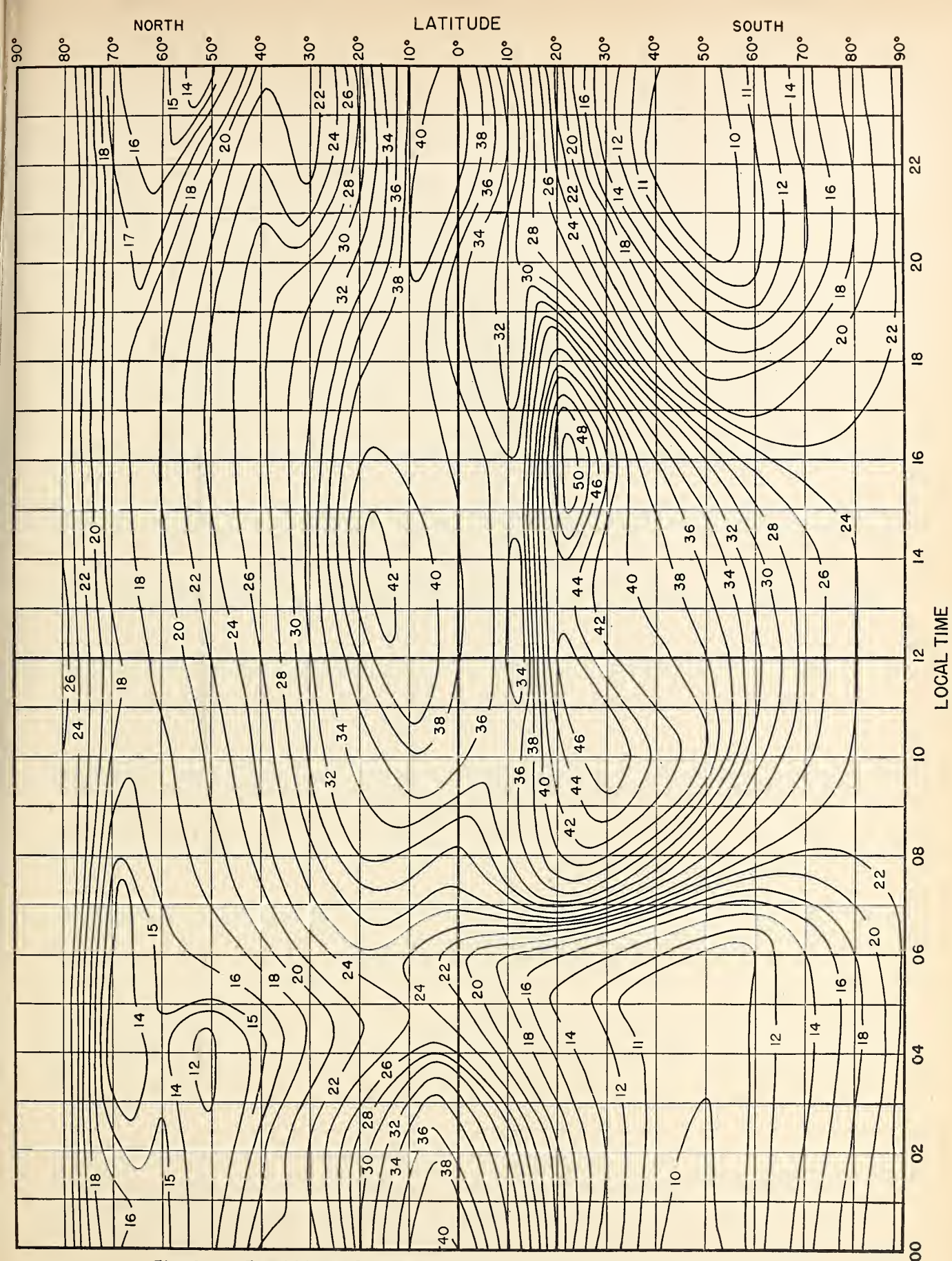
Fig. 6. F 2 4000-MUF, IN Mc, W ZONE, PREDICTED FOR MAY 1947
