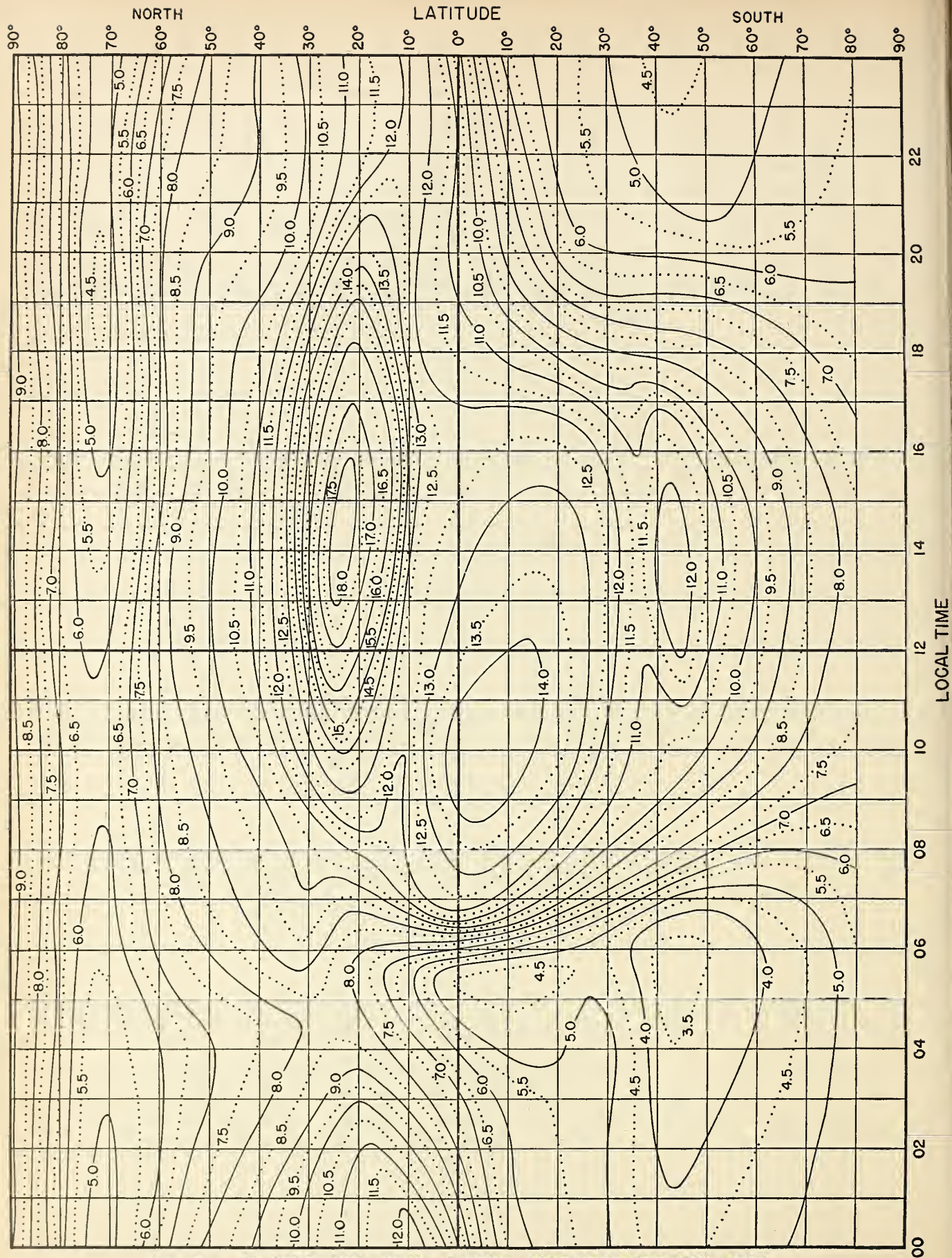
Fig. 9. F 2 ZERO-MUF, IN Mc, E ZONE, PREDICTED FOR MAY 1947
