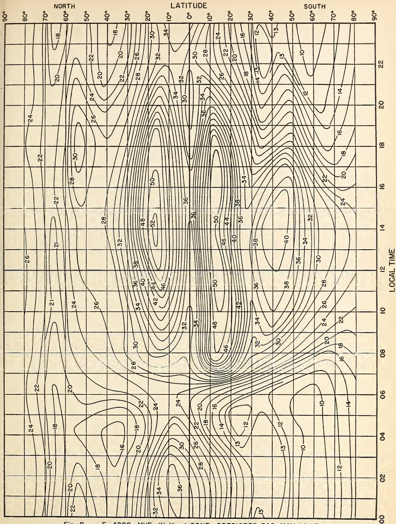
Fig. 8. F_2 4000-MUF, IN Mc, I ZONE, PREDICTED FOR MAY 1947
