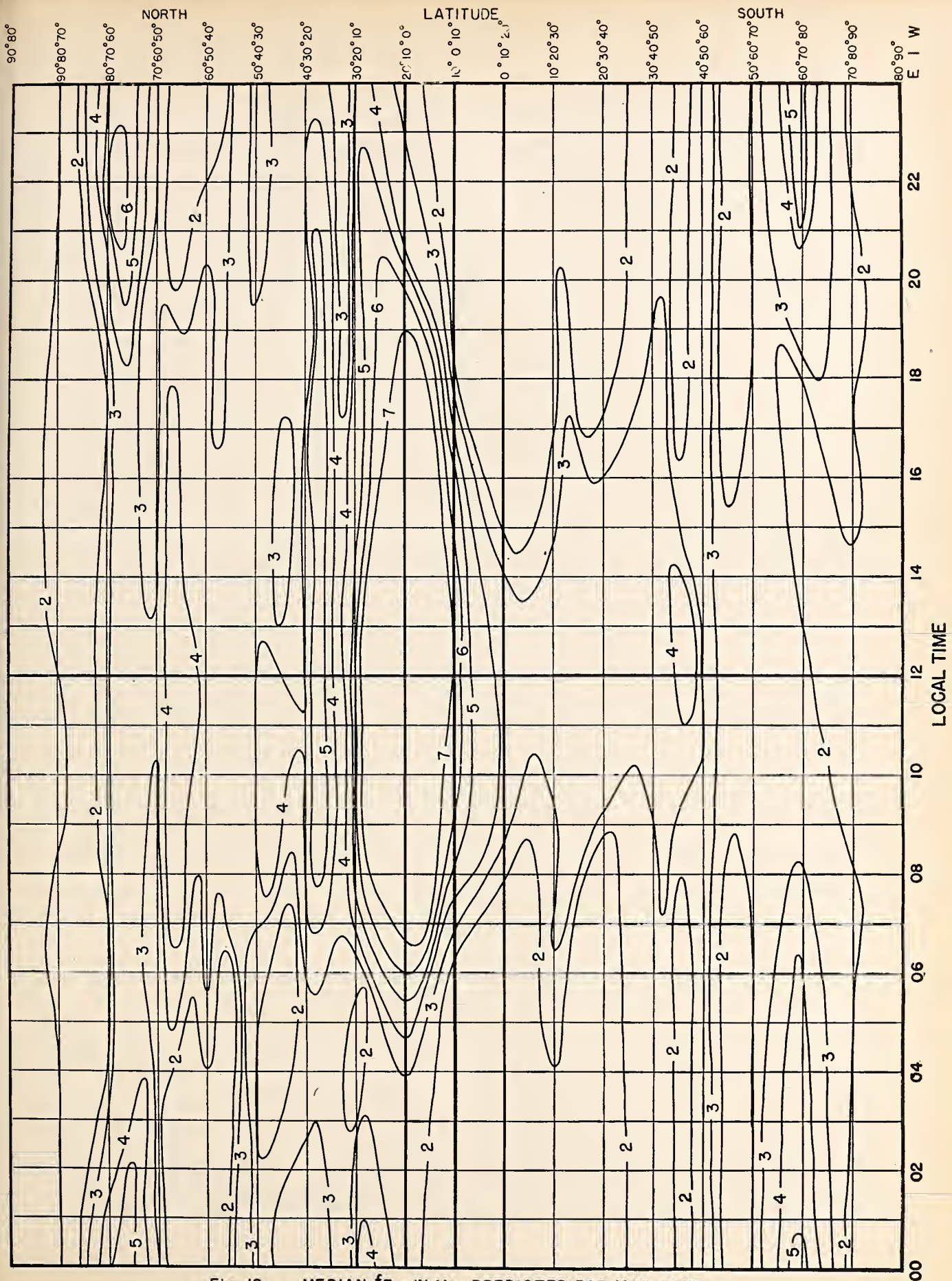
Fig. 12. MEDIAN f_{Es} , IN Mc, PREDICTED FOR MAY 1947
