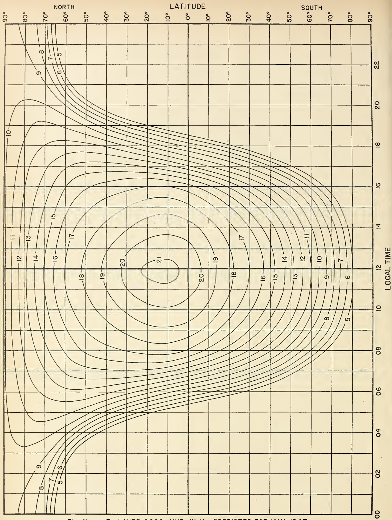
Fig. 11. E-LAYER 2000-MUF, IN Mc, PREDICTED FOR MAY 1947
