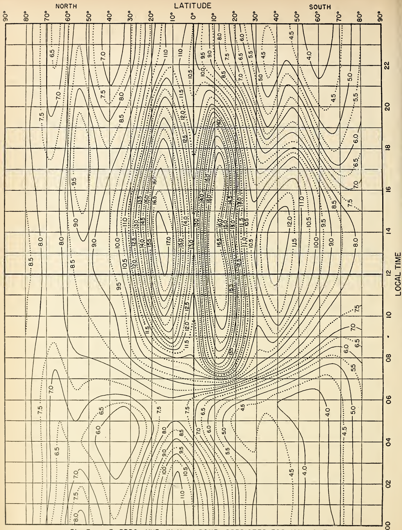
Fig. 7. F 2 ZERO-MUF, IN Mc, I ZONE, PREDICTED FOR MAY 1947
