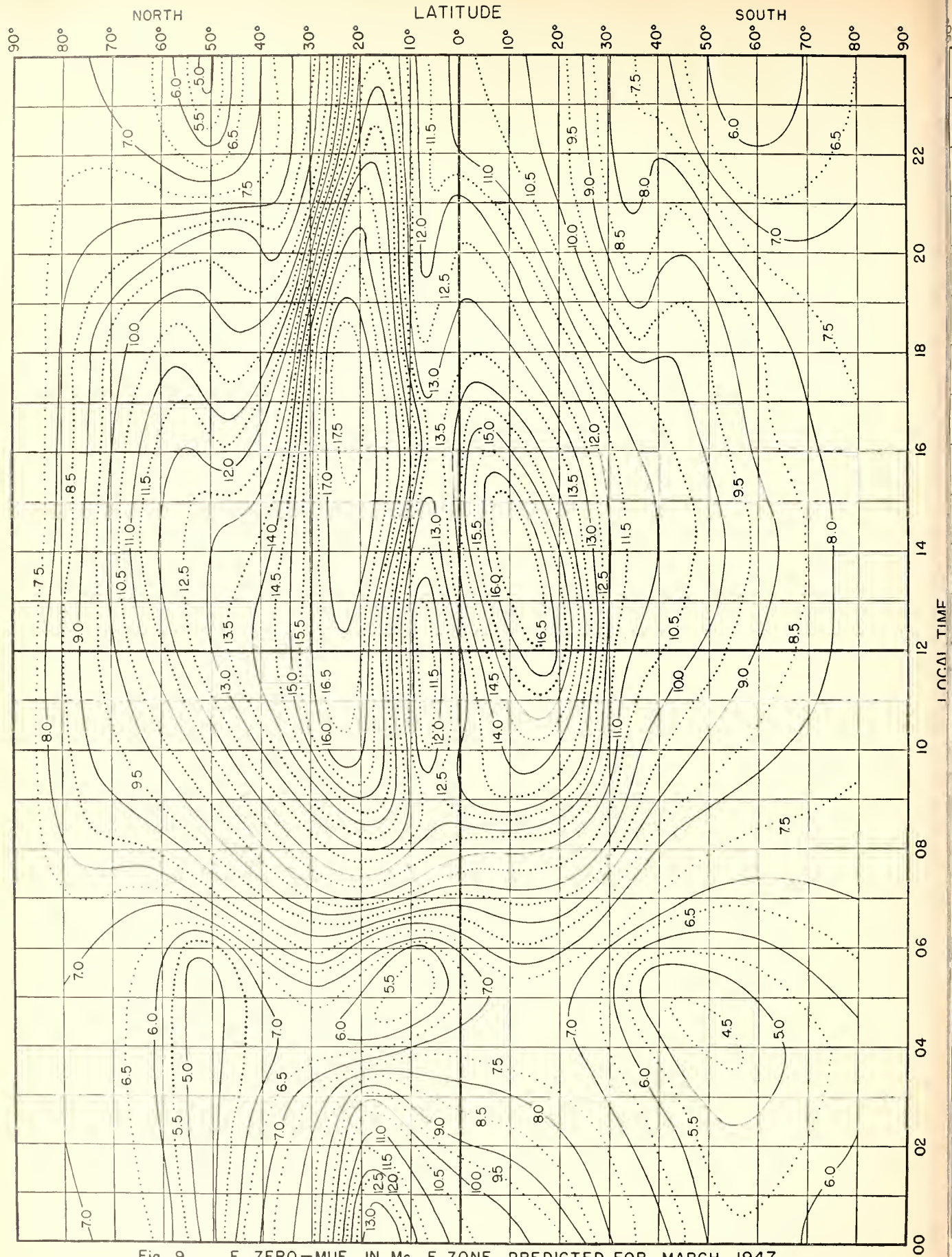
Fig. 9. F_2 ZERO-MUF, IN Mc, E ZONE, PREDICTED FOR MARCH 1947
