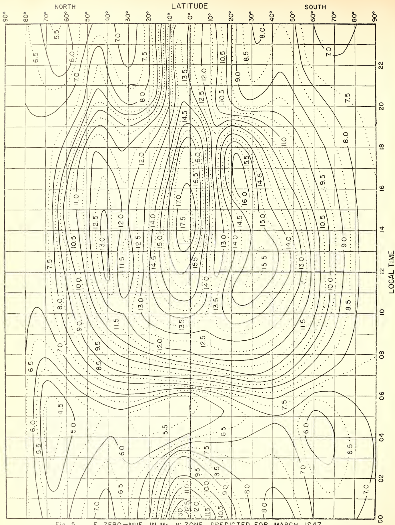
Fig. 5. F 2 ZERO-MUF, IN Mc, W ZONE, PREDICTED FOR MARCH 1947
