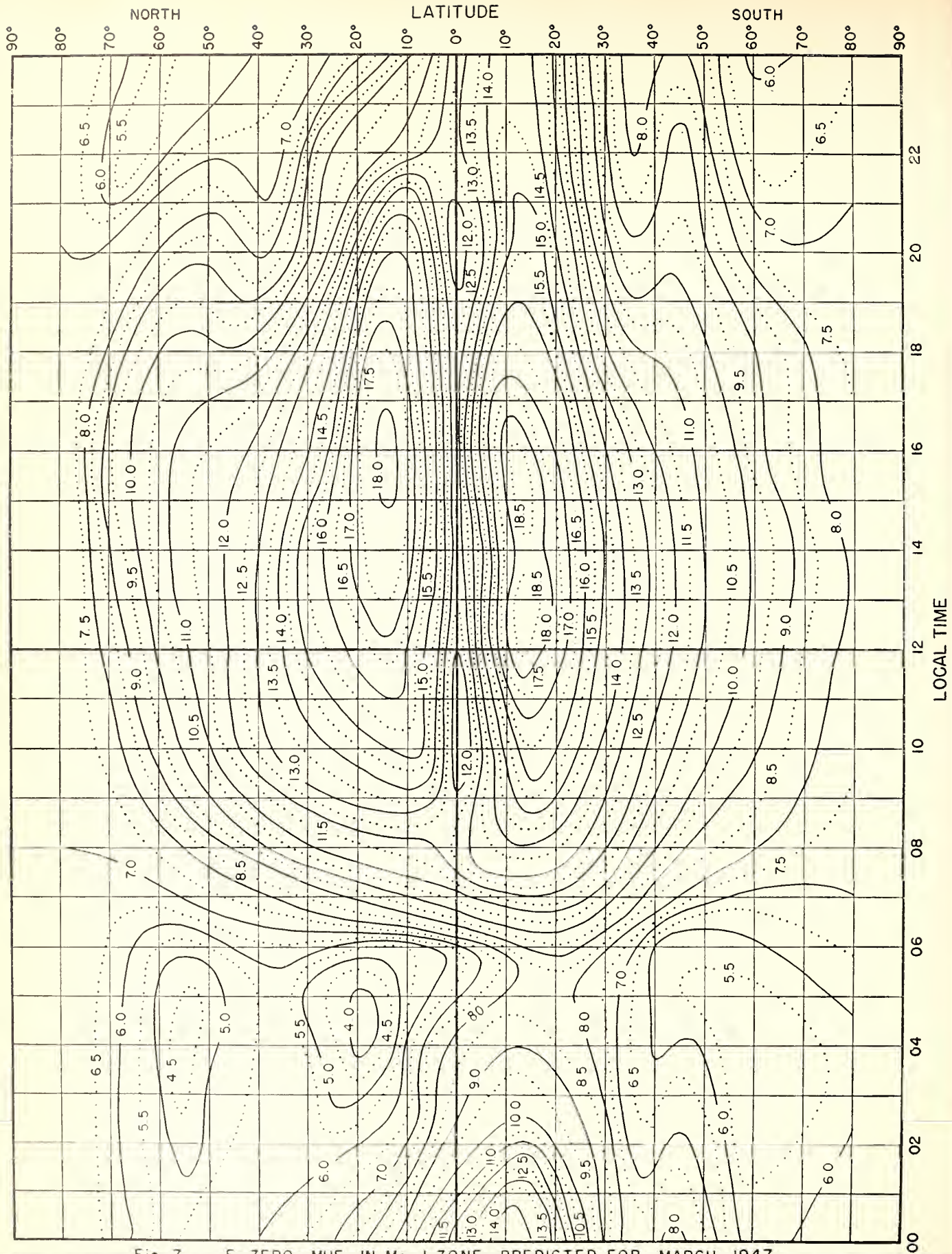
Fig. 7. F_2 ZERO-MUF, IN Mc, I ZONE, PREDICTED FOR MARCH 1947
