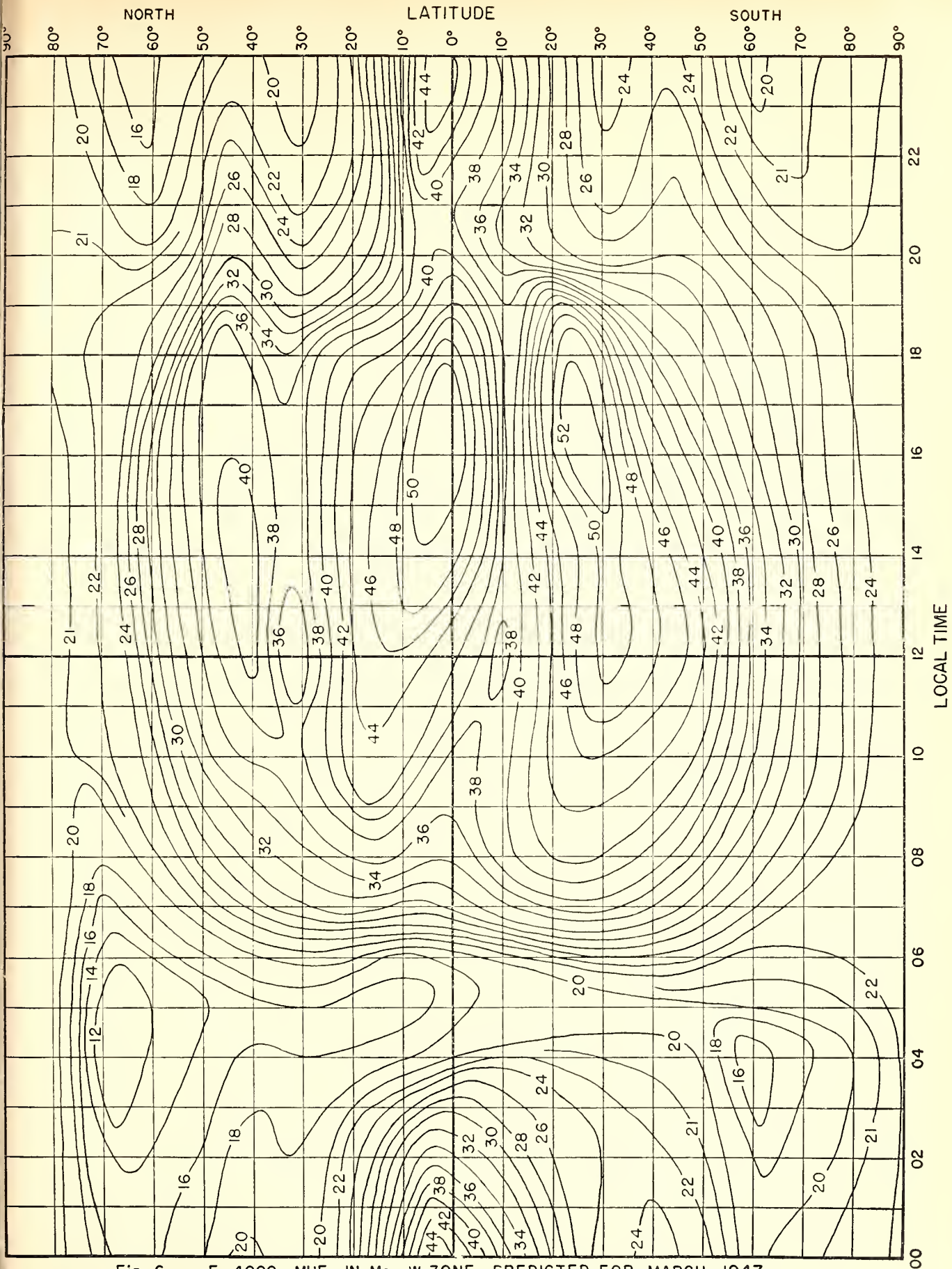
Fig. 6. F 2 4000-MUF, IN Mc, W ZONE, PREDICTED FOR MARCH 1947
