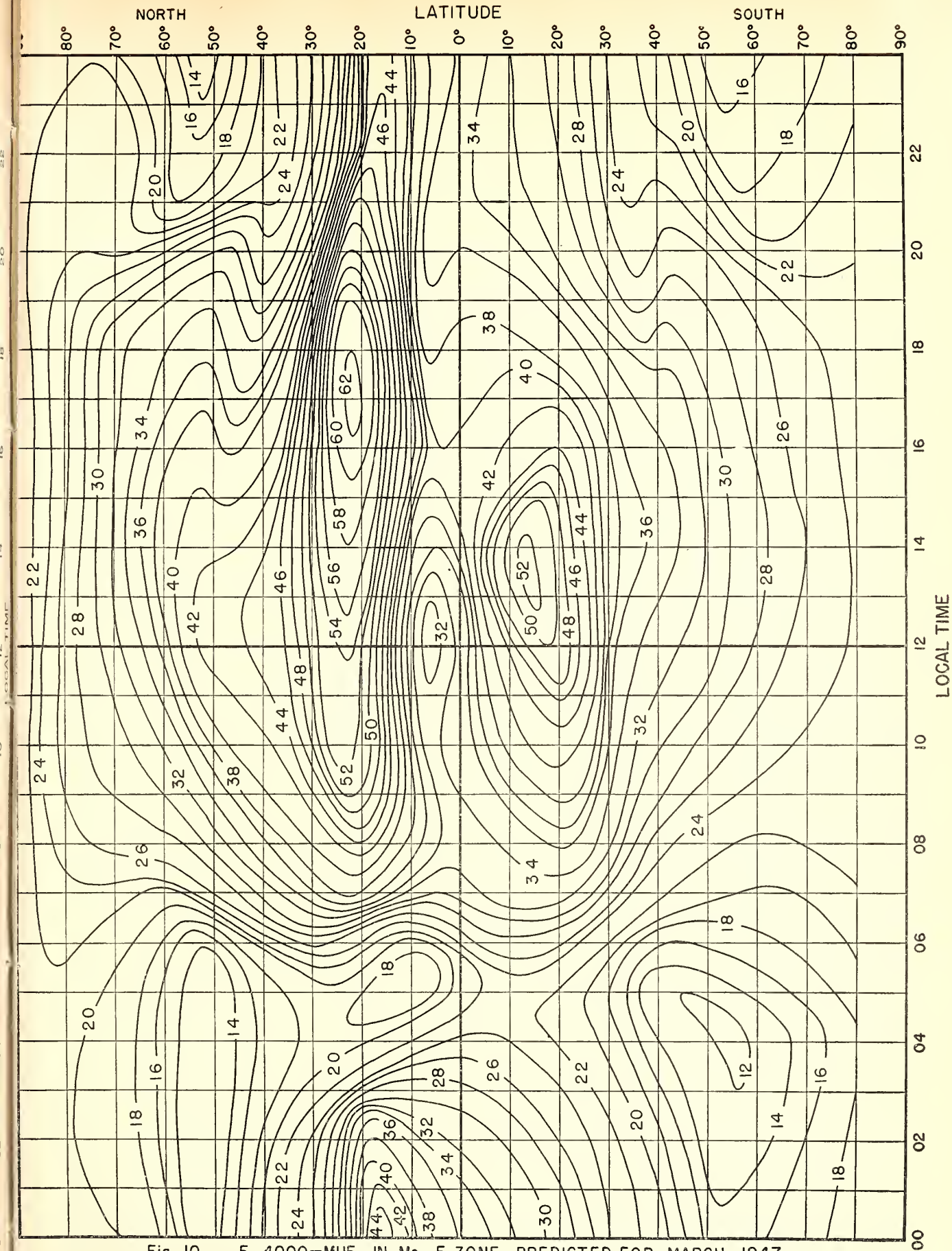
Fig. 10. F_2 4000-MUF, IN Mc, E ZONE, PREDICTED FOR MARCH 1947
