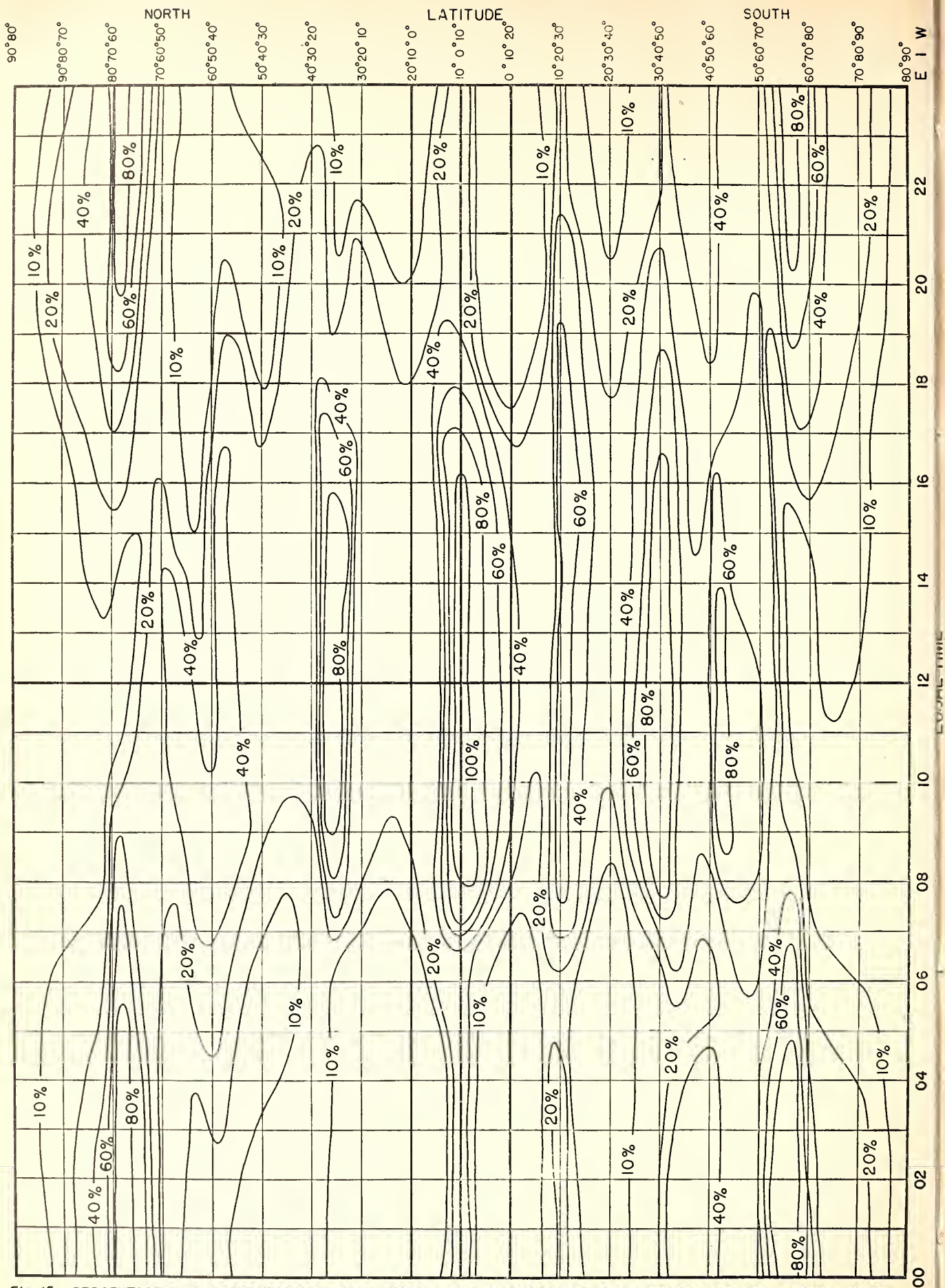
Fig. 15. PERCENTAGE OF TIME OCCURRENCE FOR E_s 2000 - MUF IN EXCESS OF 15 Mc PREDICTED FOR MARCH 1947.
