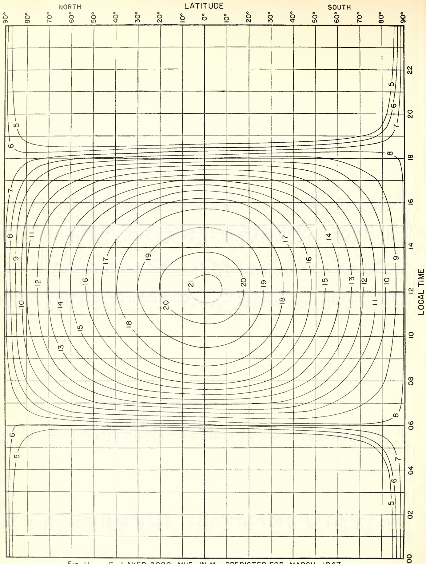
Fig. II. E-LAYER 2000-MUF, IN Mc, PREDICTED FOR MARCH 1947
