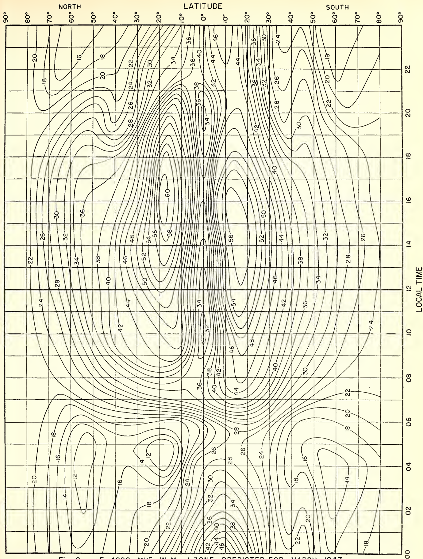
Fig. 8. F 2 4000-MUF, IN Mc, I ZONE, PREDICTED FOR MARCH 1947
