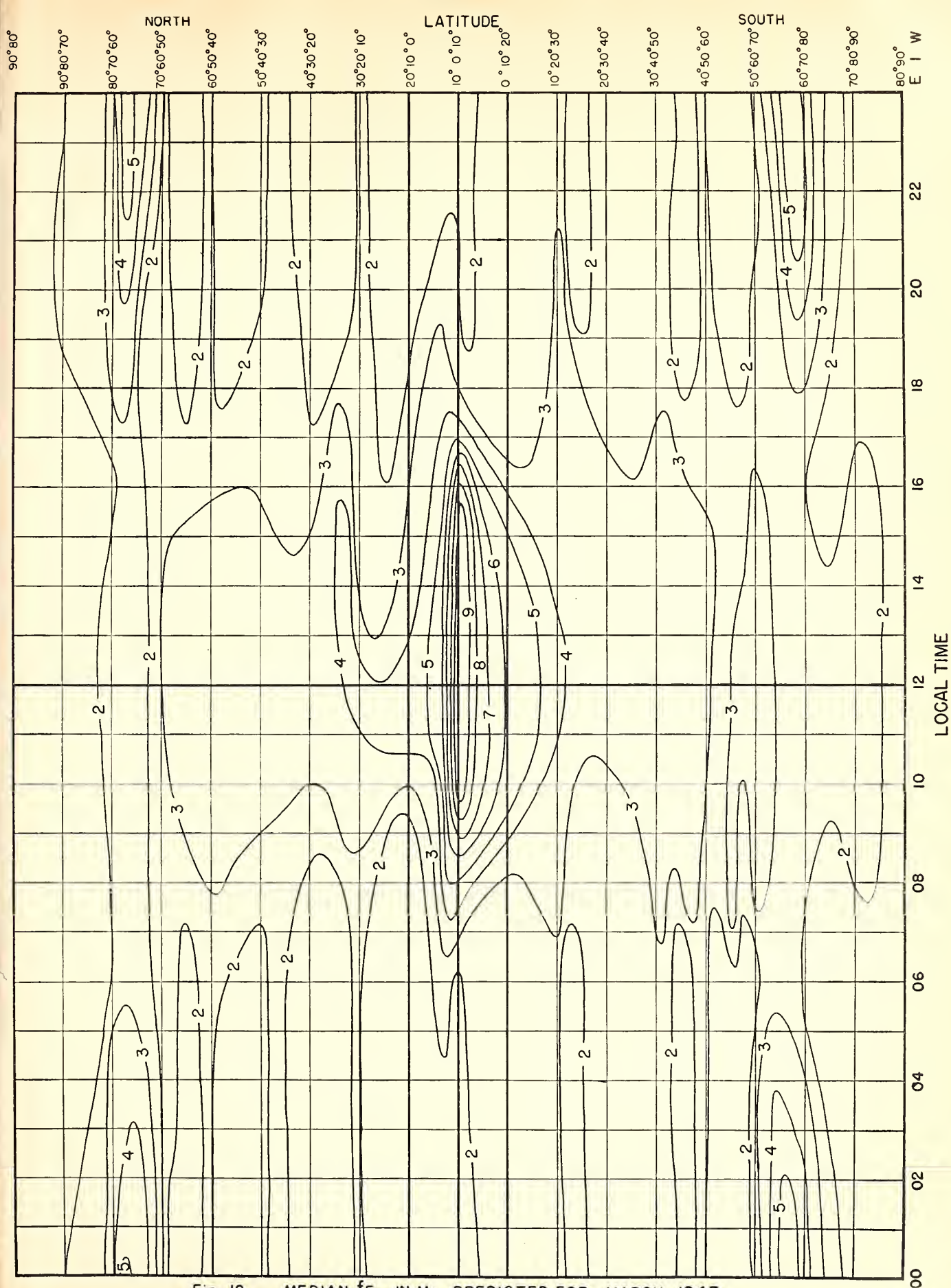
Fig. 12. MEDIAN f_{Es} , IN Mc, PREDICTED FOR MARCH 1947.
