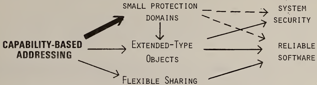
Figure 8 - Capability-Based Addressing
