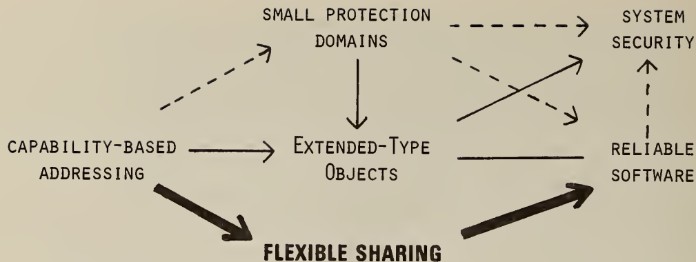
Figure 13 - Flexible Sharing
