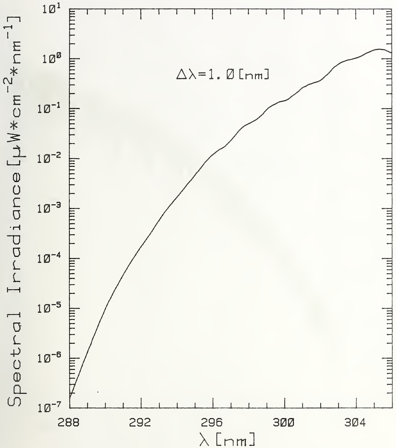
Figure 2. Calculated solar terrestrial spectral irradiance (triangular slit-scattering function with a 1 [nm] spectral slit width).
