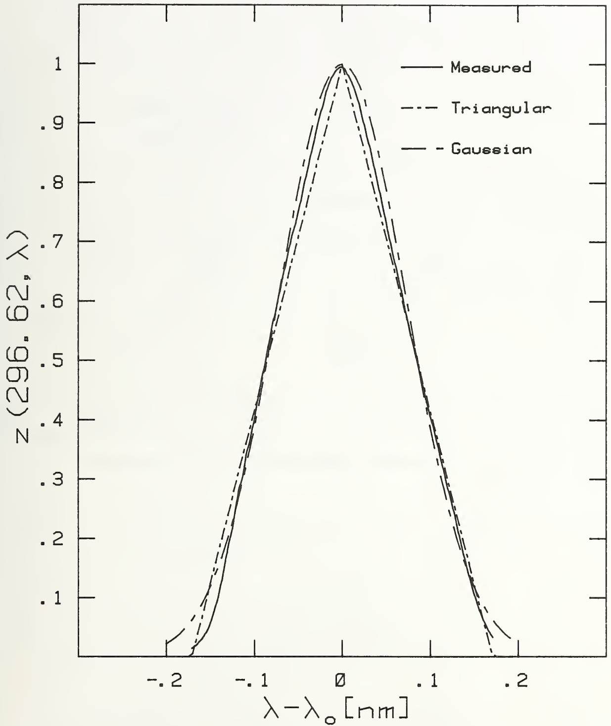
Figure 14. Measured slit-scattering function z(\lambda_0, \lambda) at \lambda_0 = 296.62 [nm] and triangular and Gaussian functions having the same spectral width.
