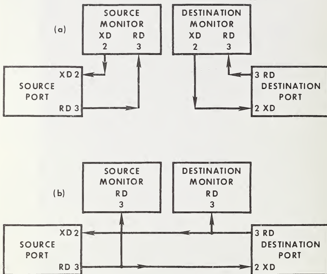
Figure 11. Connection States of the Network Measurement Machine
