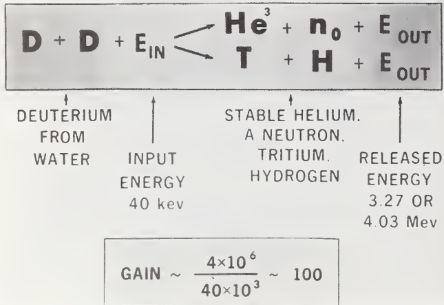
Figure 9. The D-D Fusion Fuel Reactions
