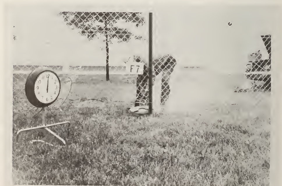
Figure 210. Cutting Metric Intermediate Post near Ground with Abrasive Wheel Saw; Test F7
