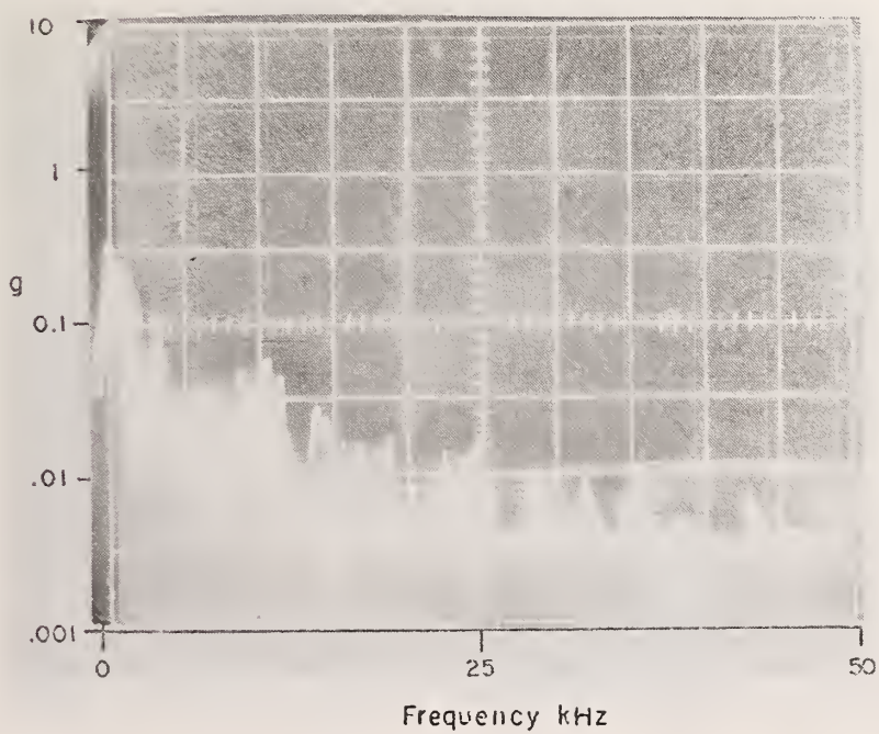
Figure 78. Vibrational Disturbances Produced by Saw; Test 9N
