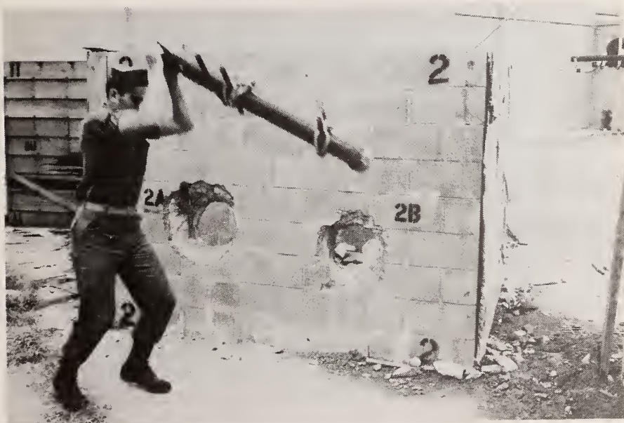
Figure 41. Test 5K. Single Man Using Suspended Battering Ram, Raising Center of Gravity 24"
