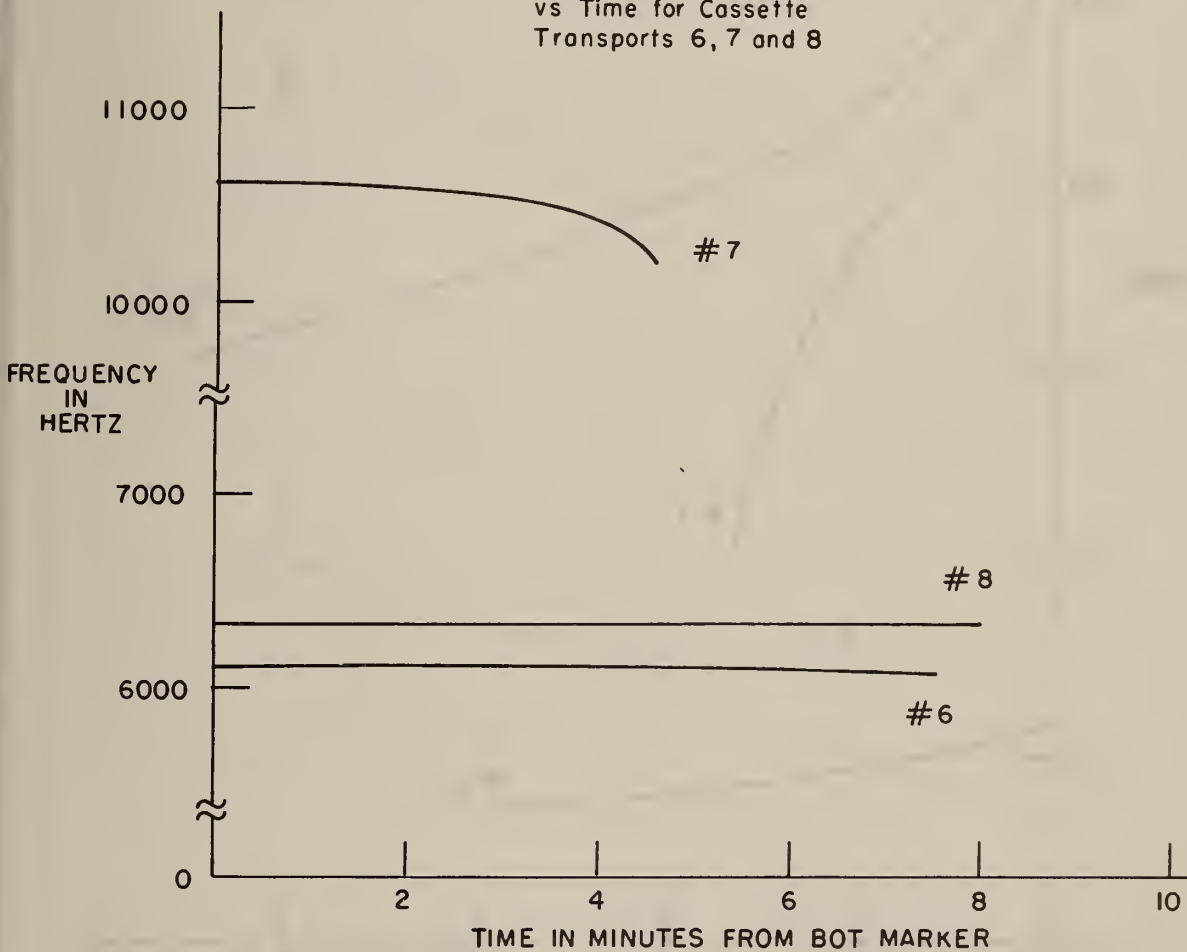
Figure 9. Cassette transport speed measurement curves
