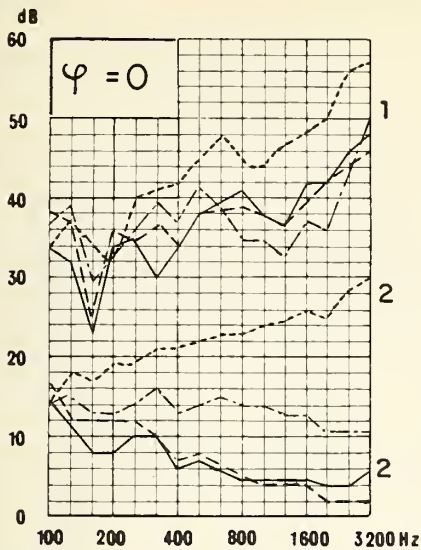
Figure 13. Normalized Sound insulation: Loggia with absorbent lining.
