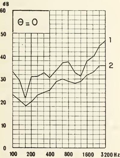
Figure 6. Normalized sound insulation for 'bare facades'.
