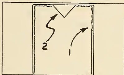
Figure 25. The dummy aperture holder. 1 - black coating on interior of dummy aperture holder (also on interior of aperture holder), 2 - 45° half-angle polished aluminum core to simulate the effect of the hole on emitted flux.
