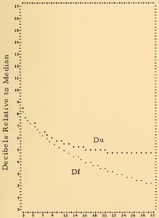
Figure 16. Frequency Dependence of Median and Deciles of Radio Noise March-April-May (0000-0400 Local Mean Time)
