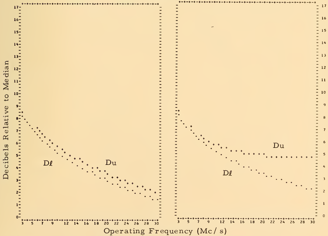
Figure 40. Frequency Dependence of Median and Deciles of Radio Noise September-October-November (0000-0400 Local Mean Time)
