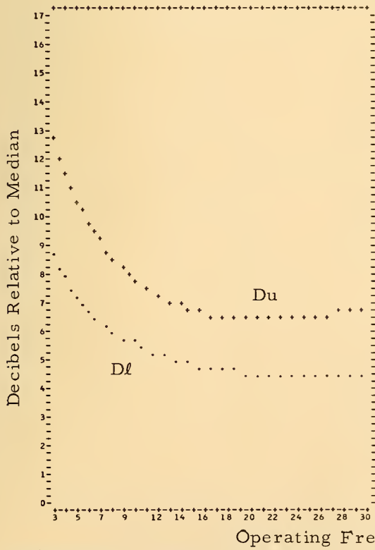
Figure 32. Frequency Dependence of Median and Deciles of Radio Noise June-July-August (0800-1200 Local Mean Time)
