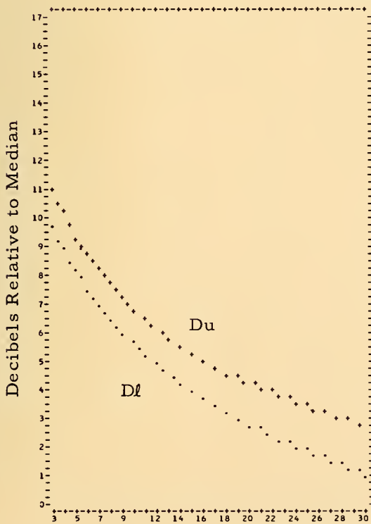
Figure 6. Frequency Dependence of Median and Deciles of Radio Noise December-January-February (0400-0800 Local Mean Time)
