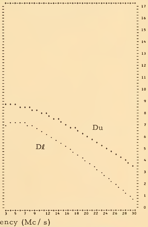
Figure 32. Frequency Dependence of Median and Deciles of Radio Noise June-July-August (0800-1200 Local Mean Time)
