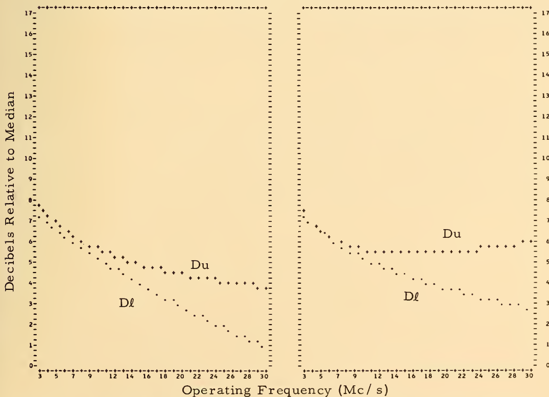
Figure 50. Frequency Dependence of Median and Deciles of Radio Noise September-October-November (2000-2400 Local Mean Time)
