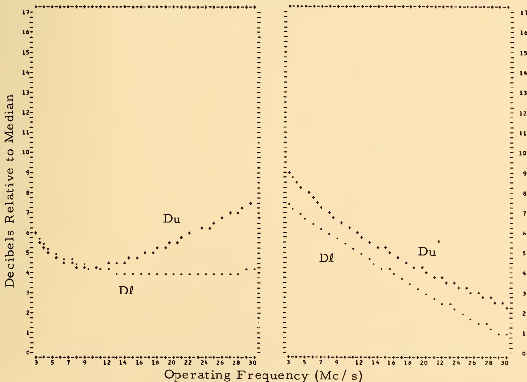
Figure 38. Frequency Dependence of Median and Deciles of Radio Noise June-July-August (2000-2400 Local Mean Time)
