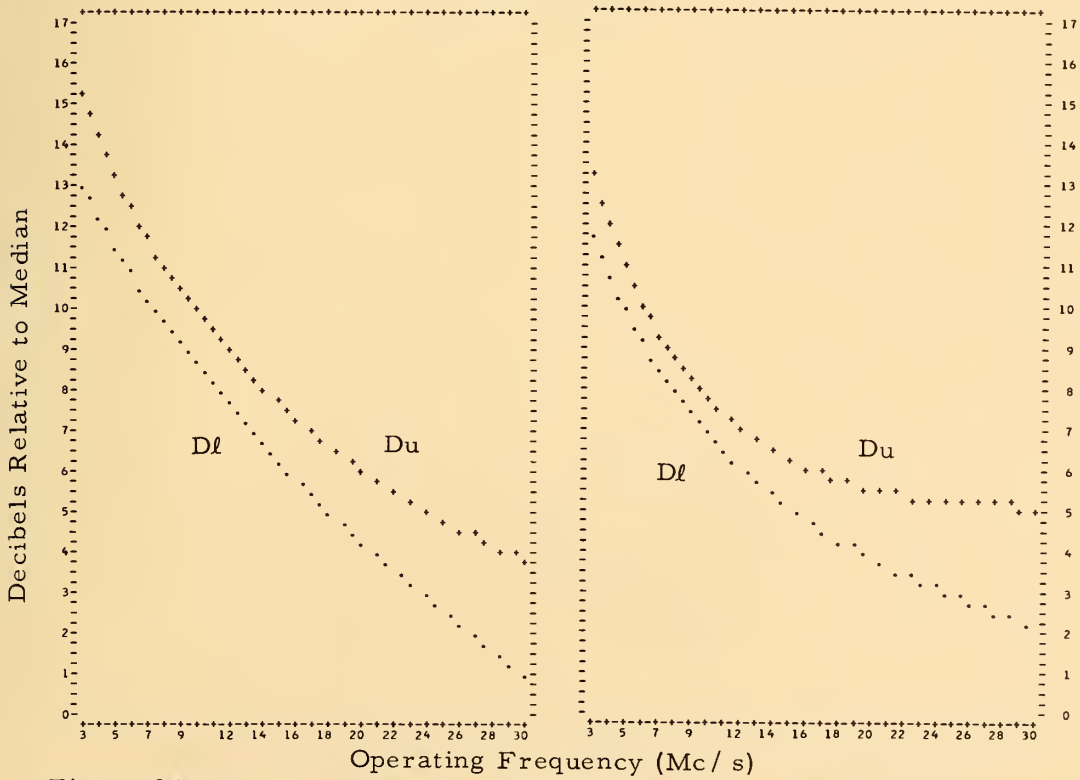
Figure 24. Frequency Dependence of Median and Deciles of Radio Noise March-April-May (1600-2000 Local Mean Time)
