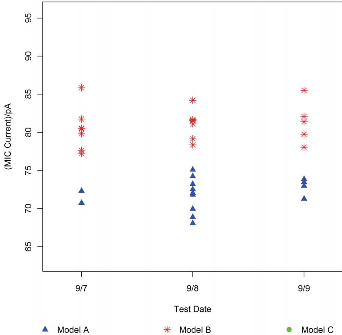
FIGURE C.2: SET 2 SMOKE ALARM RESPONSES VS. TEST DATE
